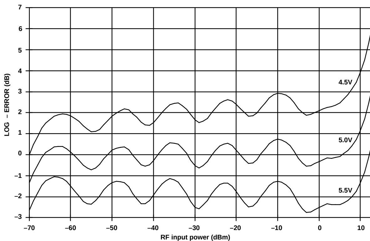
Fig. 14 Video log error, (referenced to single straight line measured at 325MHz, 25°C, 5.0V PSUs), across supply voltage
