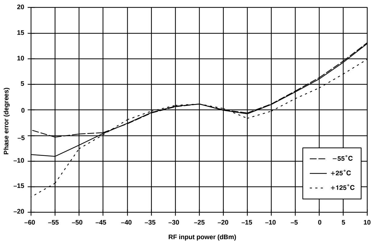
Fig. 22 Limiting phase (500MHz) normalised at -30dBm
