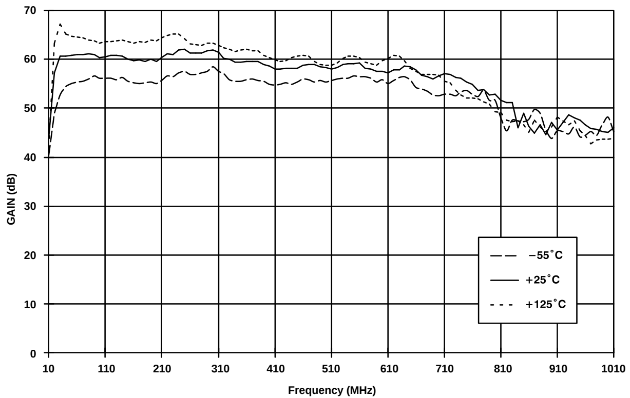
Fig. 16 Linear gain ( -70\text{dBm I/P} )
