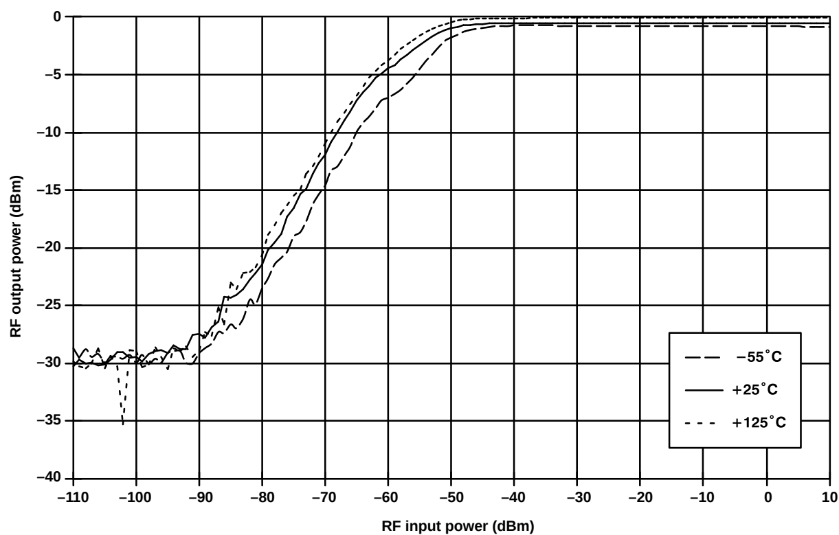
Fig. 19 RF input → output limiting transfer characteristic at Frequency = 500MHz
