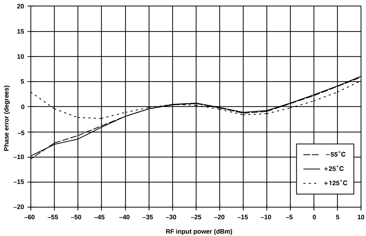
Fig. 21 Limiting phase (300MHz) normalised at -30dBm
