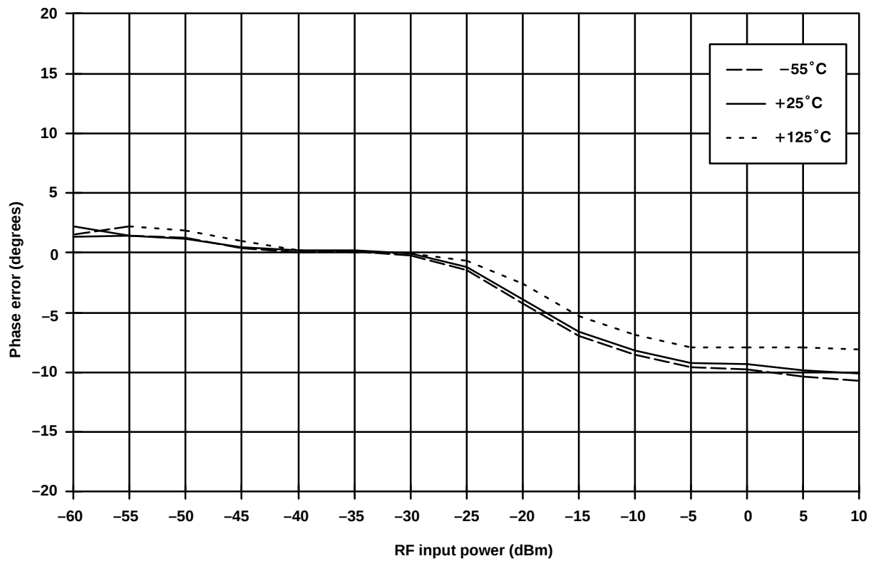
Fig. 20 Limiting phase (100MHz) normalised at -30dBm
