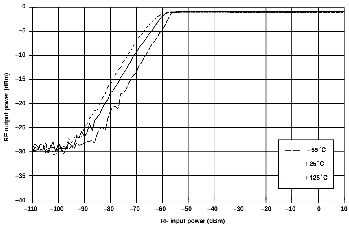
Fig. 17 RF input \rightarrow output limiting transfer characteristic at Frequency = 100MHz
