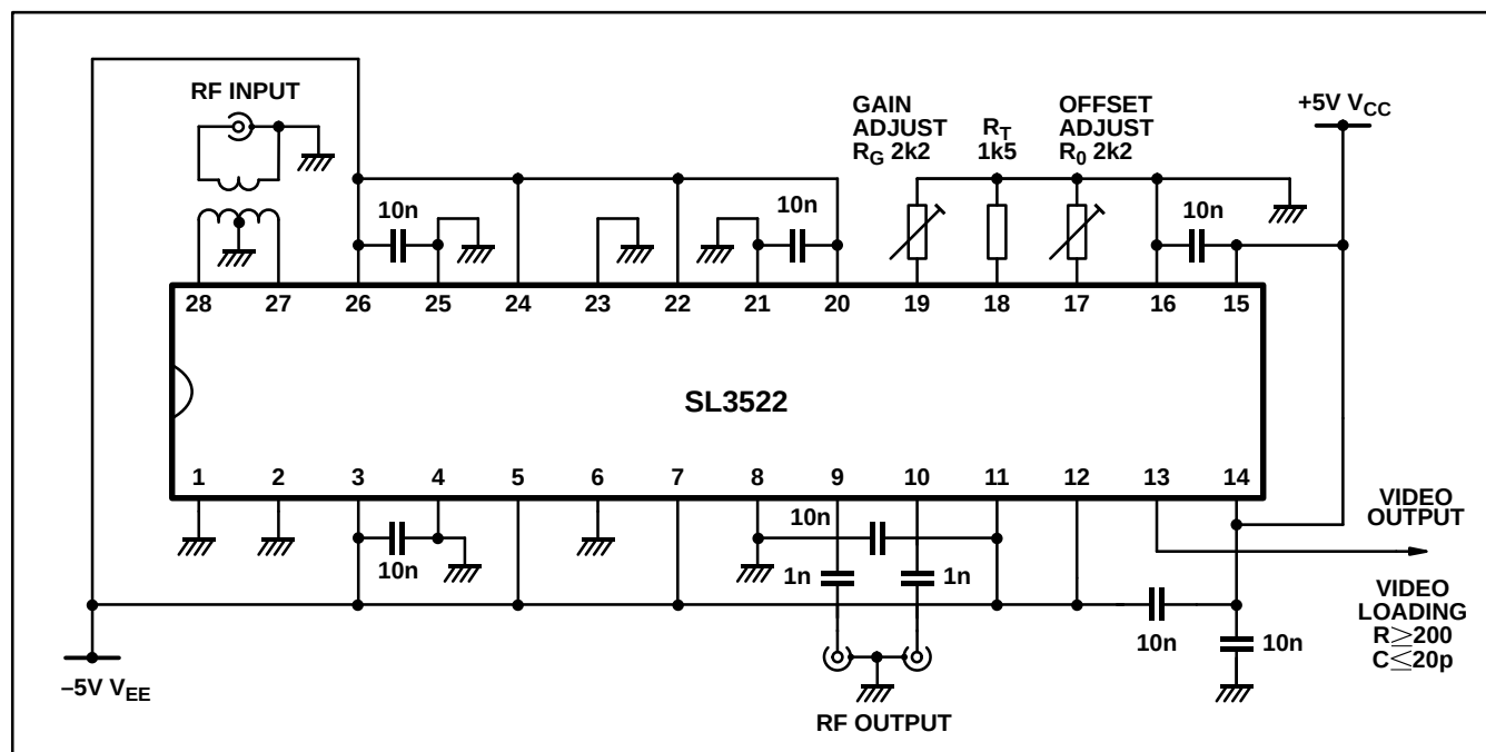
Fig. 6 Applications circuit – Log / Limiting function
