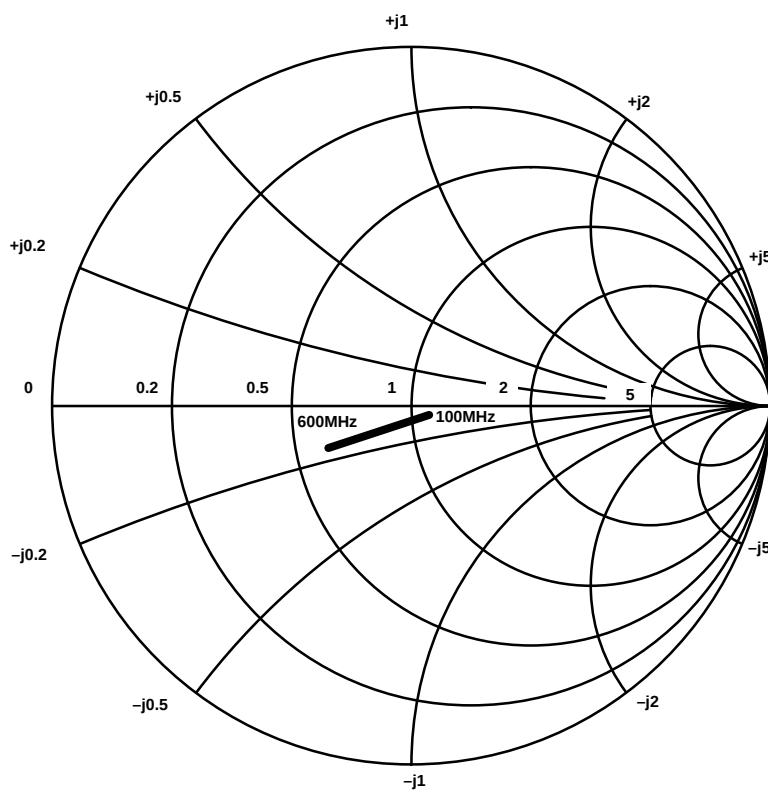
Fig. 23 Typical input impedance normalised to 50Ω – 20dBm I/P level
