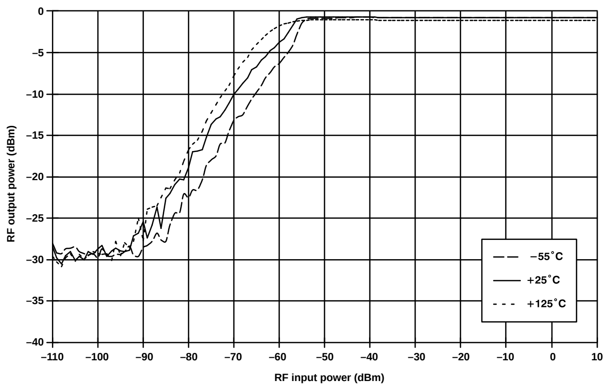
Fig. 18 RF input → output limiting transfer characteristic at Frequency = 325MHz
