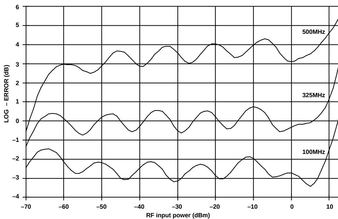
Fig. 15 Video log error, (referenced to single straight line measured at 325MHz, 25°C, 5.0V PSUs), across frequency
