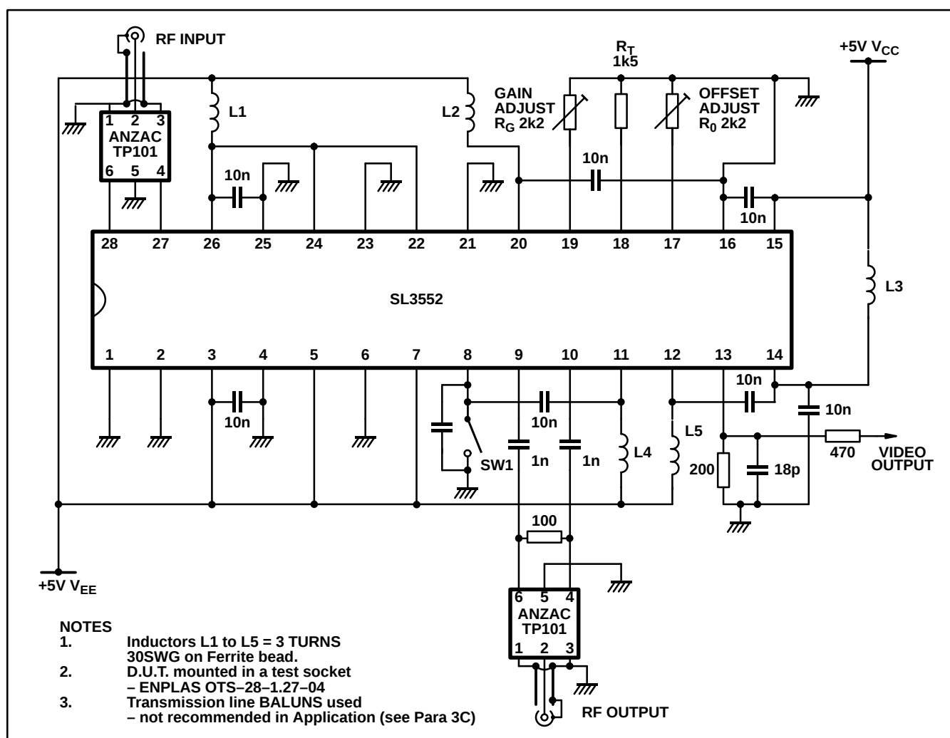
Fig. 3 Test circuit
