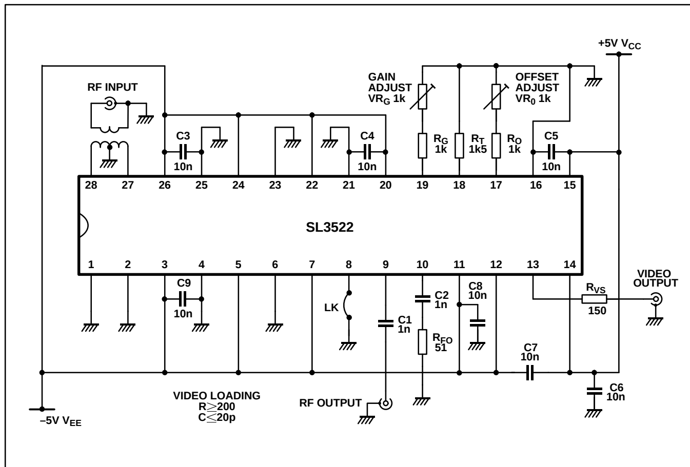
Fig. 10 SL3522 demonstration board circuit diagram
