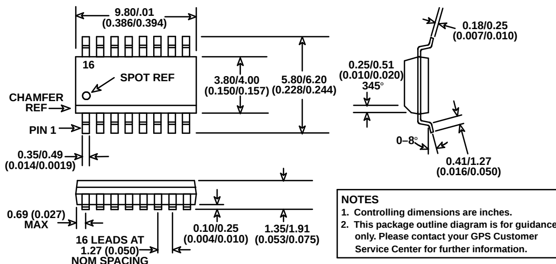
MINIATURE PLASTIC DIL – MP16
