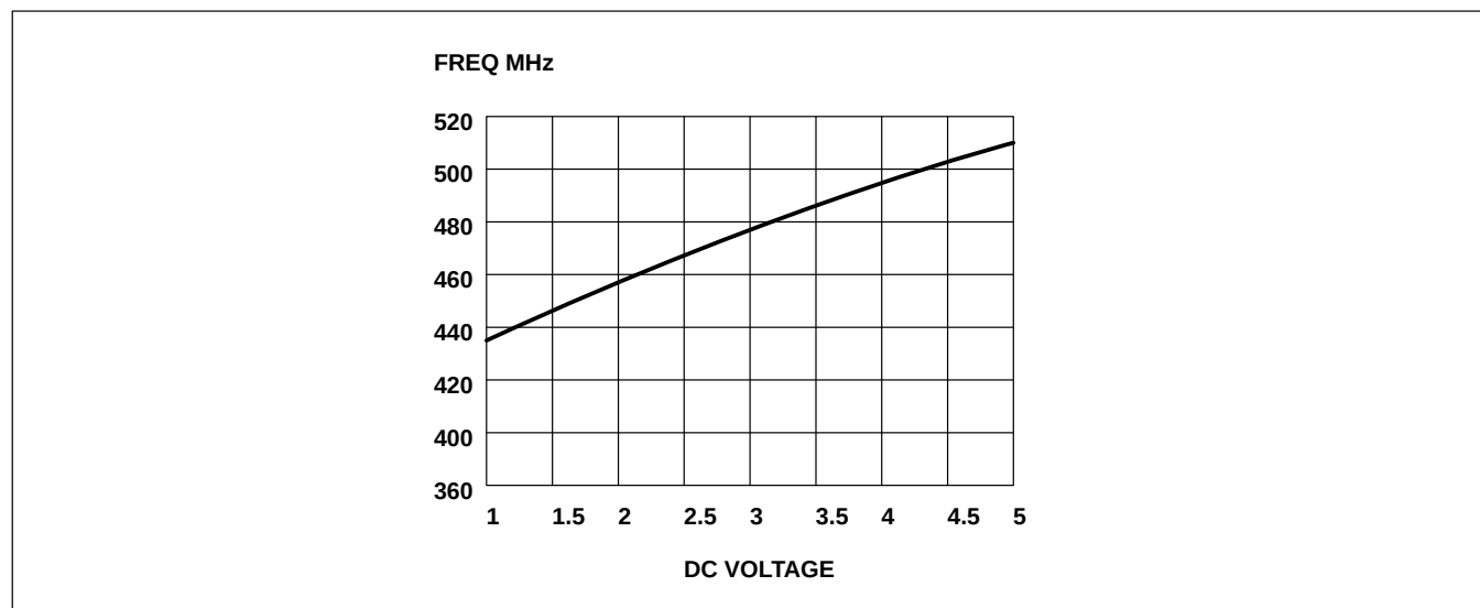
Fig. 7 Typical VCO frequency vs DC control voltage
