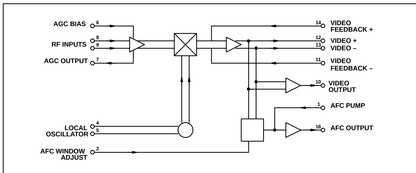
Fig. 2 SL1461SA block diagram
