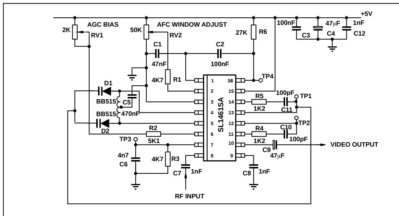
Fig.3. Standard application circuit
