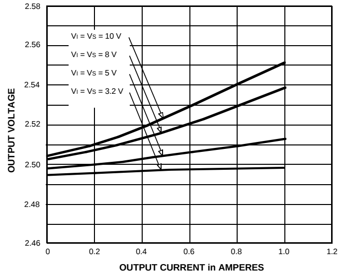
Load regulation
