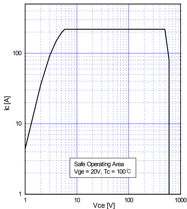
Fig.11 Turn-off SOA
