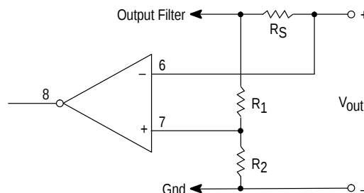
Figure 15. Foldback Current Limiting
