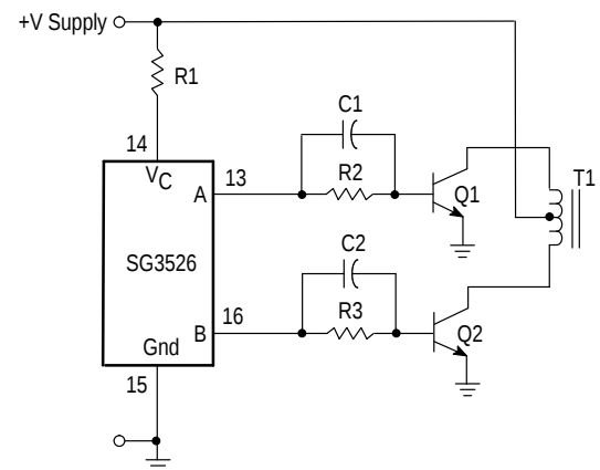
Figure 21. Push-Pull Configuration
