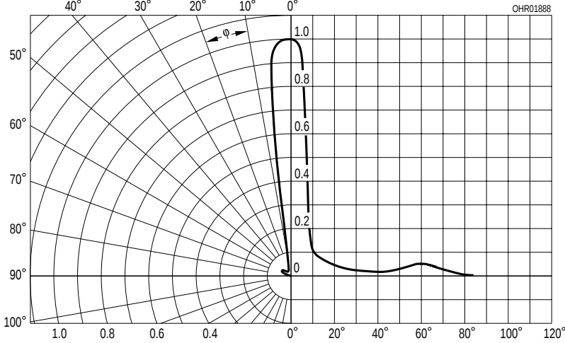
Radiation characteristics, SFH 480 I_{rel} = f(\varphi)
