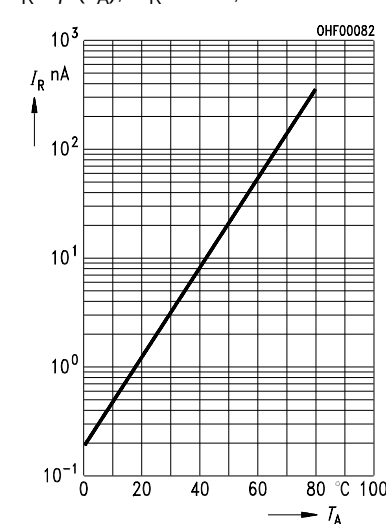
Dark current
