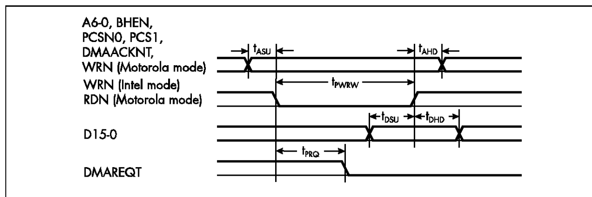
Figure 11. Write Access to Control Registers
