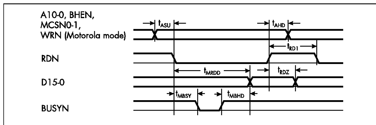
Figure 10. Read Access of Dual Port RAM
