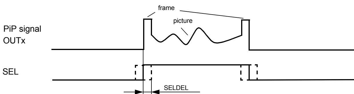
Figure 4-14 Select timing
