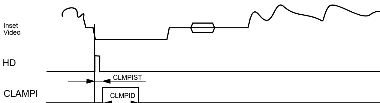
Figure 4-1 Clamping timing
