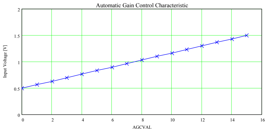
Figure 4-2 AGC characteristic
