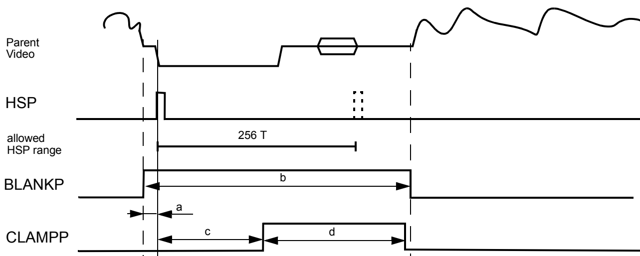
Figure 4-16 PIP horizontal blanking timing
