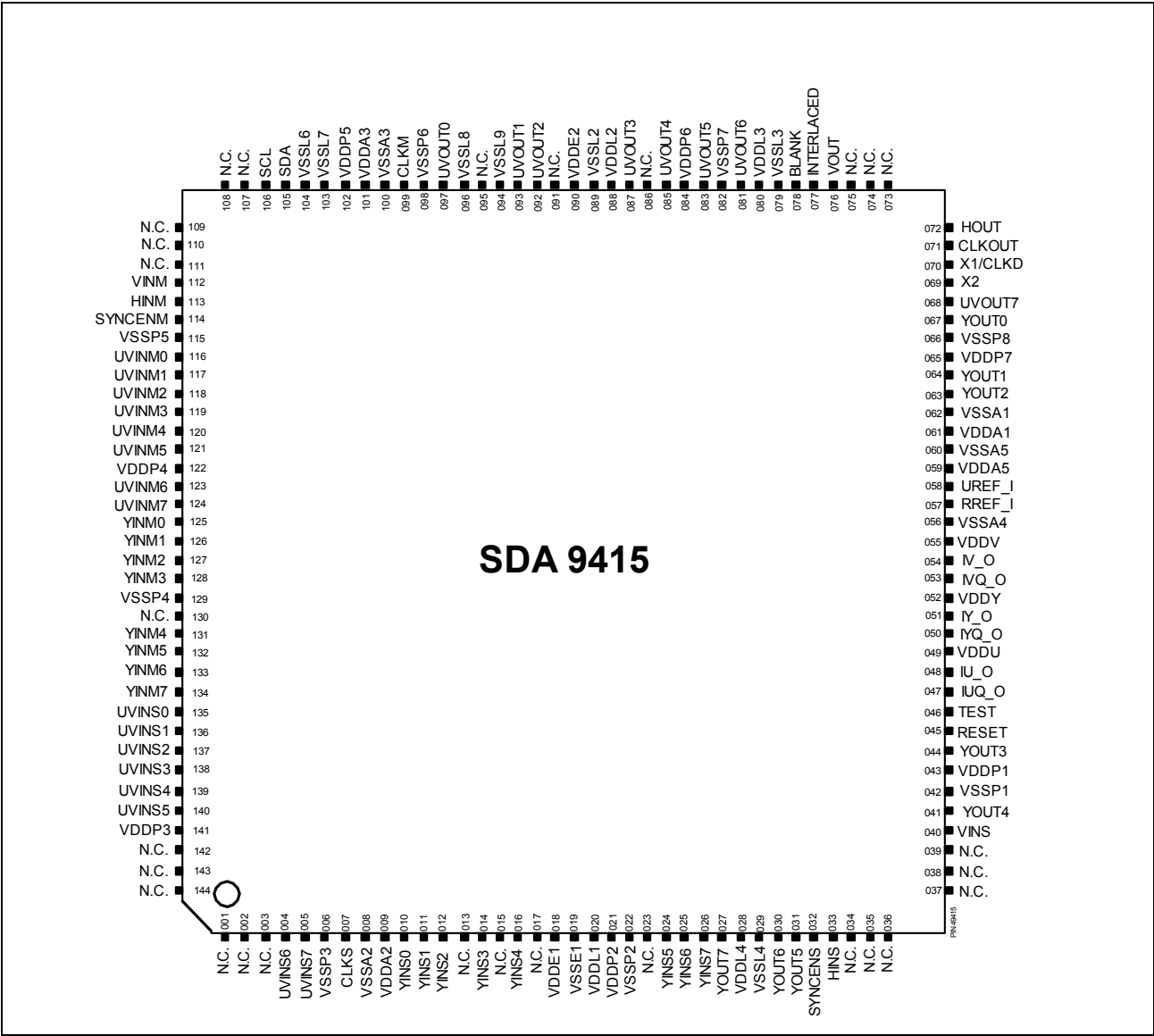
Figure 3 Pin configuration
