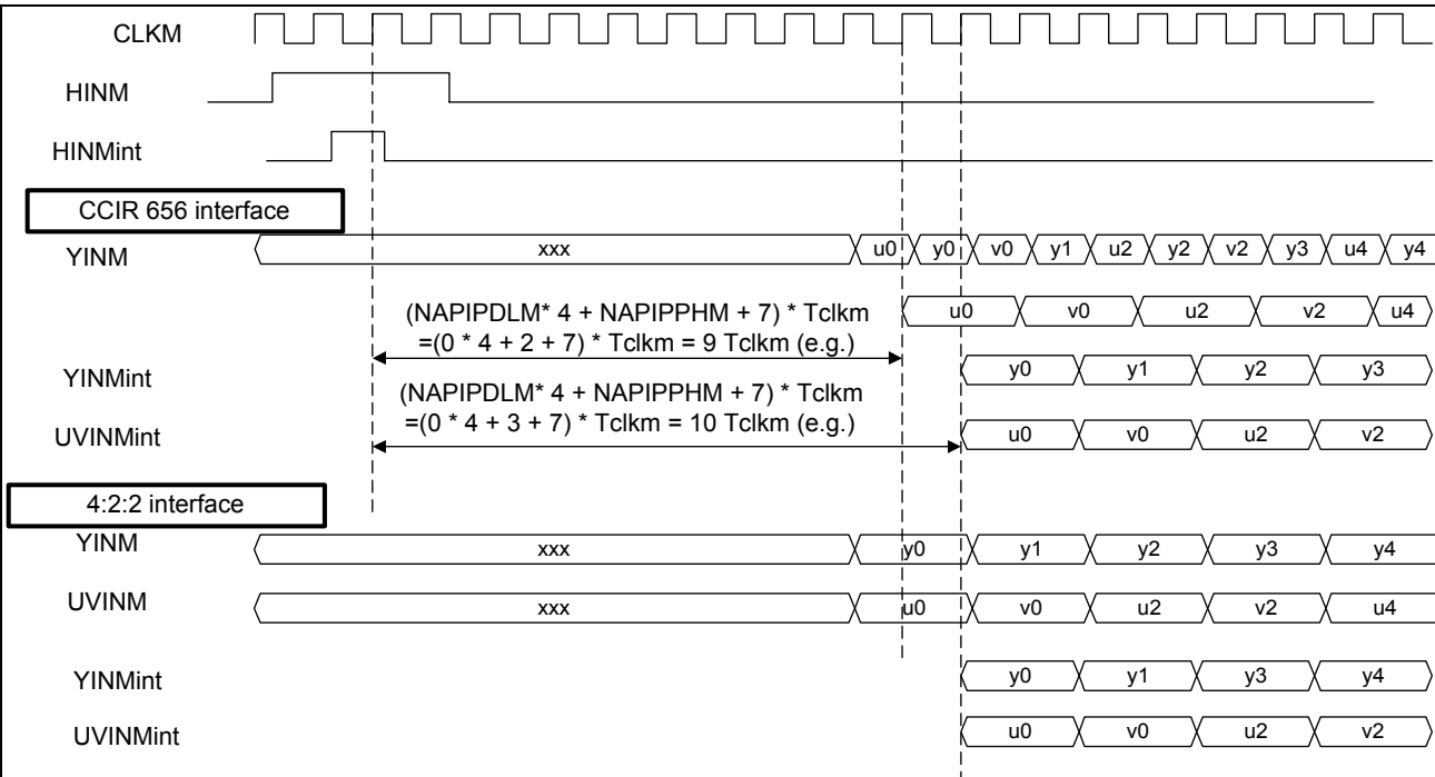
Figure 11 Input timing
