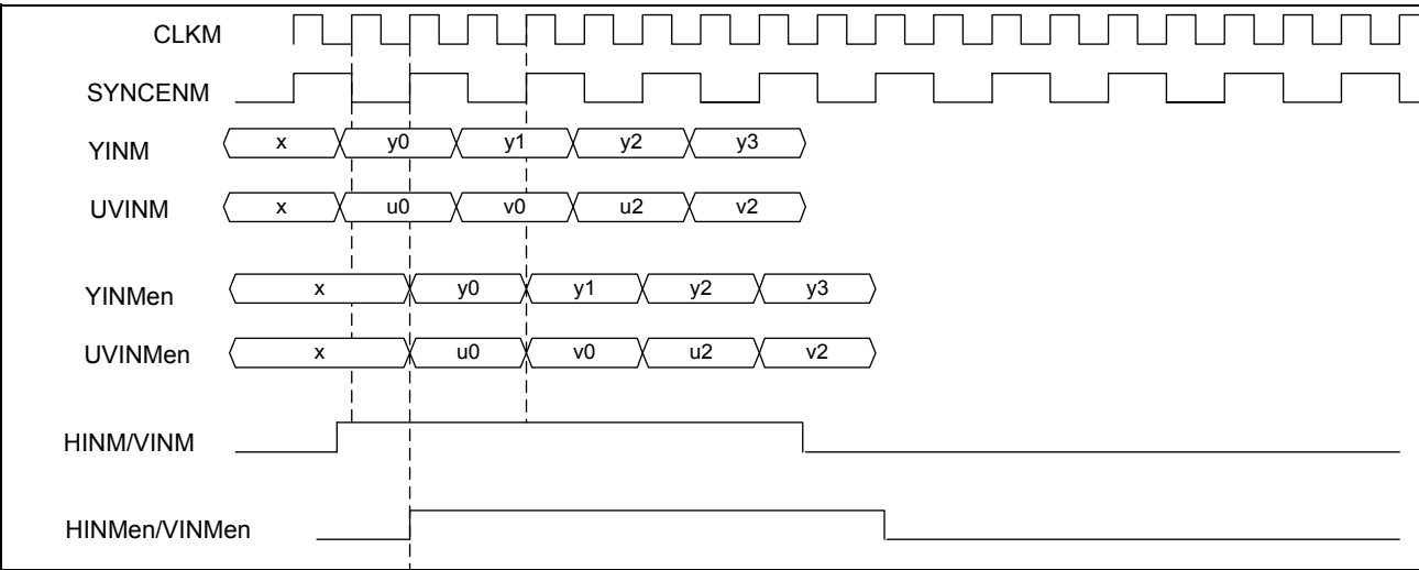
Figure 10 SYNCENM/SYNCENS signal
