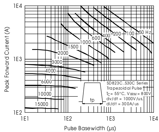
Fig. 37 - Frequency Characteristics
