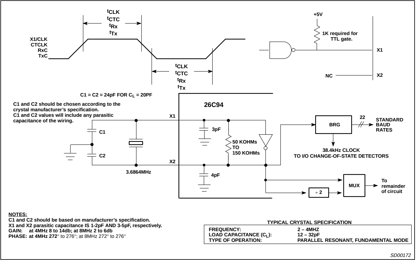
Figure 10. Clock Timing
