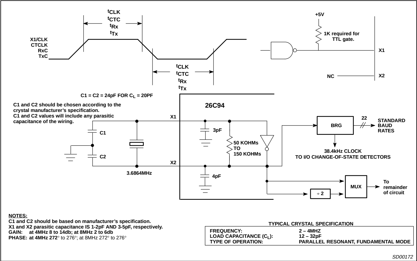
Figure 10. Clock Timing
