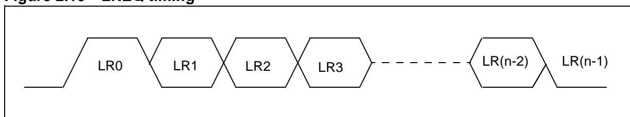
Figure 2.10 LREQ timing
