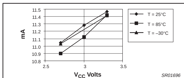
Figure 9. Cellular FM RxTx current
