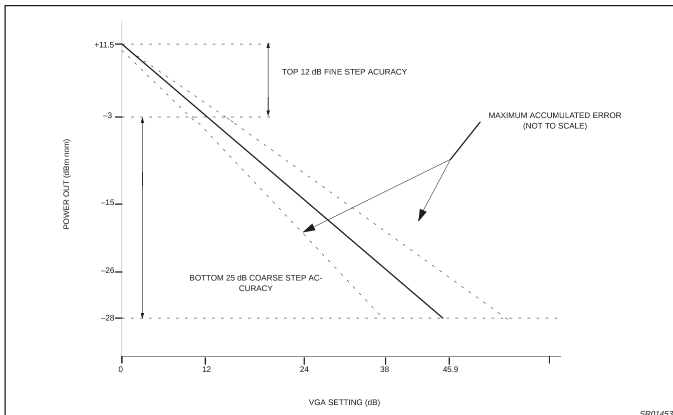
Figure 11. Power Control
