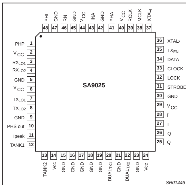
Figure 1. Pin Configuration
