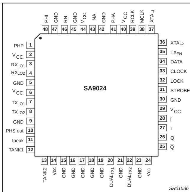
Figure 1. Pin Configuration
