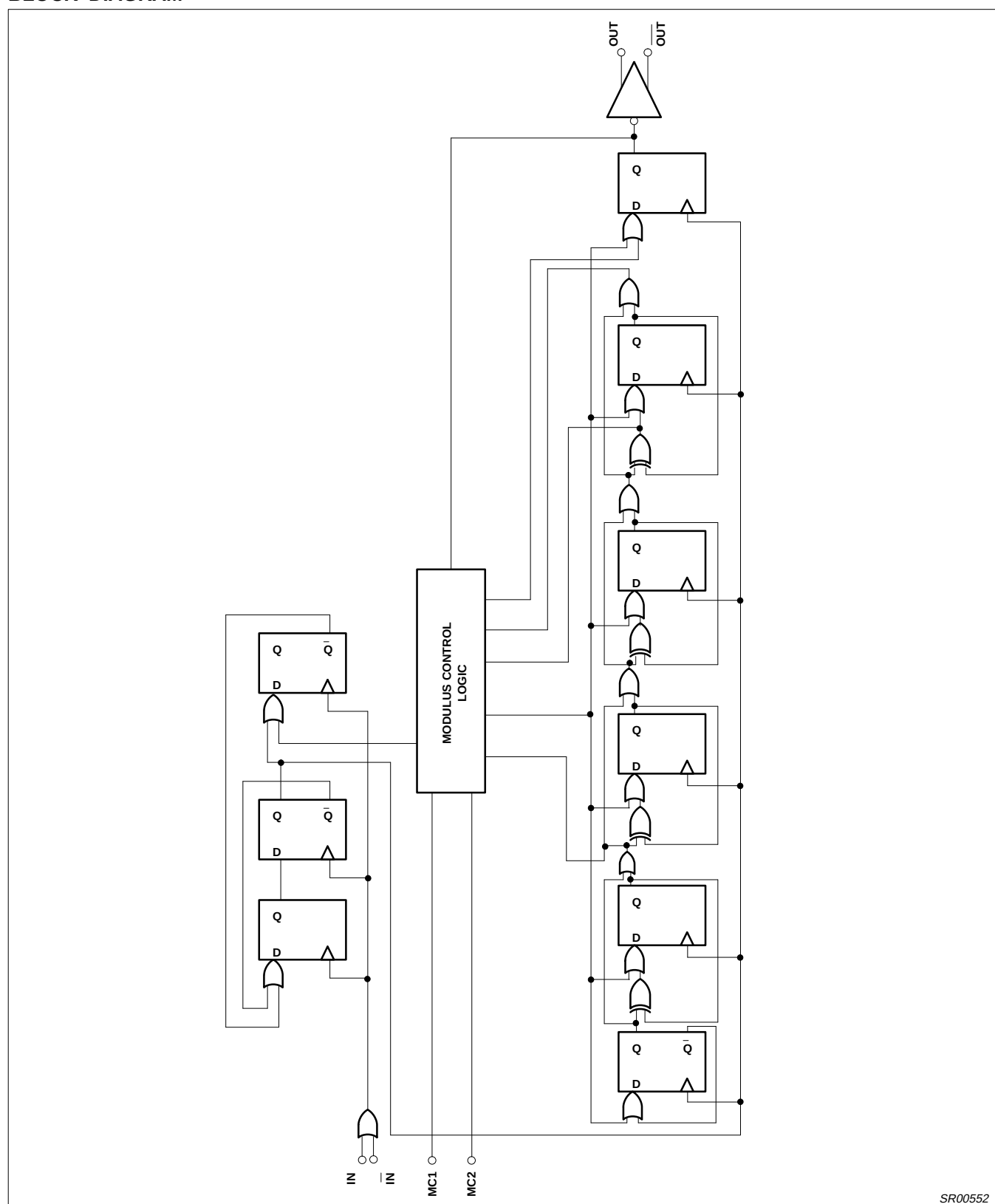
Figure 2. Block Diagram
