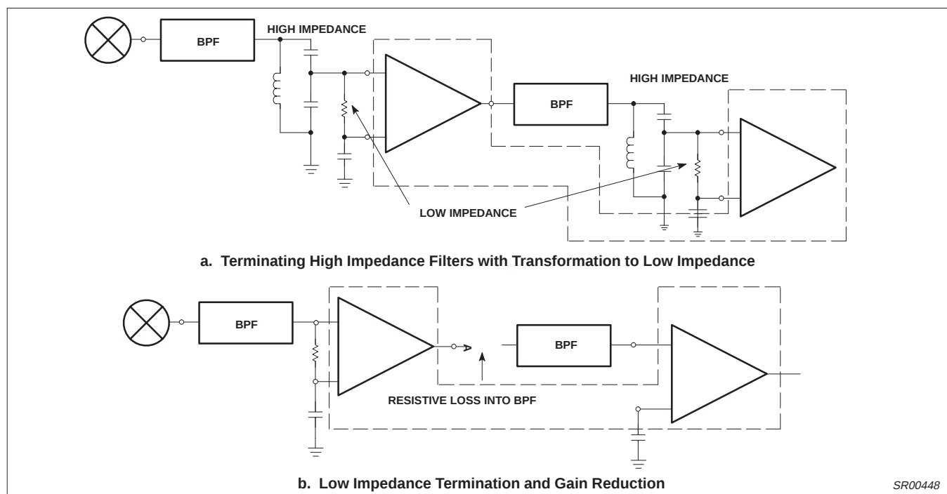
Figure 9. Practical Termination
