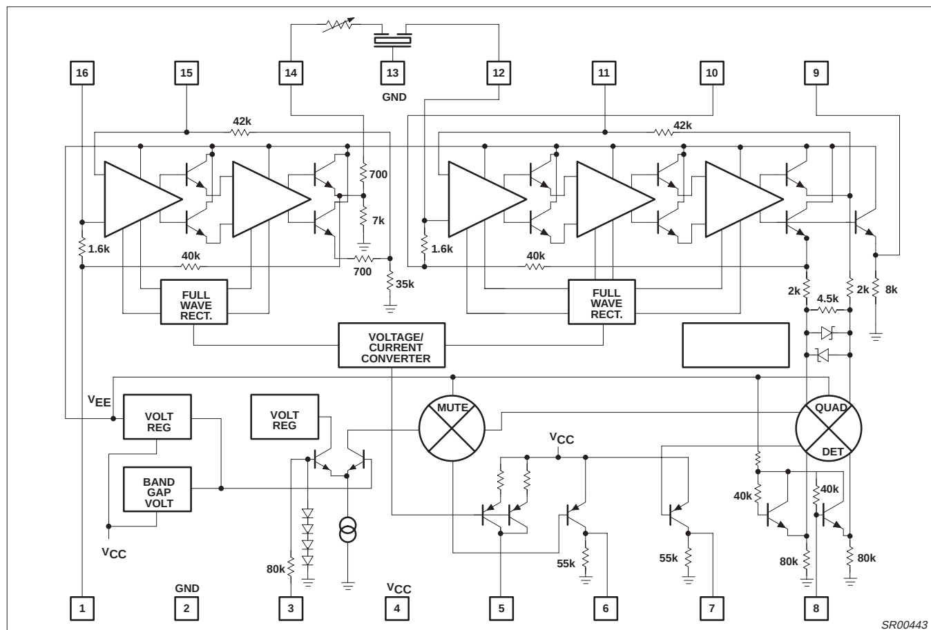
Figure 4. Equivalent Circuit
