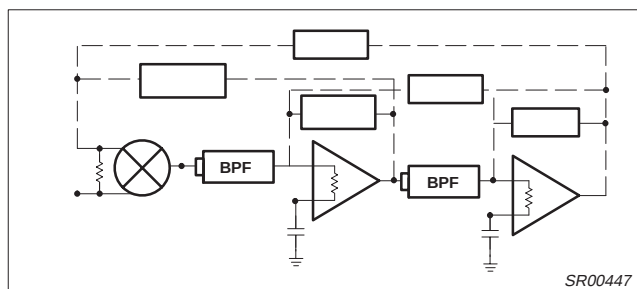
Figure 8. Feedback Paths
