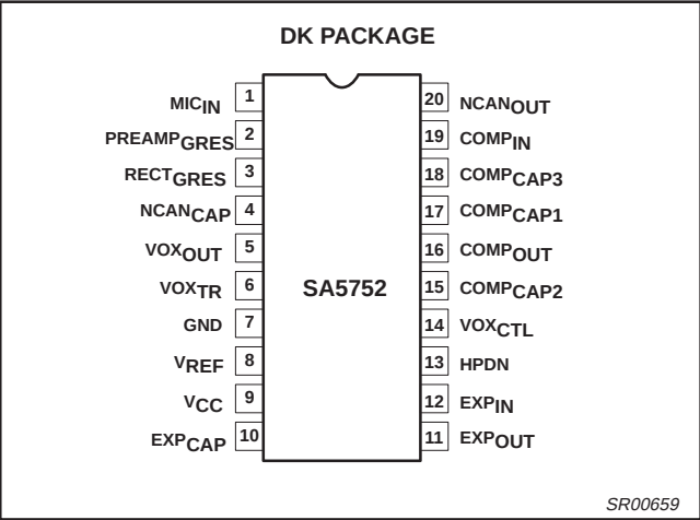
Figure 1. Pin Configuration
