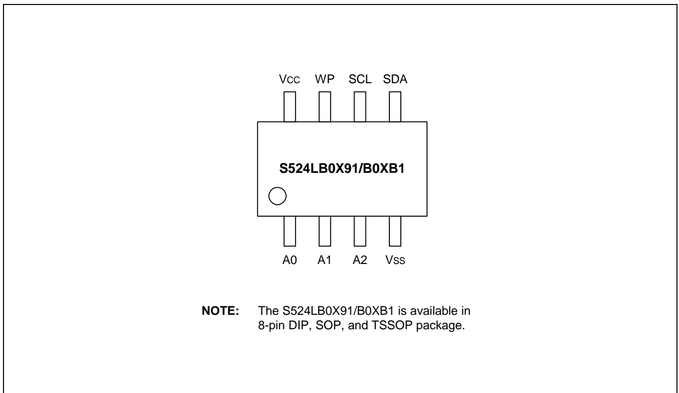
Figure 7-2. Pin Assignment Diagram
