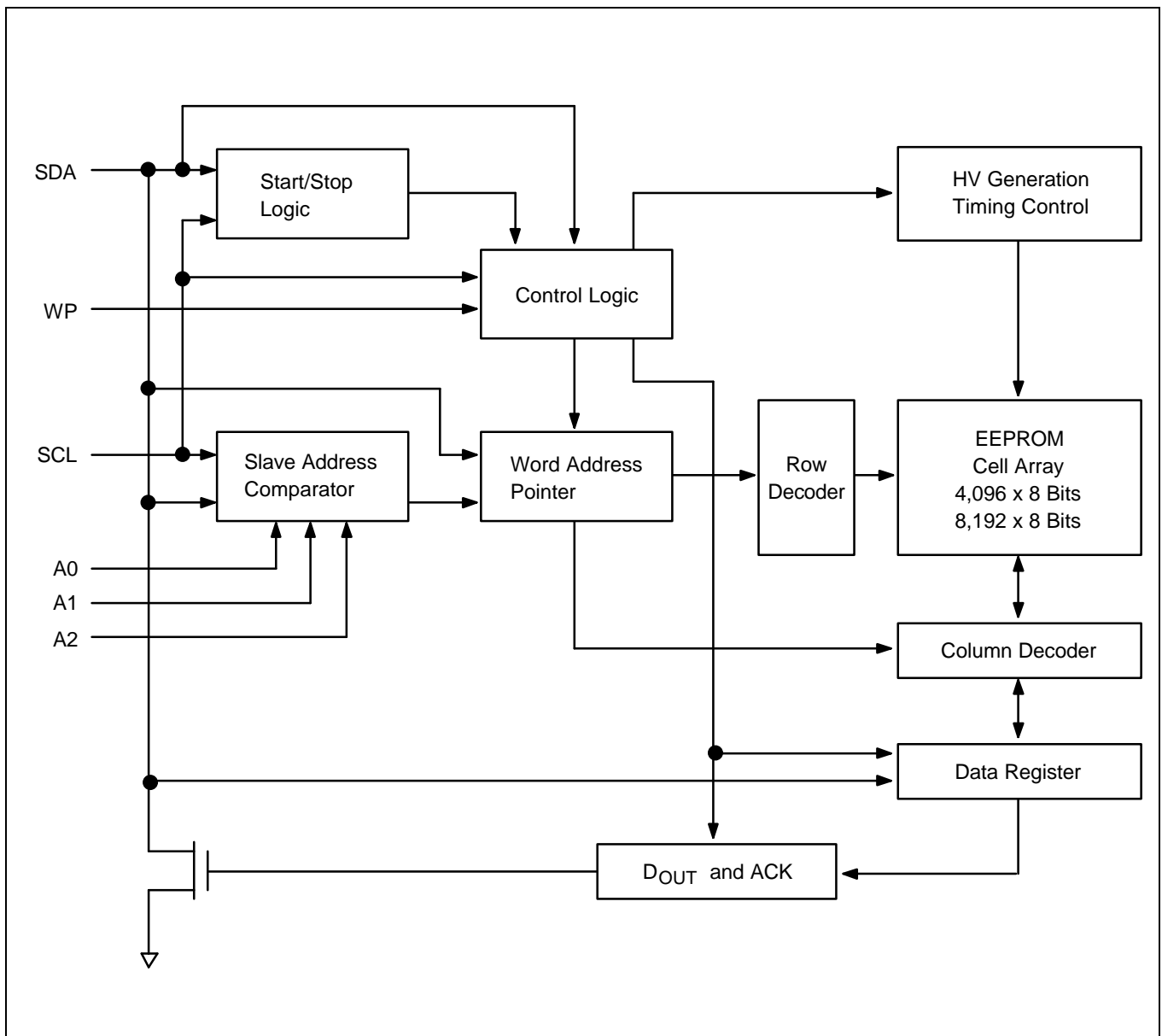
Figure 7-1. S524LB0X91/B0XB1 Block Diagram
