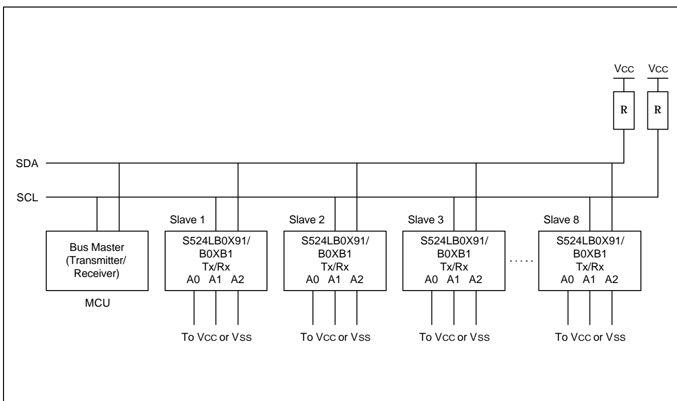
Figure 7-6. Typical Configuration
