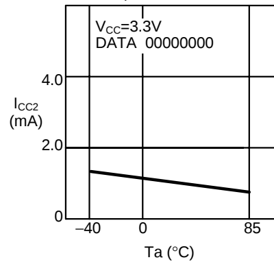
1.8 Standby current consumption I_{SB} - Ambient temperature T_a
