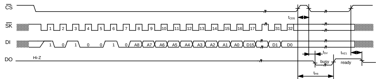
Figure 6 PROGRAM Timing
