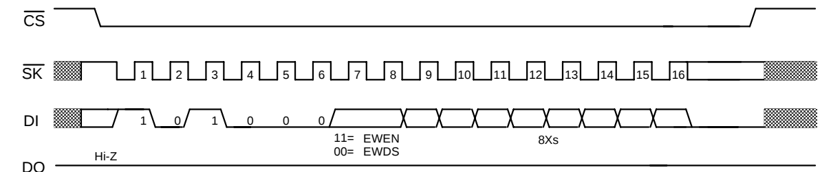
Figure 7 EWEN/EWDS Timing
