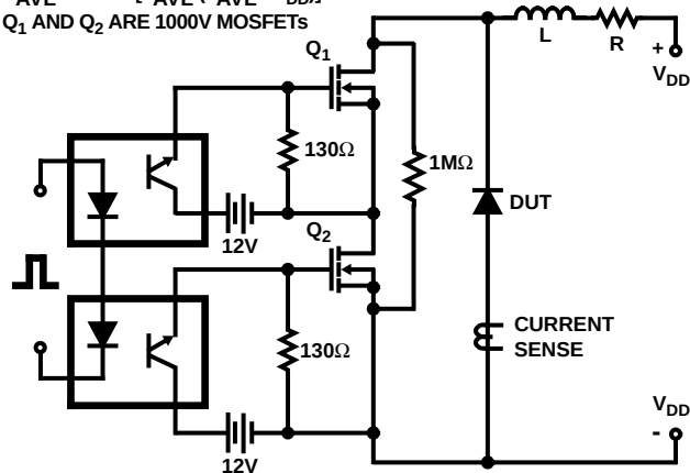
FIGURE 7. AVALANCHE ENERGY TEST CIRCUIT
