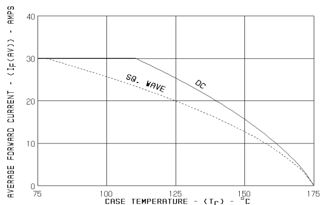
FIGURE 6. CURRENT DERATING CURVE FOR ALL TYPES
