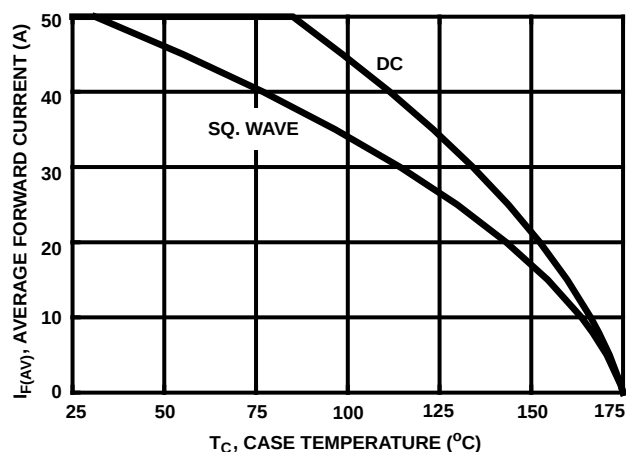
FIGURE 8. CURRENT DERATING CURVE FOR ALL TYPES
