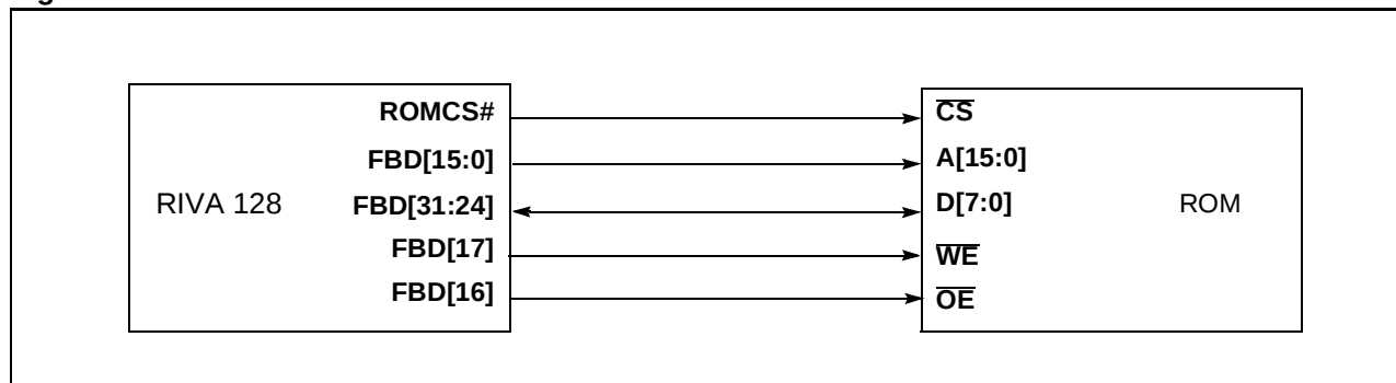
Figure 55. ROM interface
