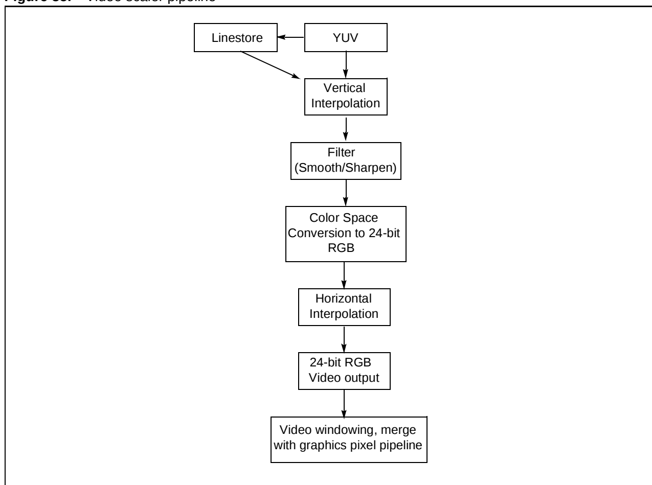
Figure 35. Video scaler pipeline
