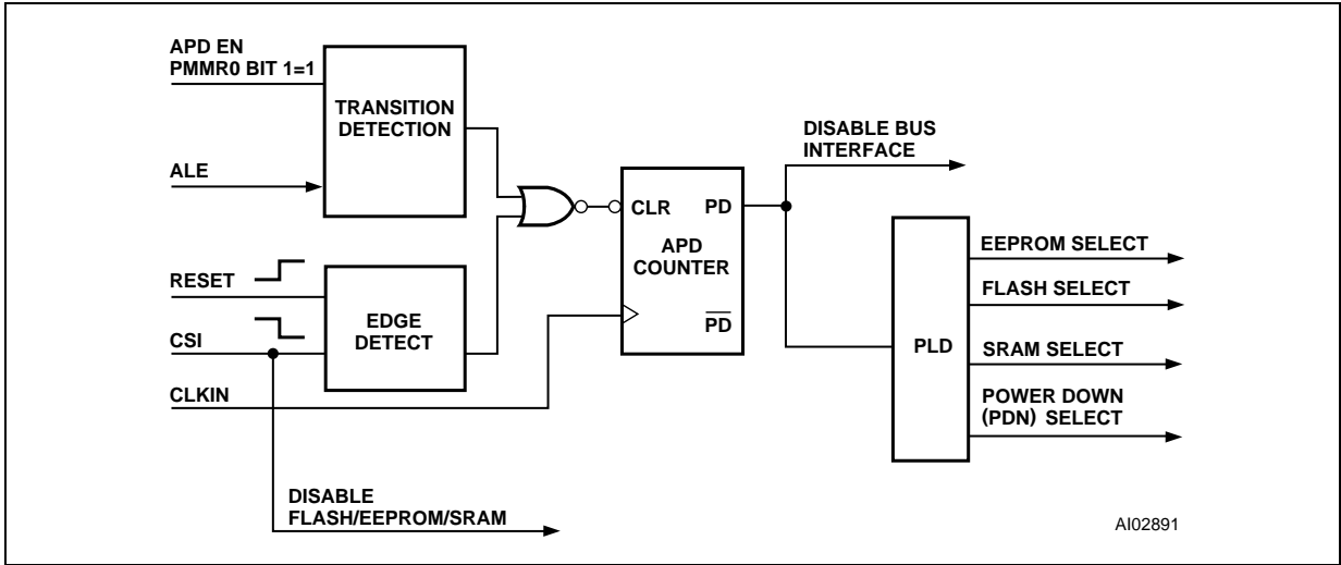
Figure 29. APD Unit
