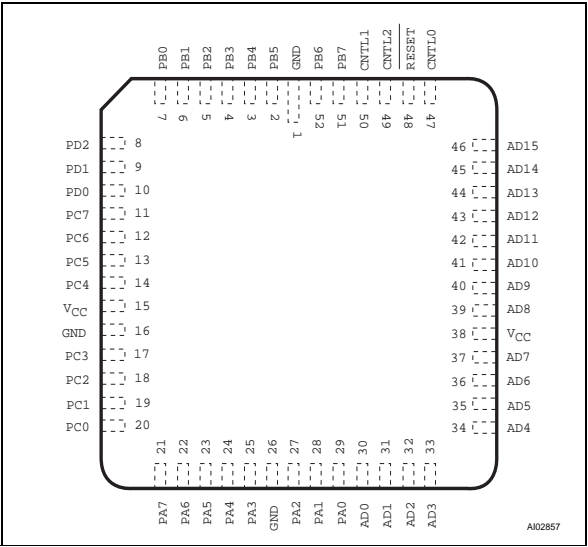
Figure 49. PLCC52 Connections
