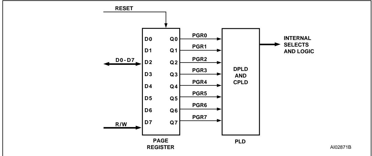
Figure 10. Page Register
