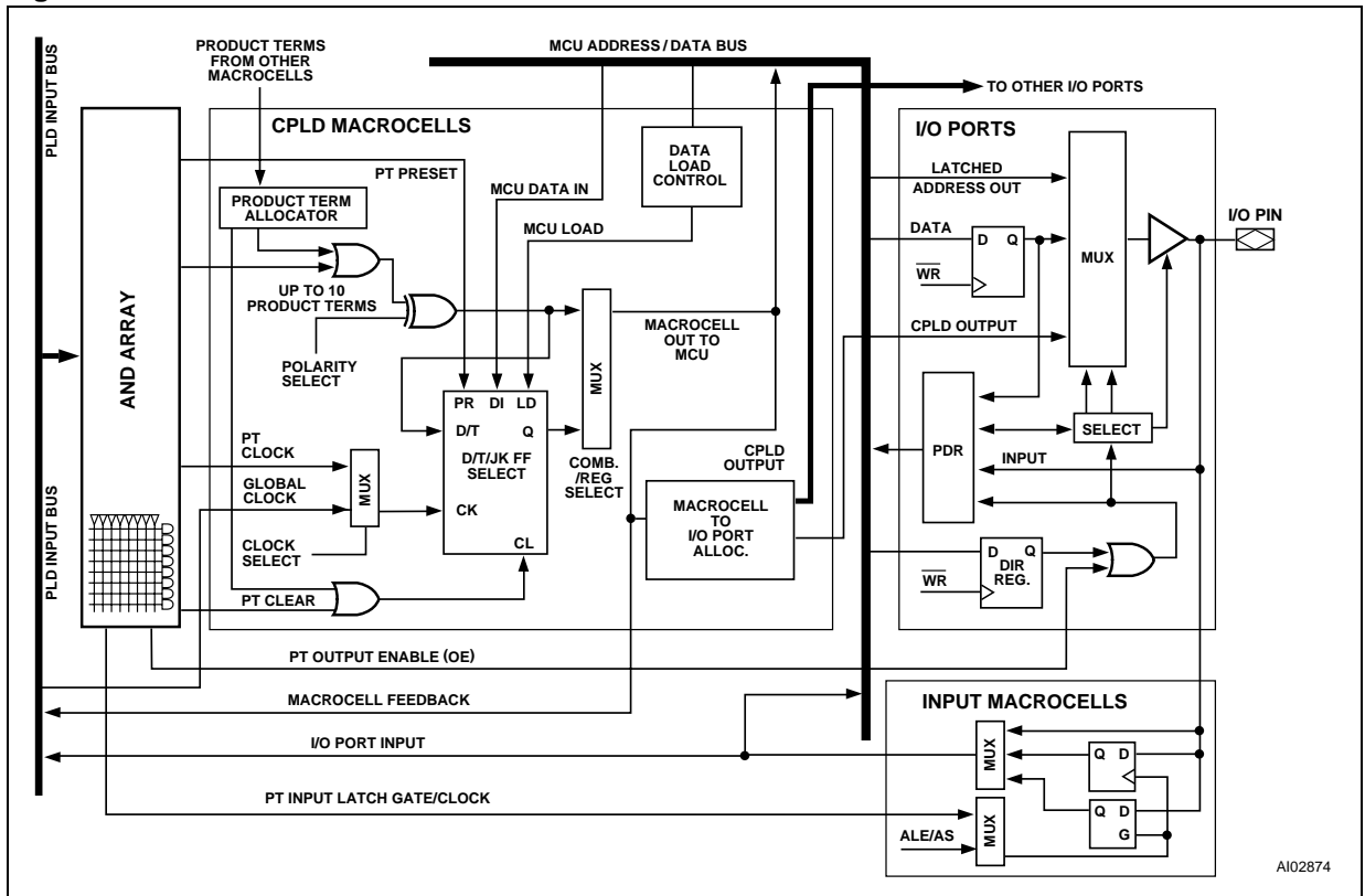
Figure 13. Macrocell and I/O Port
