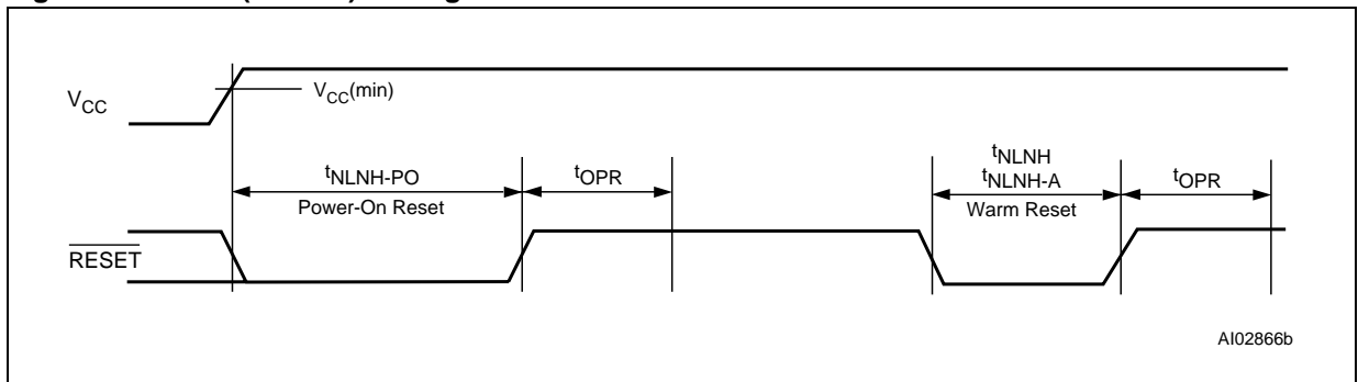
Figure 31. Reset (RESET) Timing
