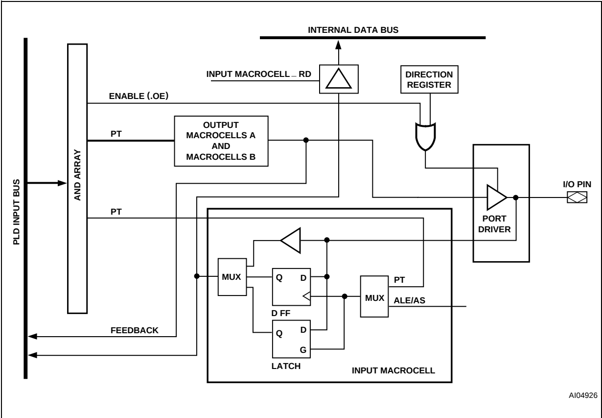
Figure 16. Input Macrocell
