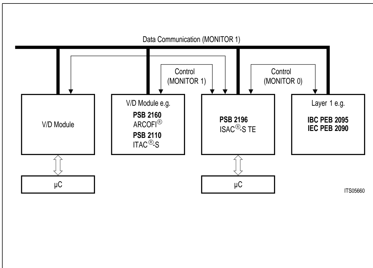
Figure 17 Examples of MONITOR Channel Applications
