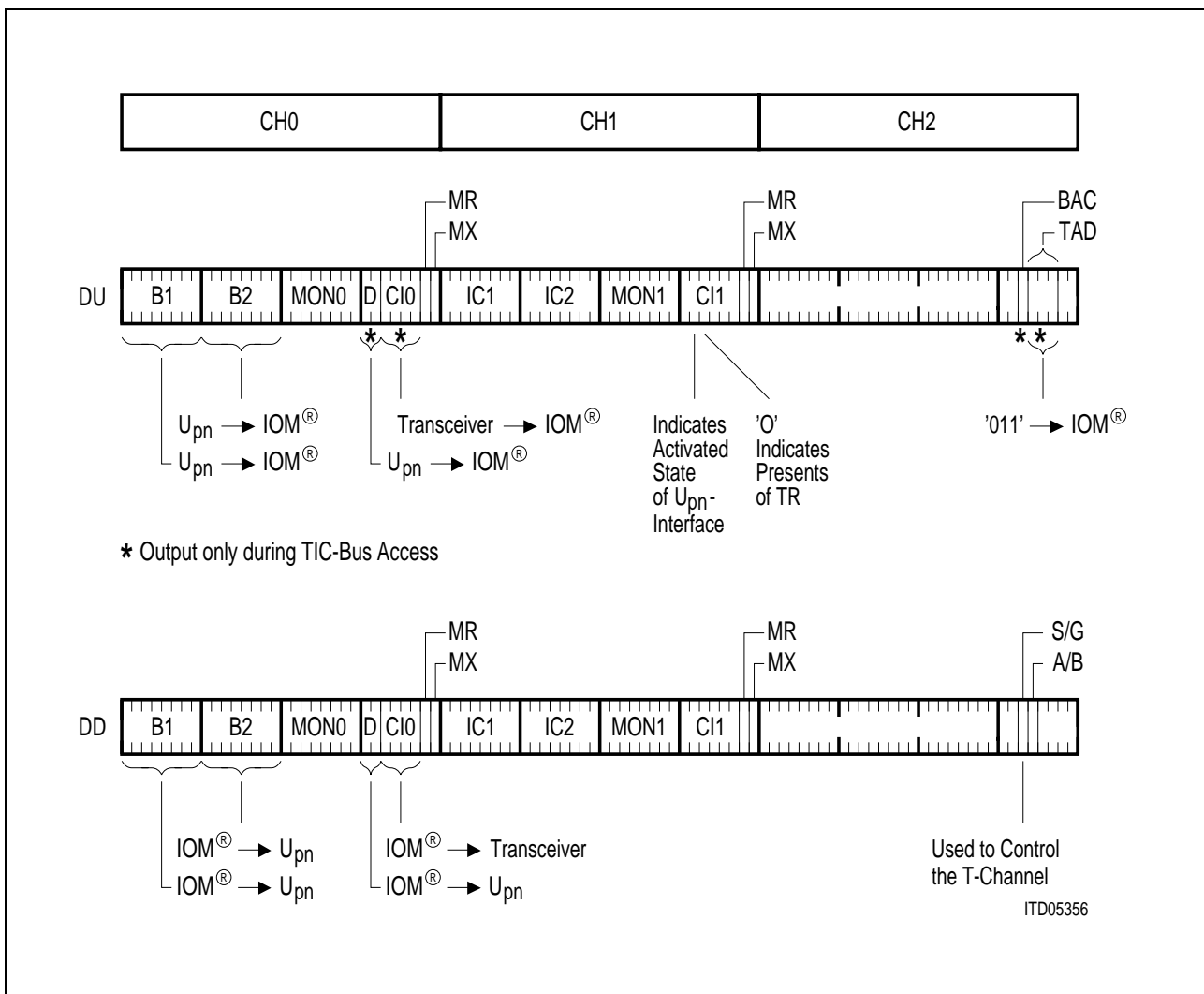
Figure 37 IOM ® -2 Frame Structure in TR-Mode
