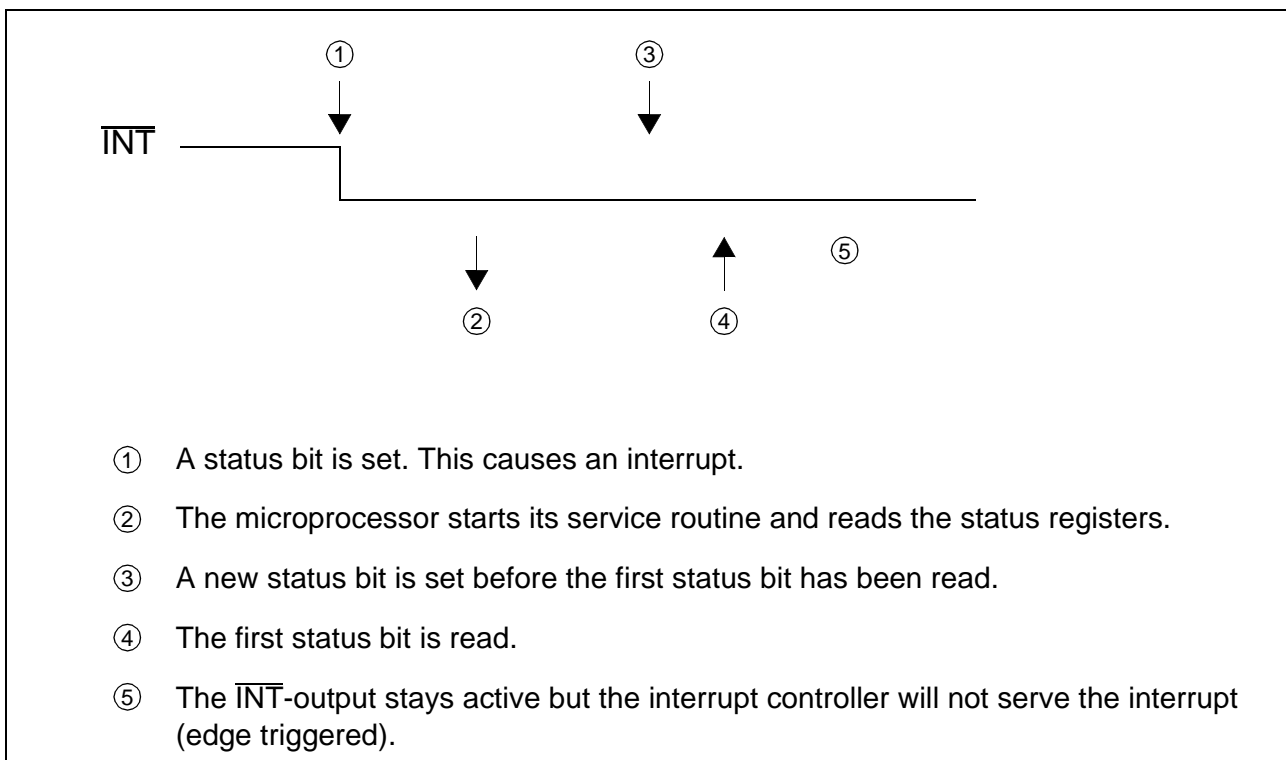
Figure 40 \overline{\text{INT}} -Handling
