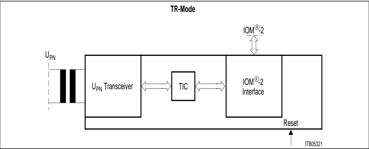
Figure 4 Block Diagram of the ISAC ® -P TE TR-Mode
