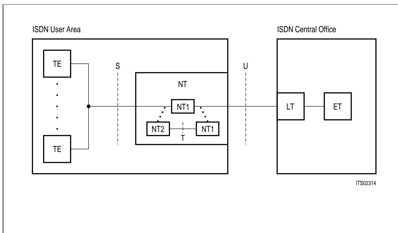
Figure 3 ISDN-Basic Subscriber Access Architecture
