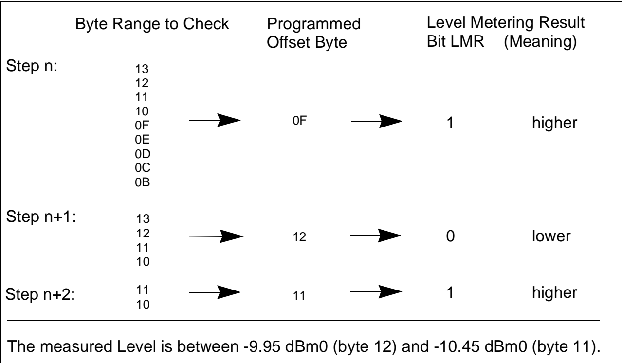
Figure 31 Procedure to find an unknown level with the Level Metering Function
