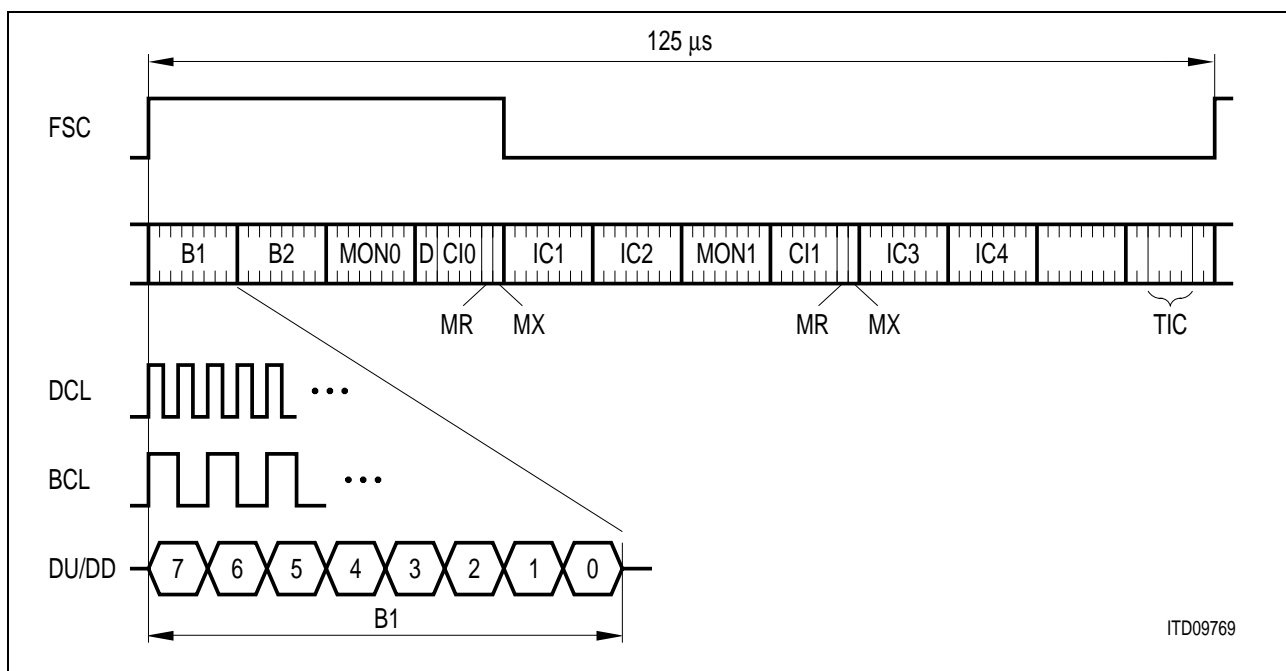
Figure 5 Example for IOM-2 Terminal Mode
