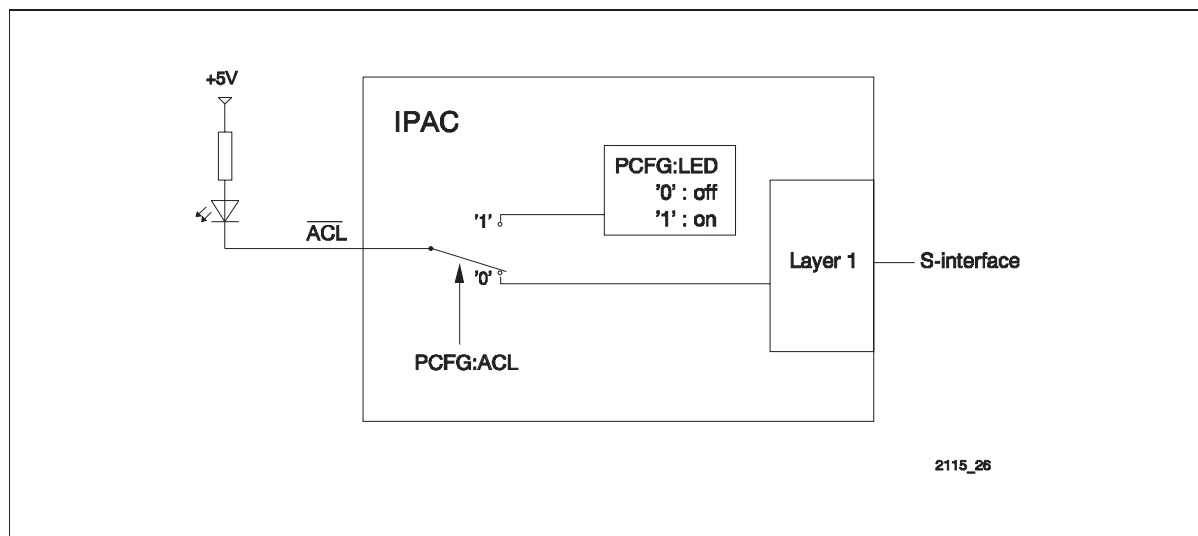
Figure 37 ACL Configuration
