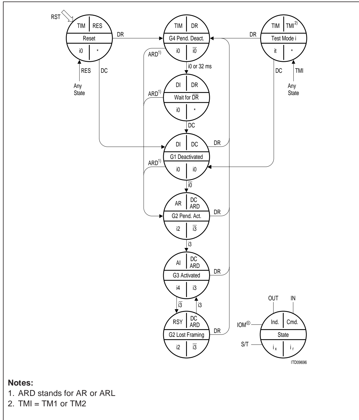
Figure 94 State Transition Diagram in LT-S Mode
