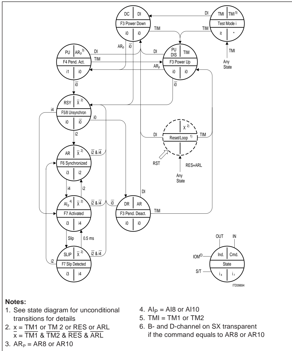
Figure 92 State Transition Diagram in TE/LT-T Modes
