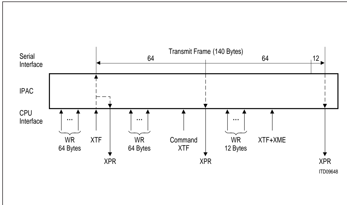
Figure 80 Interrupt Driven Transmission Sequence Example
