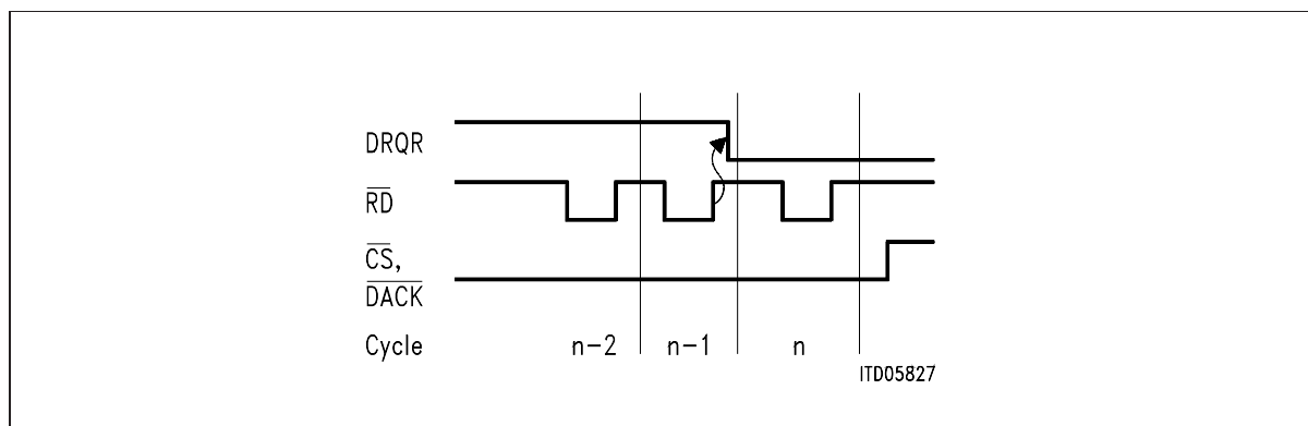
Figure 43 Timing Diagram for DMA-Transfer (fast) Receive ( n = k \times 64 )
