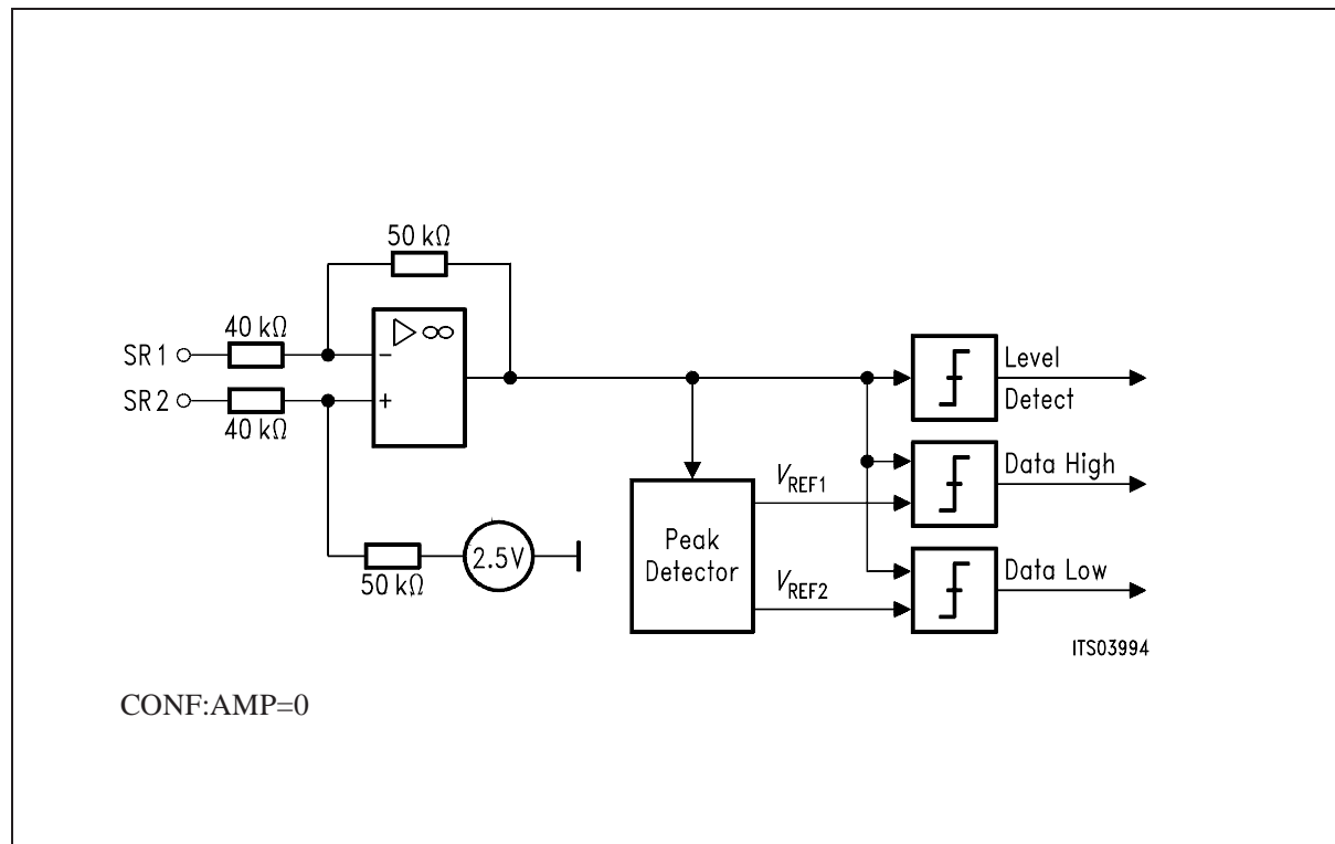
Figure 31 Receiver Circuit
