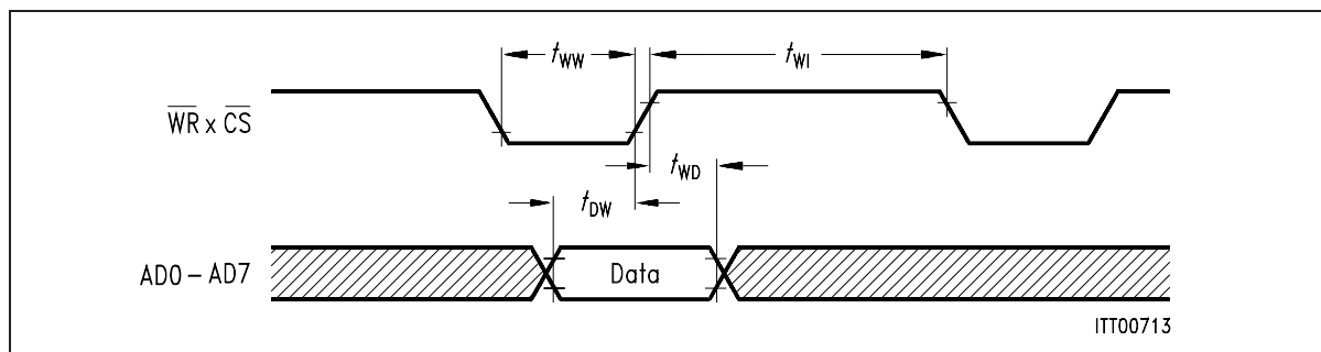
Figure 103 Microprocessor Write Cycle
