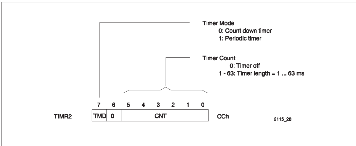
Figure 50 Timer 2 Register
