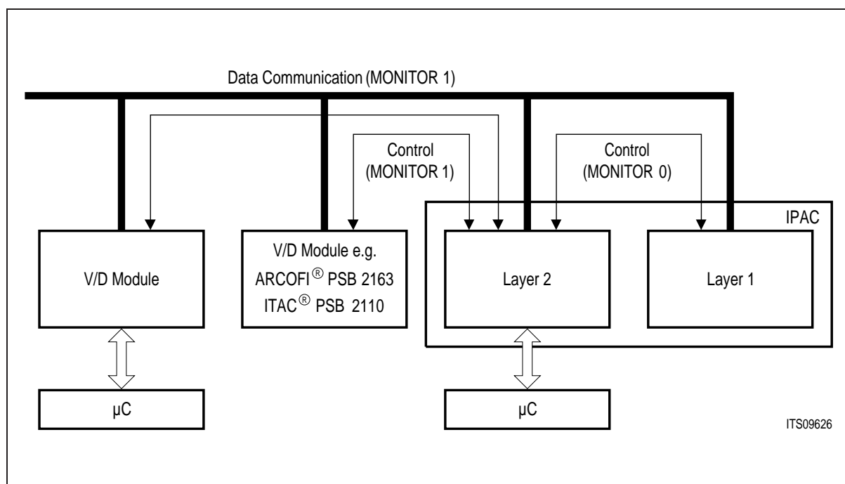
Figure 18 Examples of MONITOR Channel Applications
