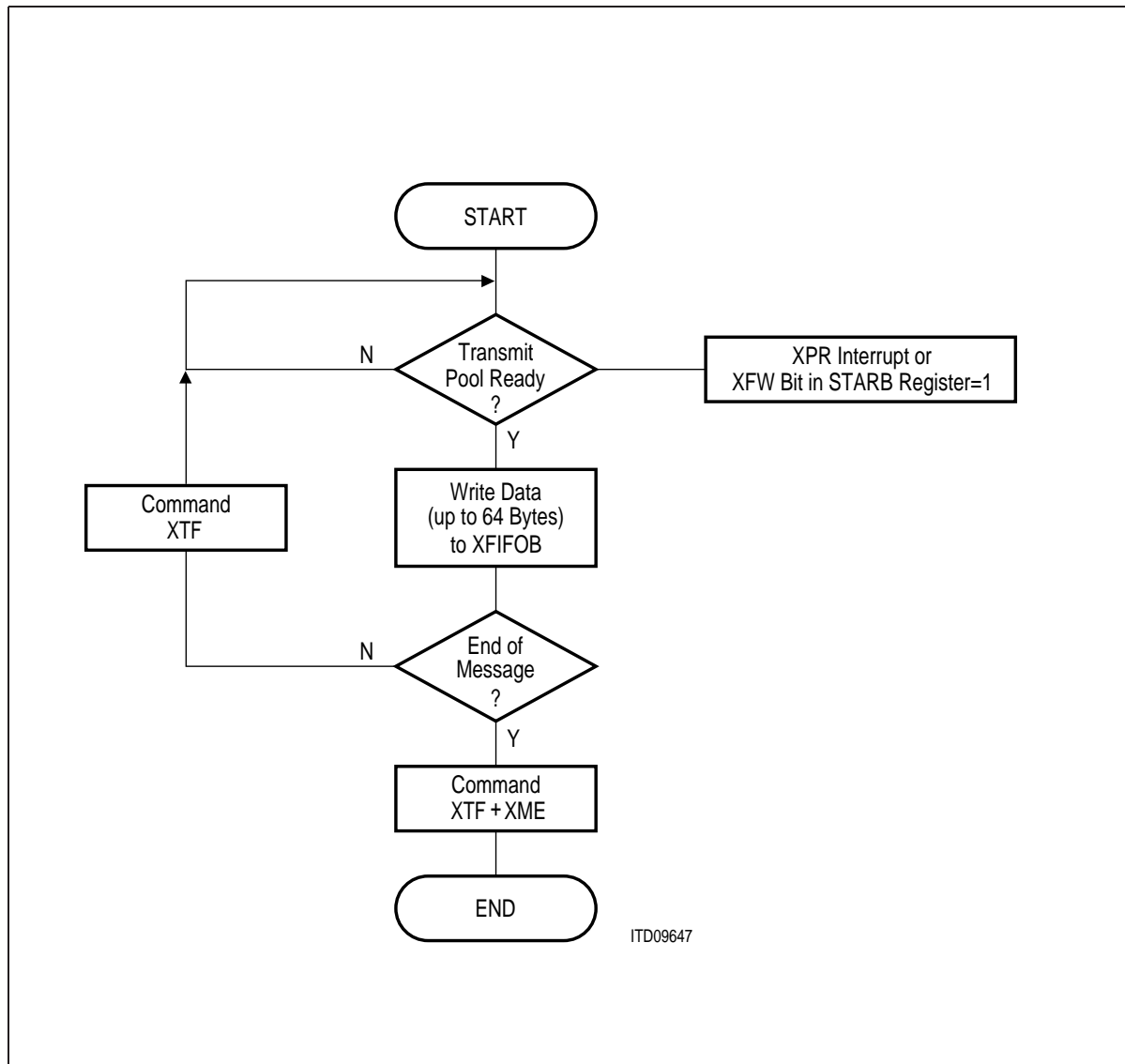
Figure 79 Interrupt Driven Data Transmission (Flow Diagram)
