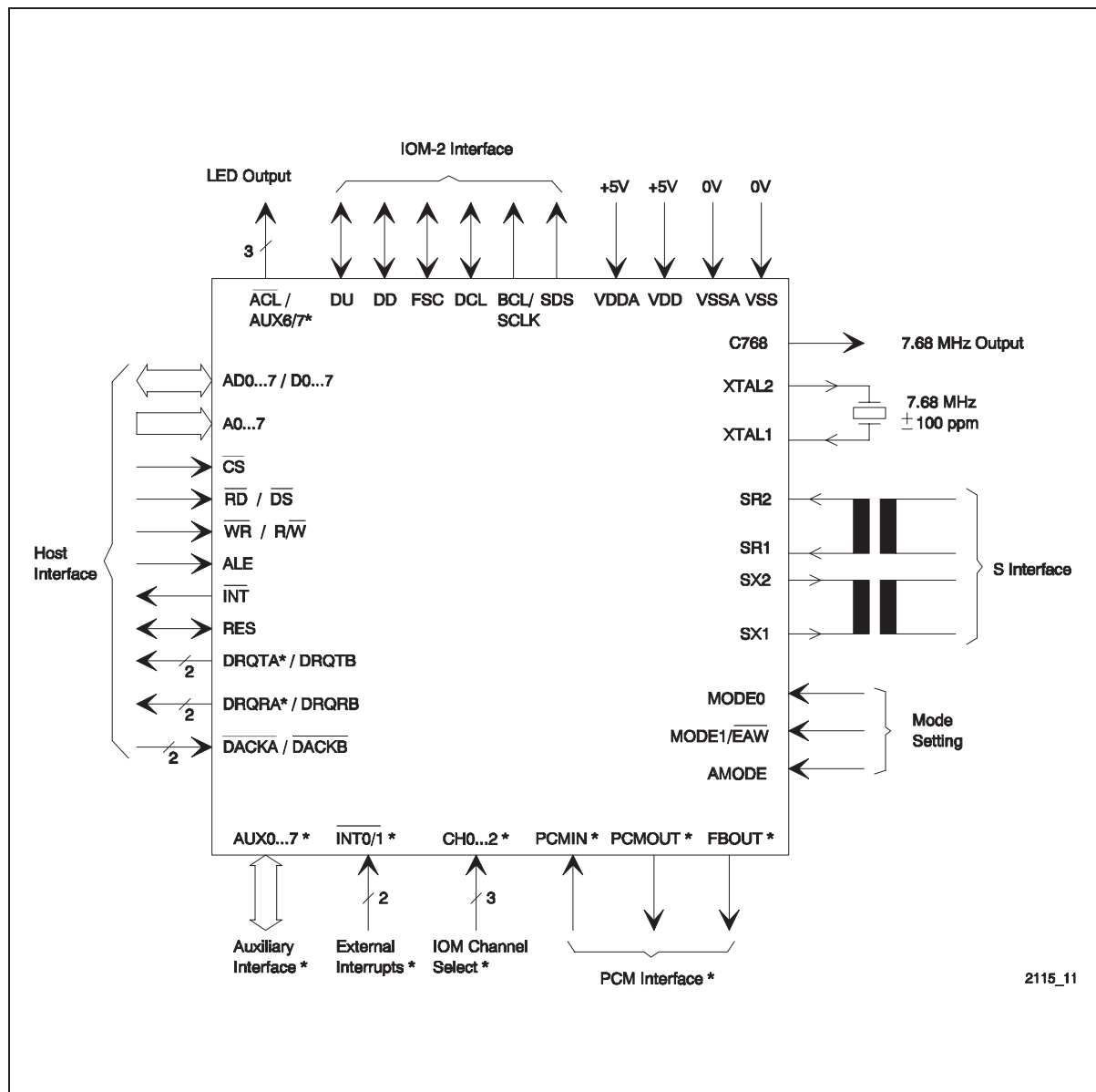
Figure 1 Logic Symbol
