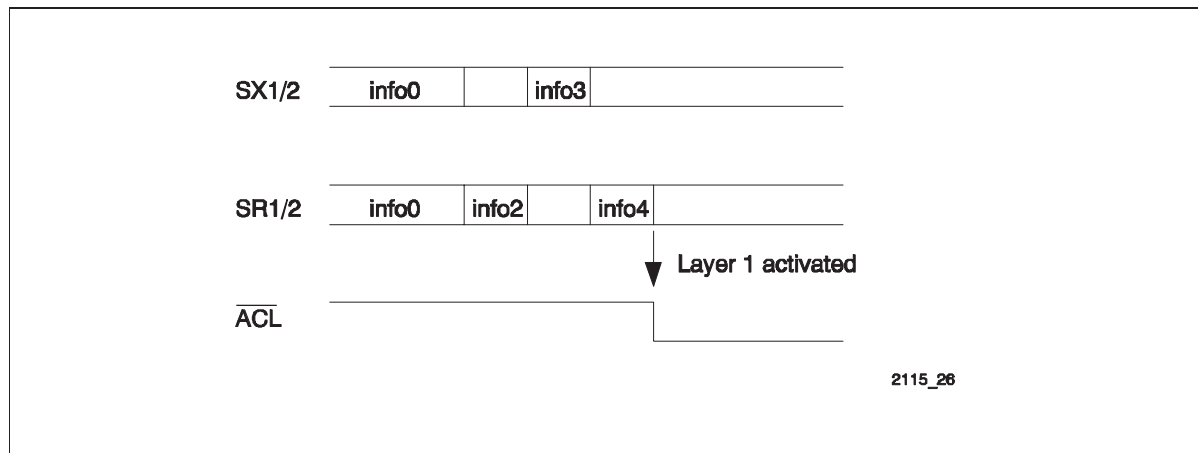
Figure 36 ACL Indication of Activated Layer 1
