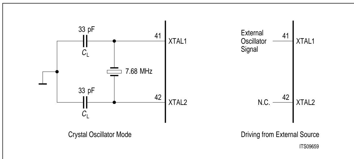
Figure 100 Oscillator Circuits
