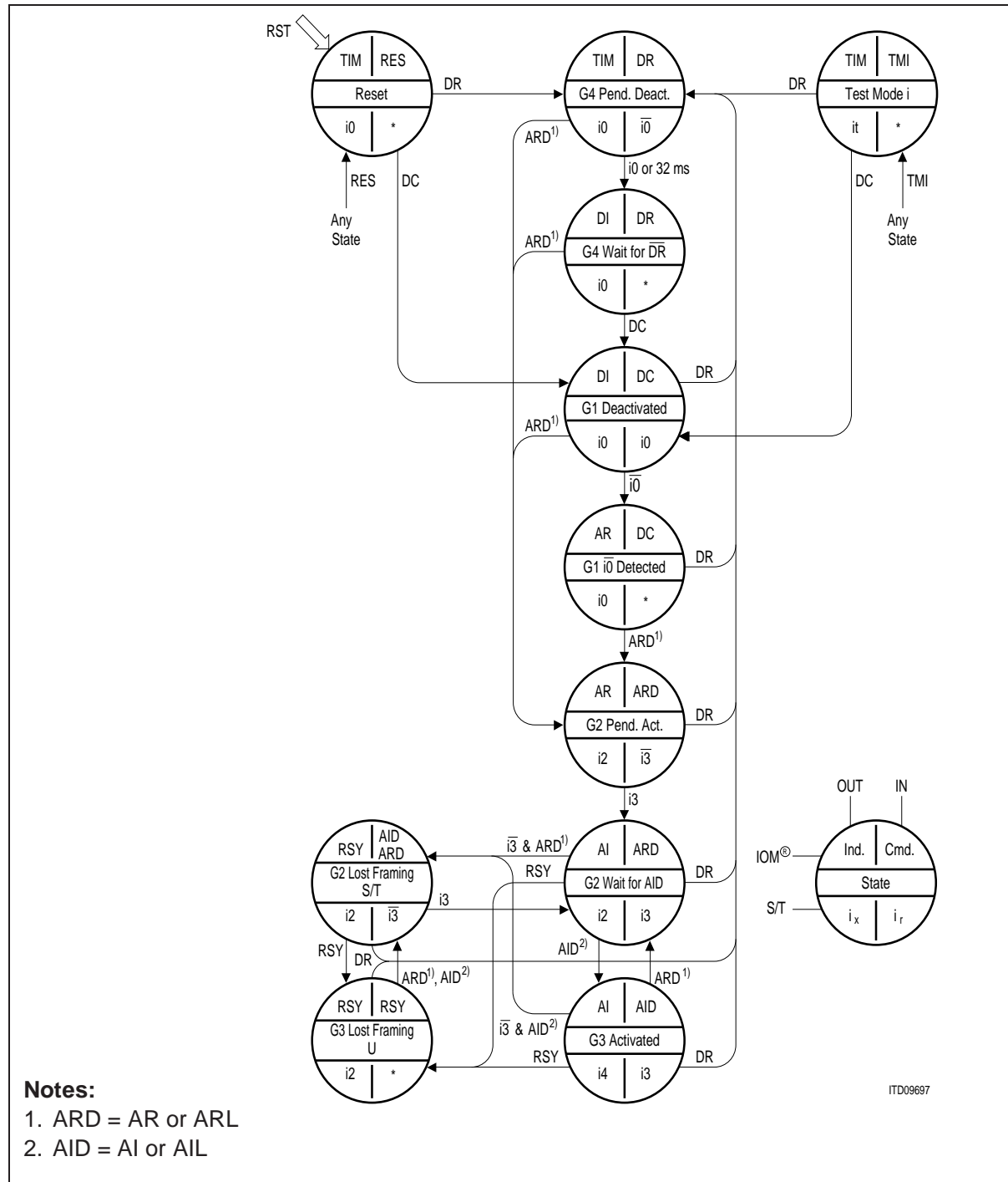
Figure 95 NT Mode State Diagram
