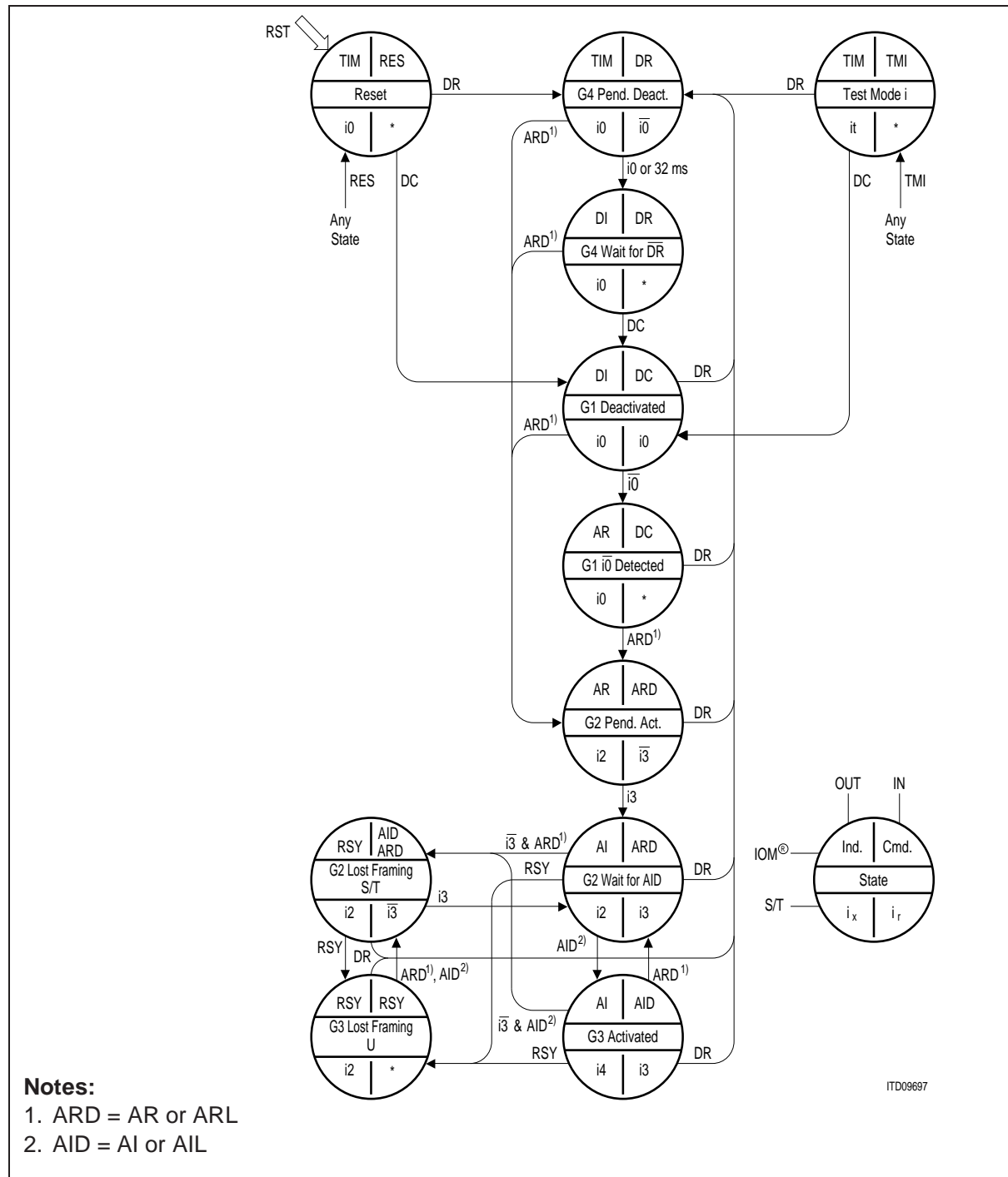
Figure 120 NT Mode State Diagram
