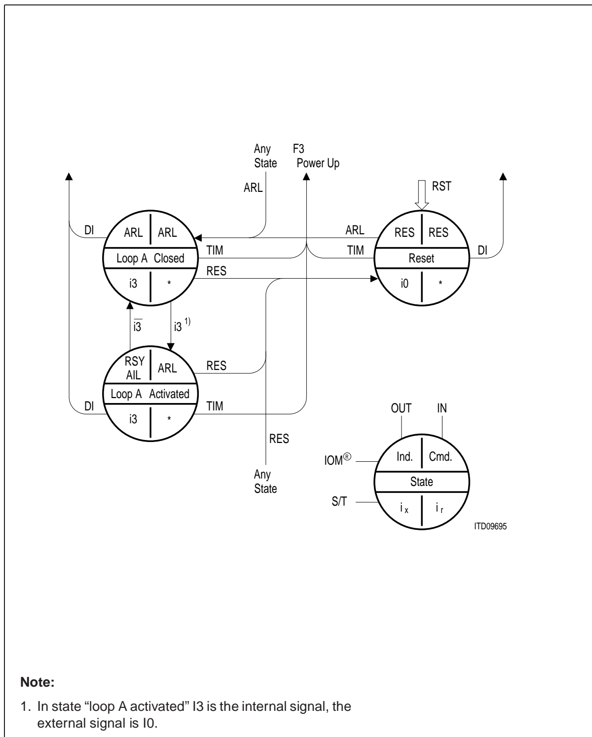
Figure 118 State Diagram of the TE/LT-T Modes, Unconditional Transitions
