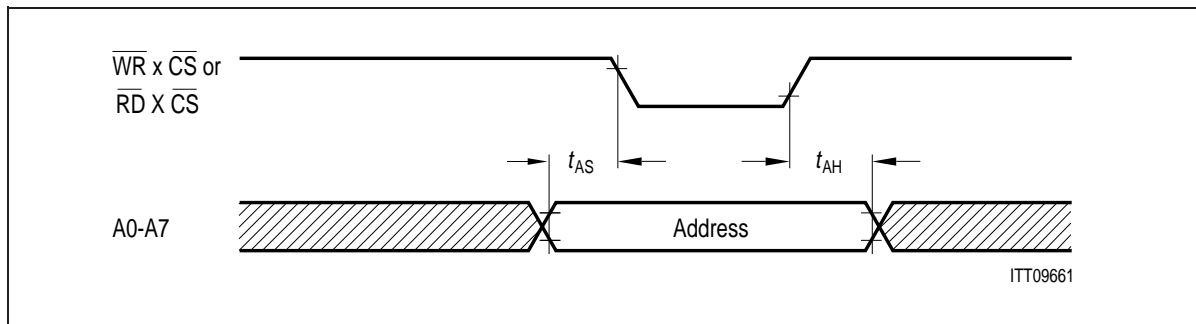
Figure 105 Non-Multiplexed Address Timing
