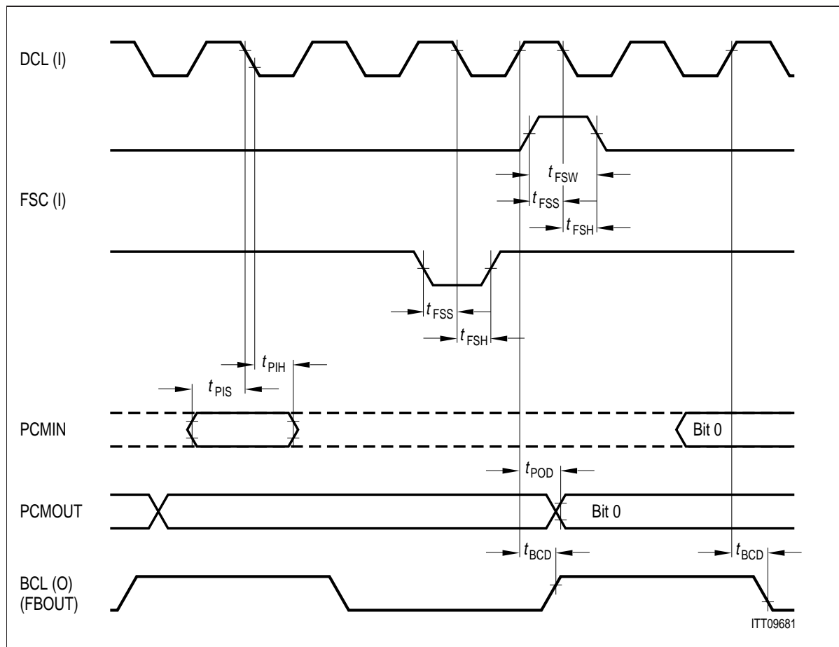
Figure 111 PCM Interface Timing (LT-S, LT-T mode)
