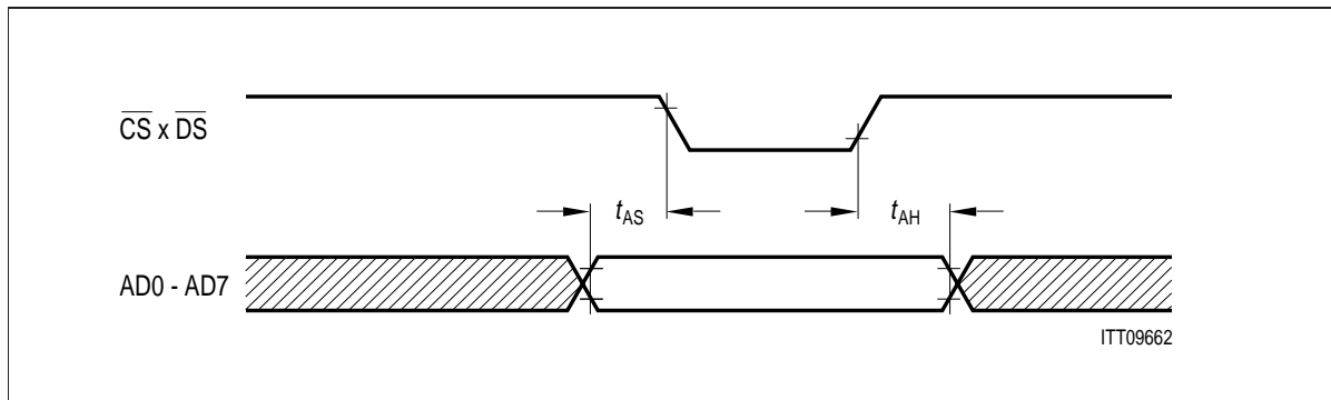
Figure 108 Non-Multiplexed Address Timing
