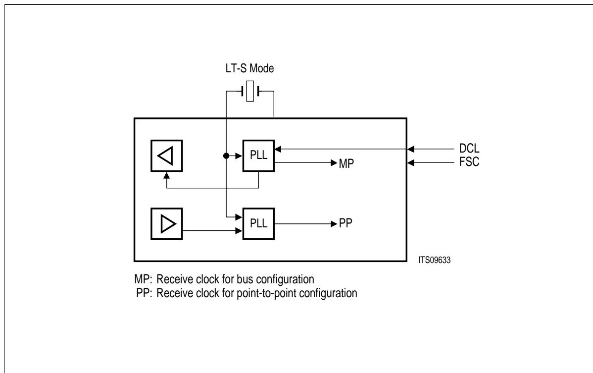
Figure 34 Clock System of the IPAC in LT-S Mode
