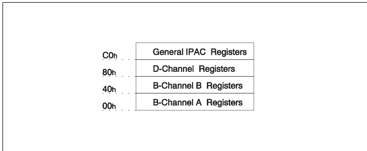
Figure 97 Register mapping
