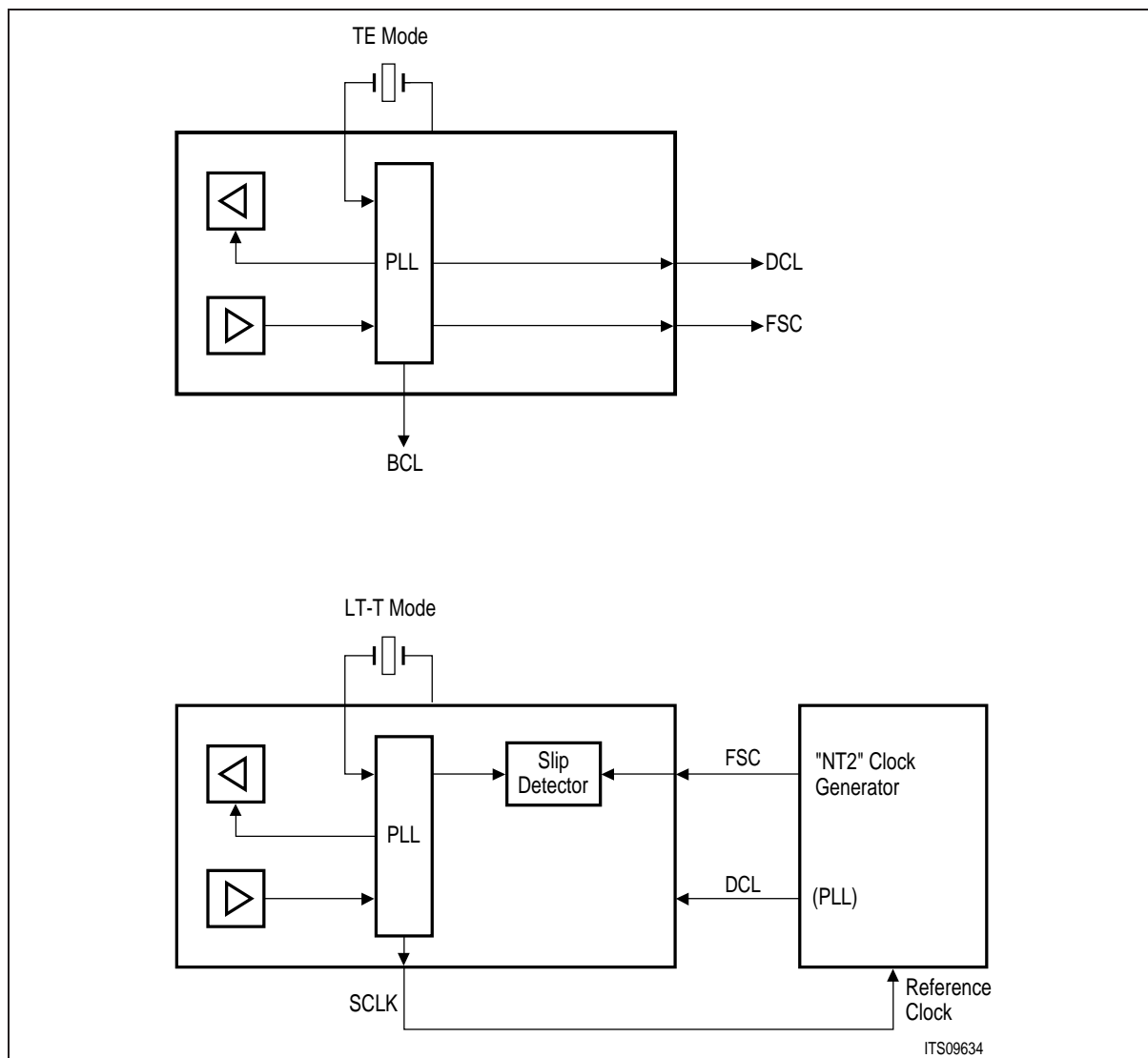
Figure 35 Clock System of the IPAC in TE and LT-T Modes
