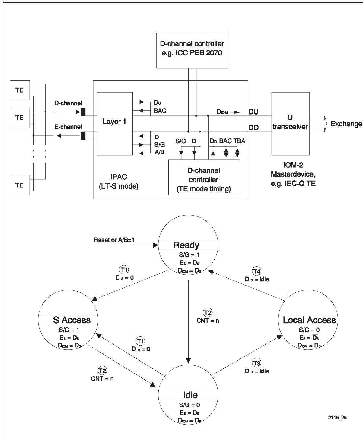
Figure 21 Data Flow for Collision Resolution Procedure in Intelligent NT
