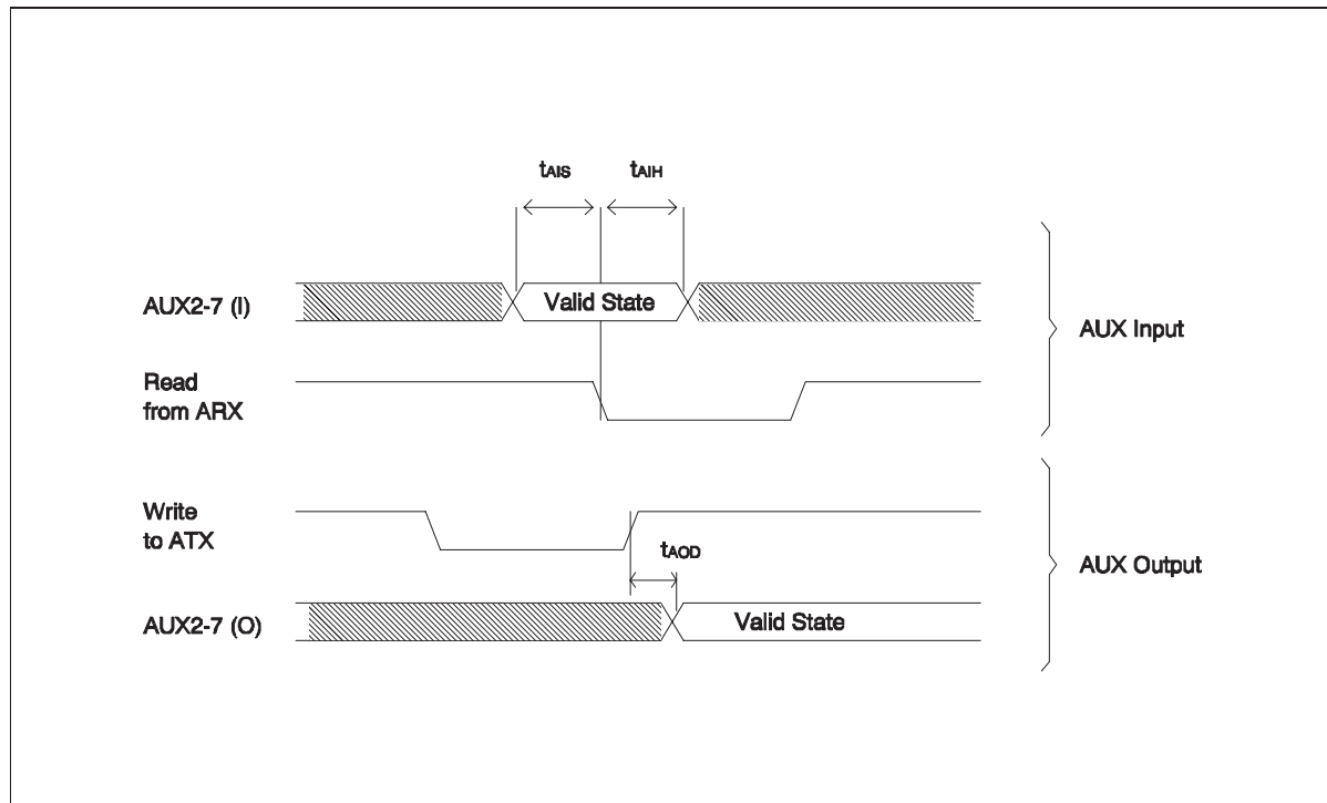
Figure 112 AUX Interface I/O Timing
