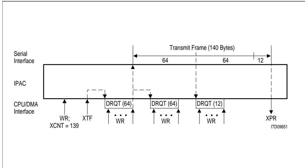
Figure 83 DMA Driven Transmission Sequence Example
