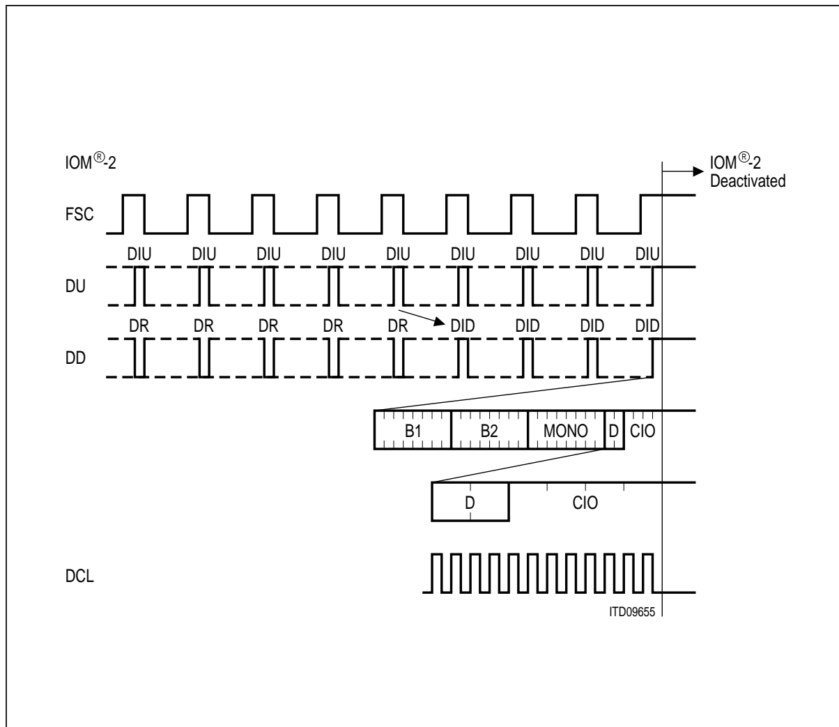
Figure 89 Deactivation of the IOM ® Interface
