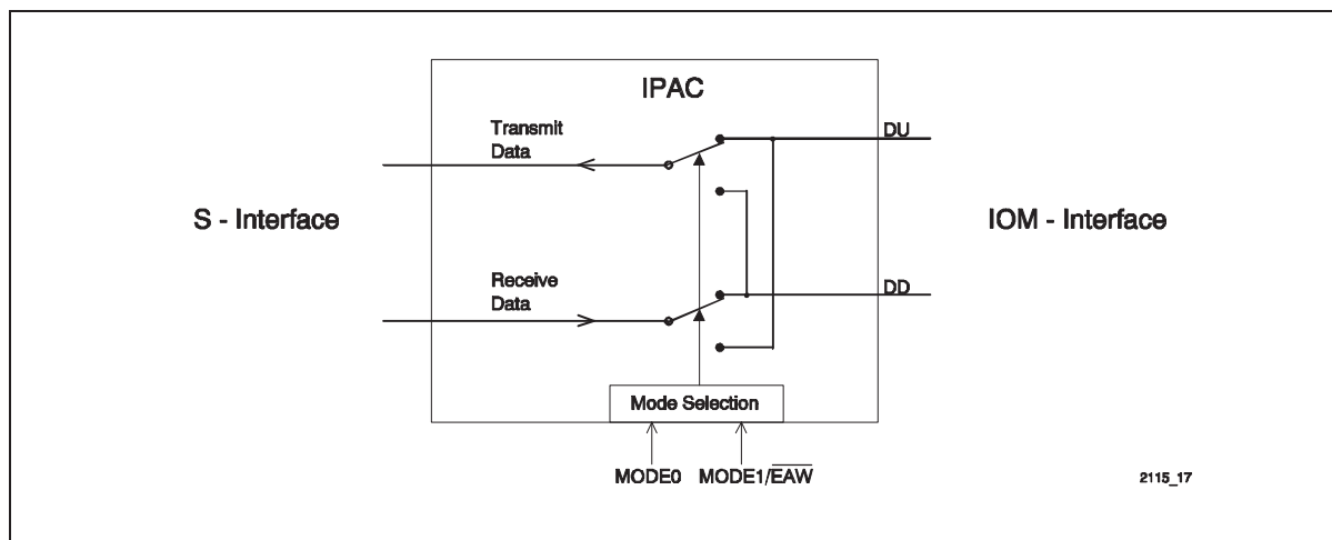
Figure 23 Data path switching
