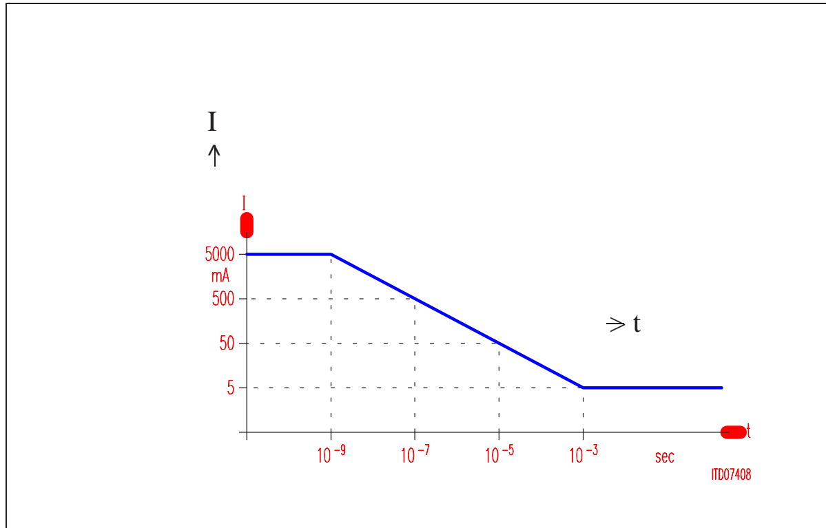
Figure 99 Maximum Line Input Current
