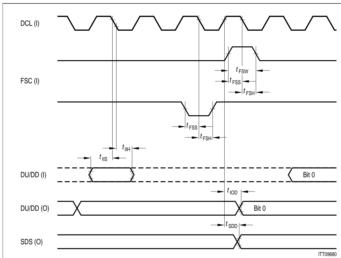
Figure 110 IOM® Timing (LT-S, LT-T mode)
