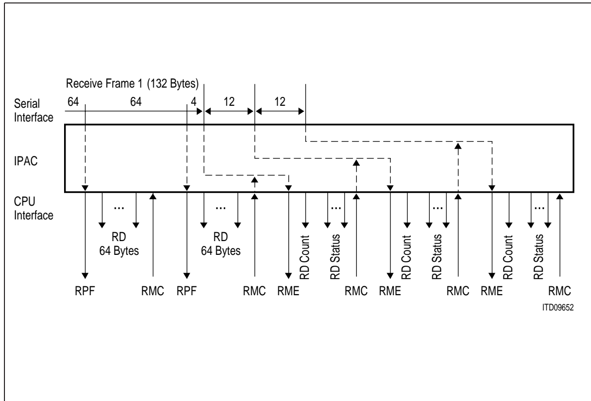
Figure 84 Interrupt Driven Reception Sequence Example
