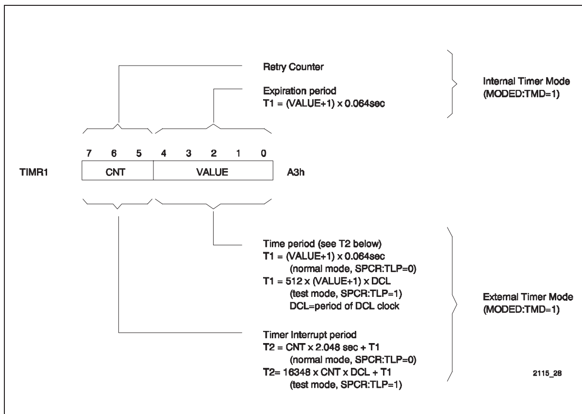
Figure 49 Timer 1 Register
