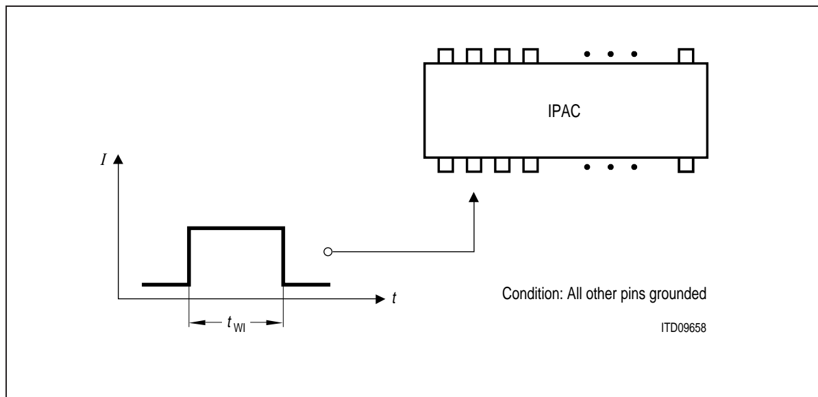
Figure 98 Test Condition for Maximum Input Current
