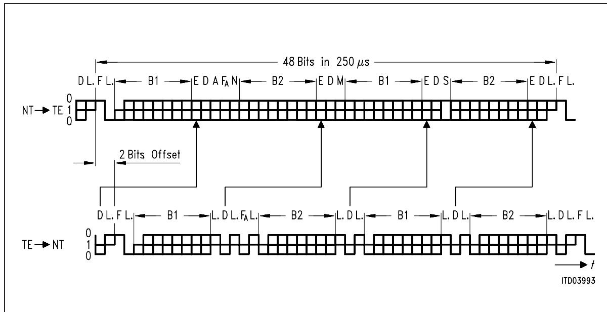
Figure 25 Frame Structure at Reference Points S and T (ITU I.430)
