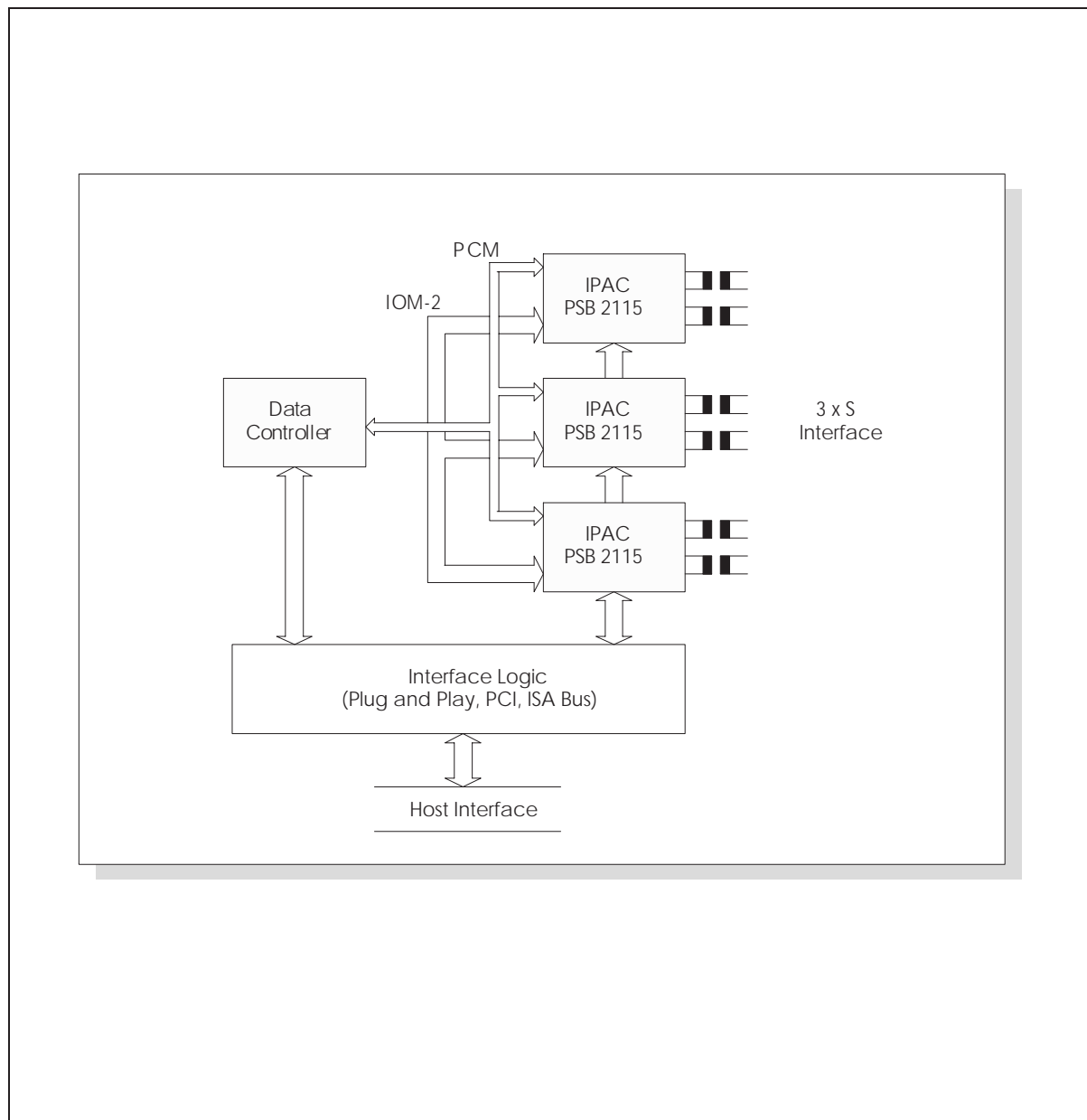
Figure 8 Multiline PC-Adapter
