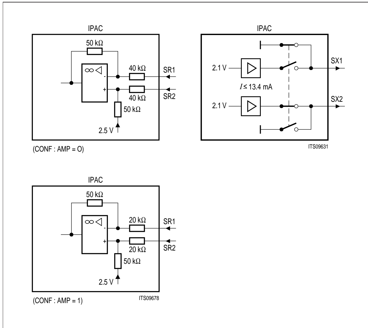
Figure 28 Equivalent Internal Circuits of Receiver and Transmitter Stages
