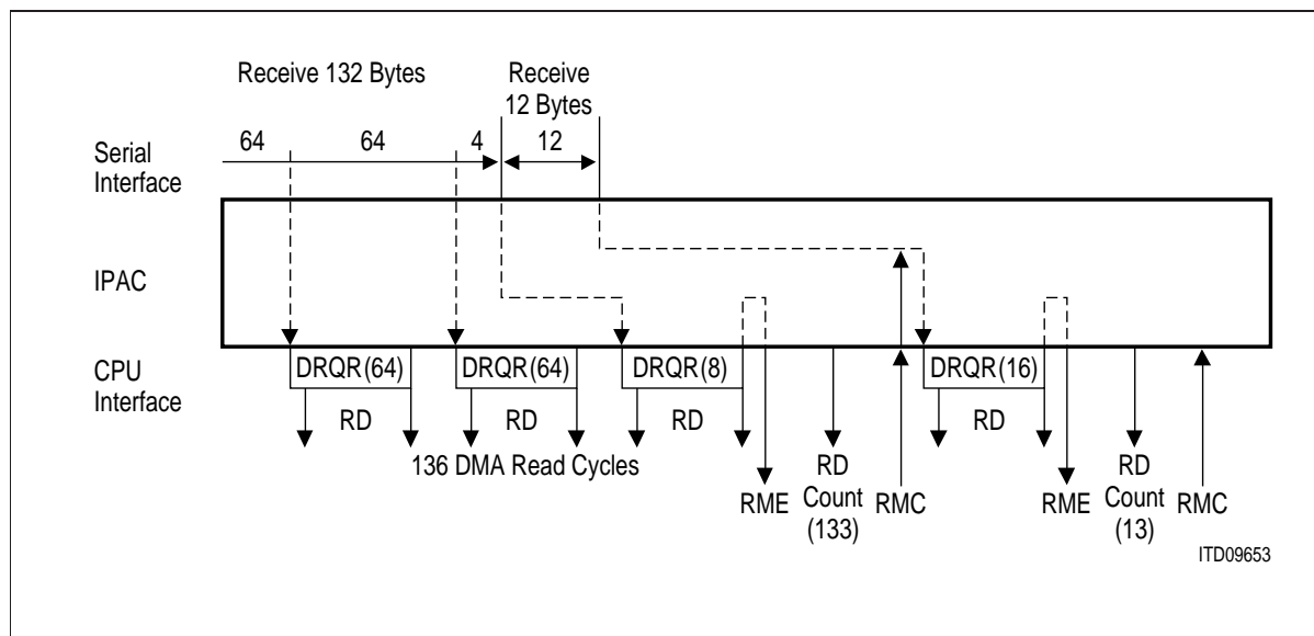
Figure 85 DMA Driven Reception Sequence Example
