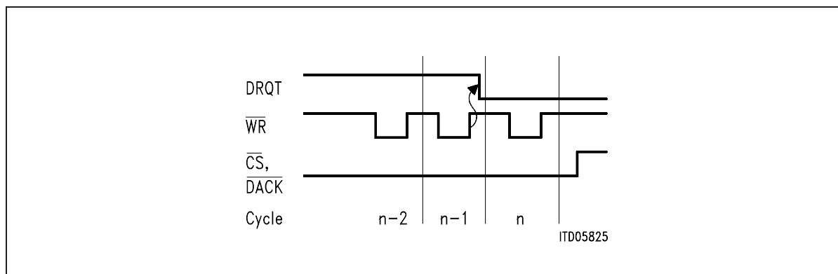
Figure 41 Timing Diagram for DMA-Transfers (fast) Transmit ( n < 64 , remainder of a long message or n = k \times 64 )
