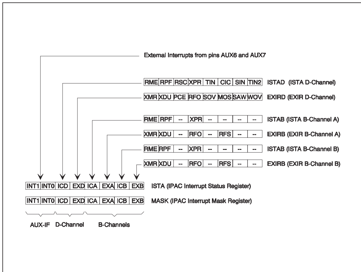
Figure 40 IPAC Interrupt Status Registers
