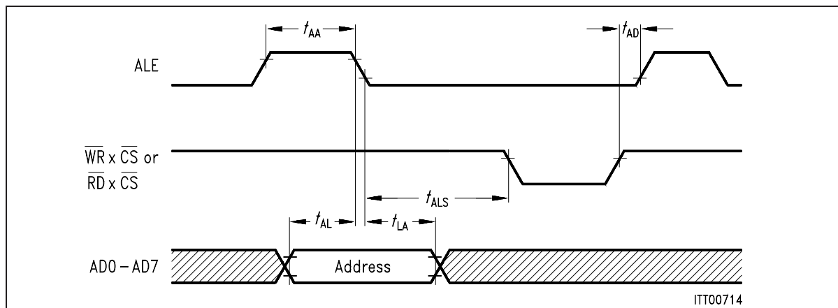
Figure 104 Multiplexed Address Timing
