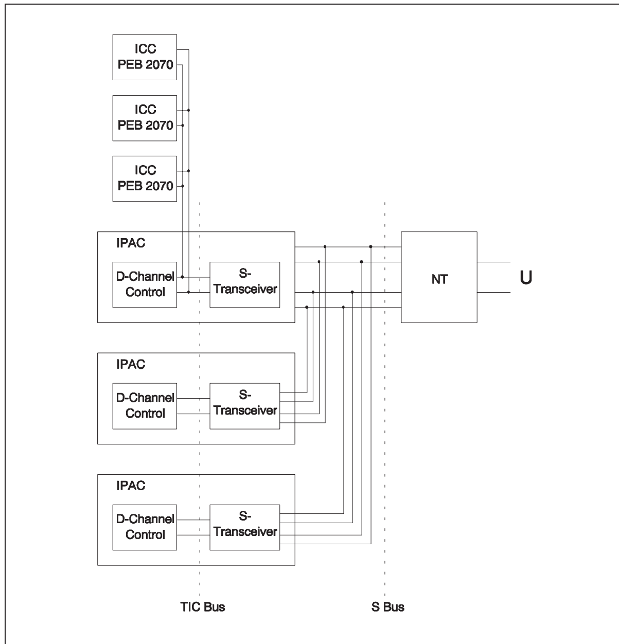
Figure 20 D-Channel Access Control on TIC Bus and S Bus
