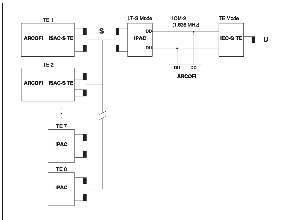
Figure 22 Intelligent NT-Configuration for IOM ® -2 Channel Switching
