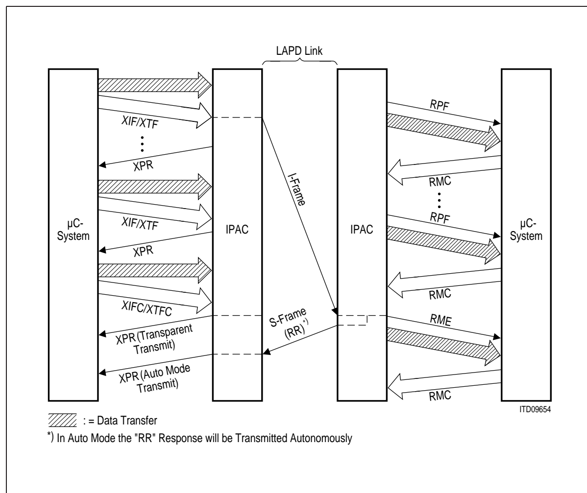
Figure 87 Transmission of an I Frame in the D Channel (Subscriber to Exchange)
