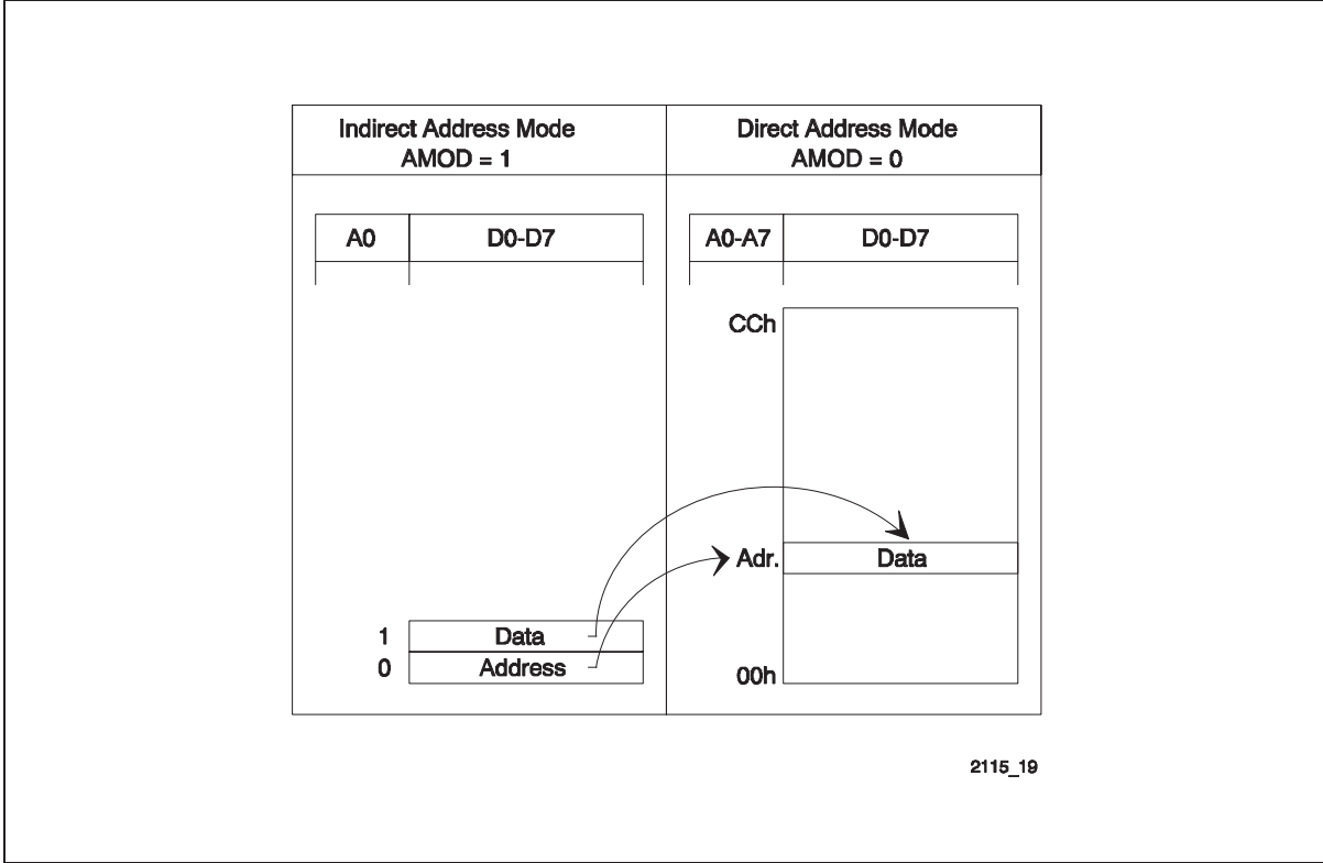
Figure 39 Indirect register address mode
