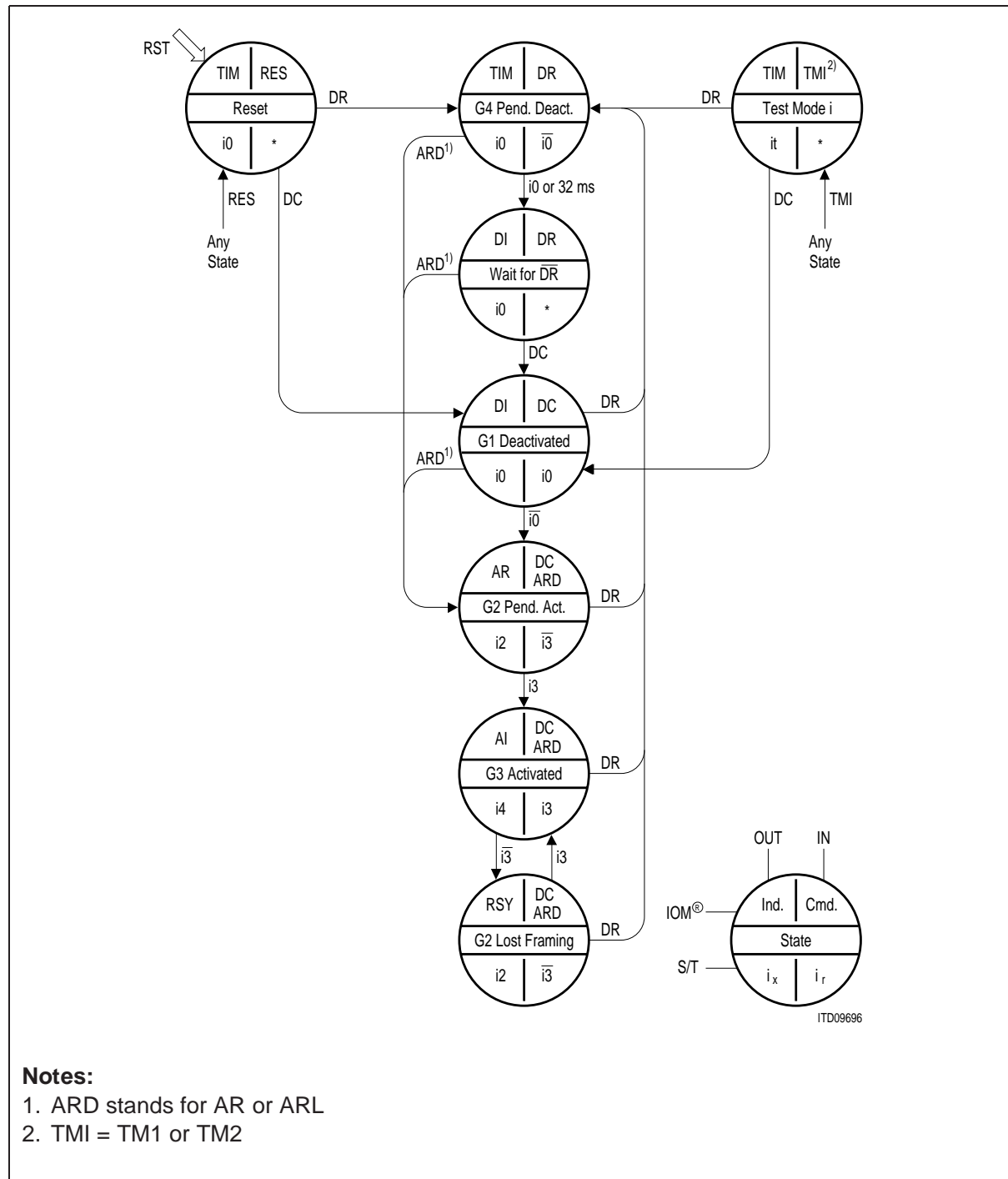
Figure 119 State Transition Diagram in LT-S Mode
