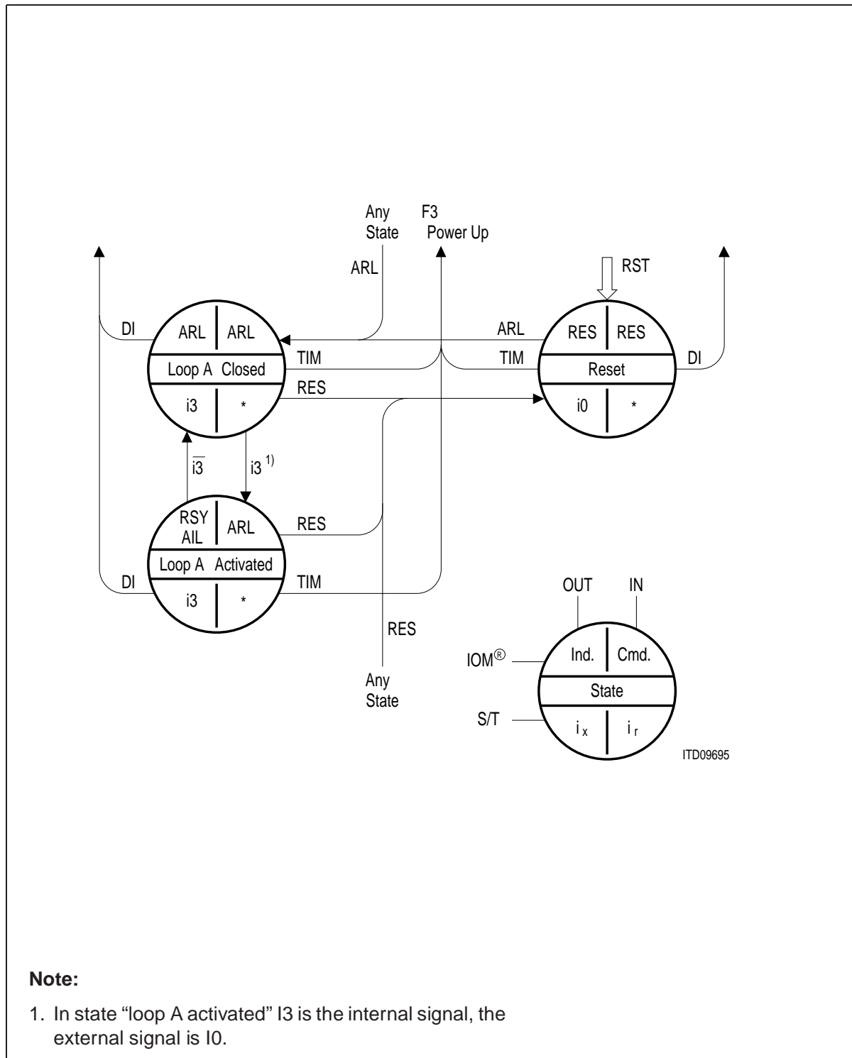
Figure 93 State Diagram of the TE/LT-T Modes, Unconditional Transitions
