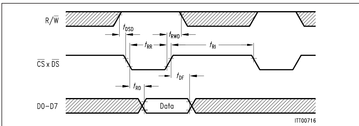
Figure 106 Microprocessor Read Timing
