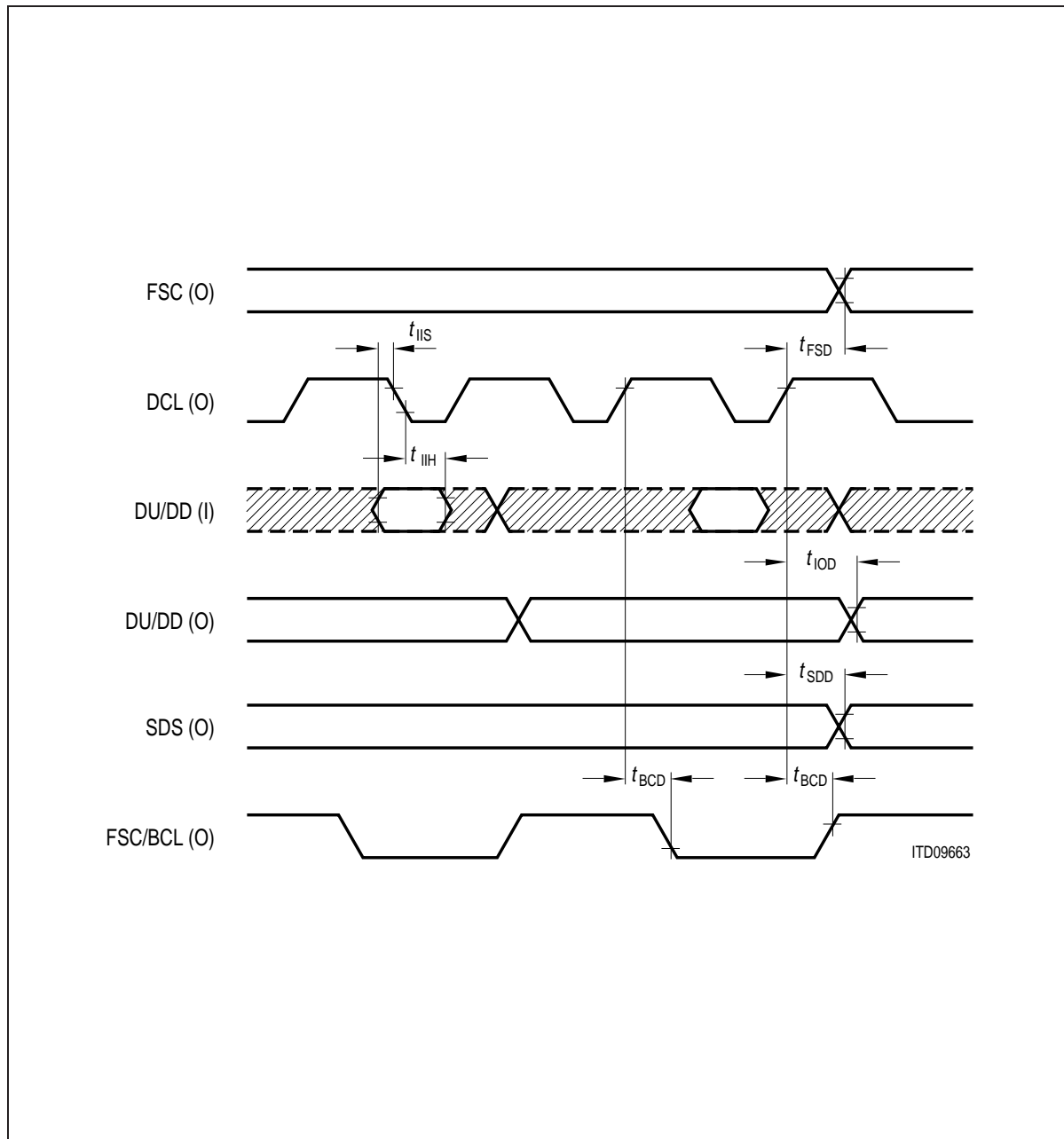
Figure 109 IOM® Timing (TE mode)
