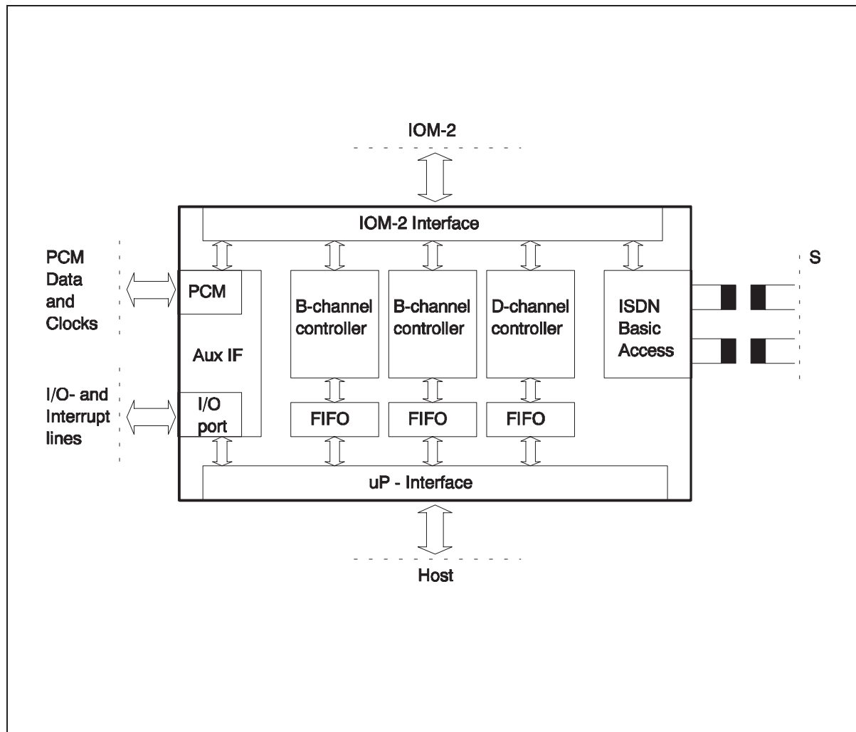
Figure 3 Block Diagram
