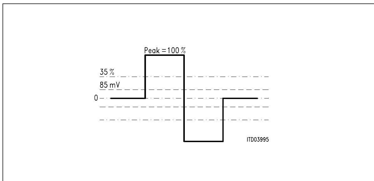
Figure 32 Receiver Thresholds
