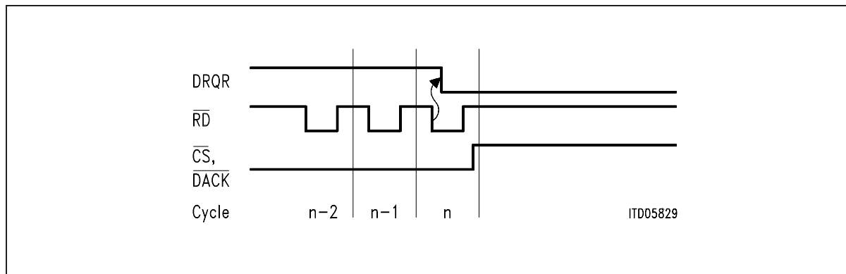
Figure 45 Timing Diagram for DMA-Transfers (slow or fast) Receive ( n = 4, 8, 16 or 32 )
