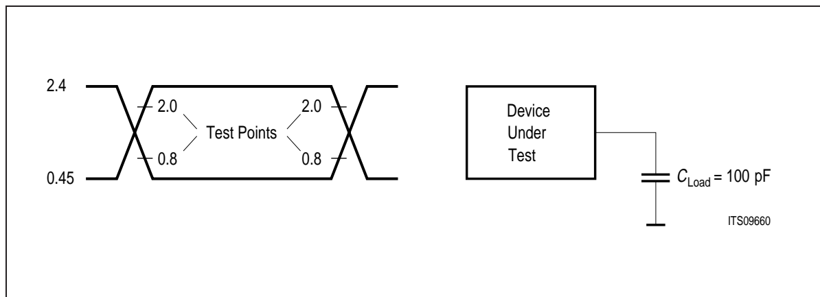
Figure 101 Input/Output Waveform for AC Tests
