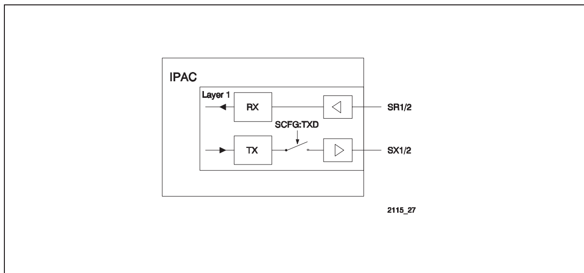
Figure 33 Disabling of S/T Transmitter
