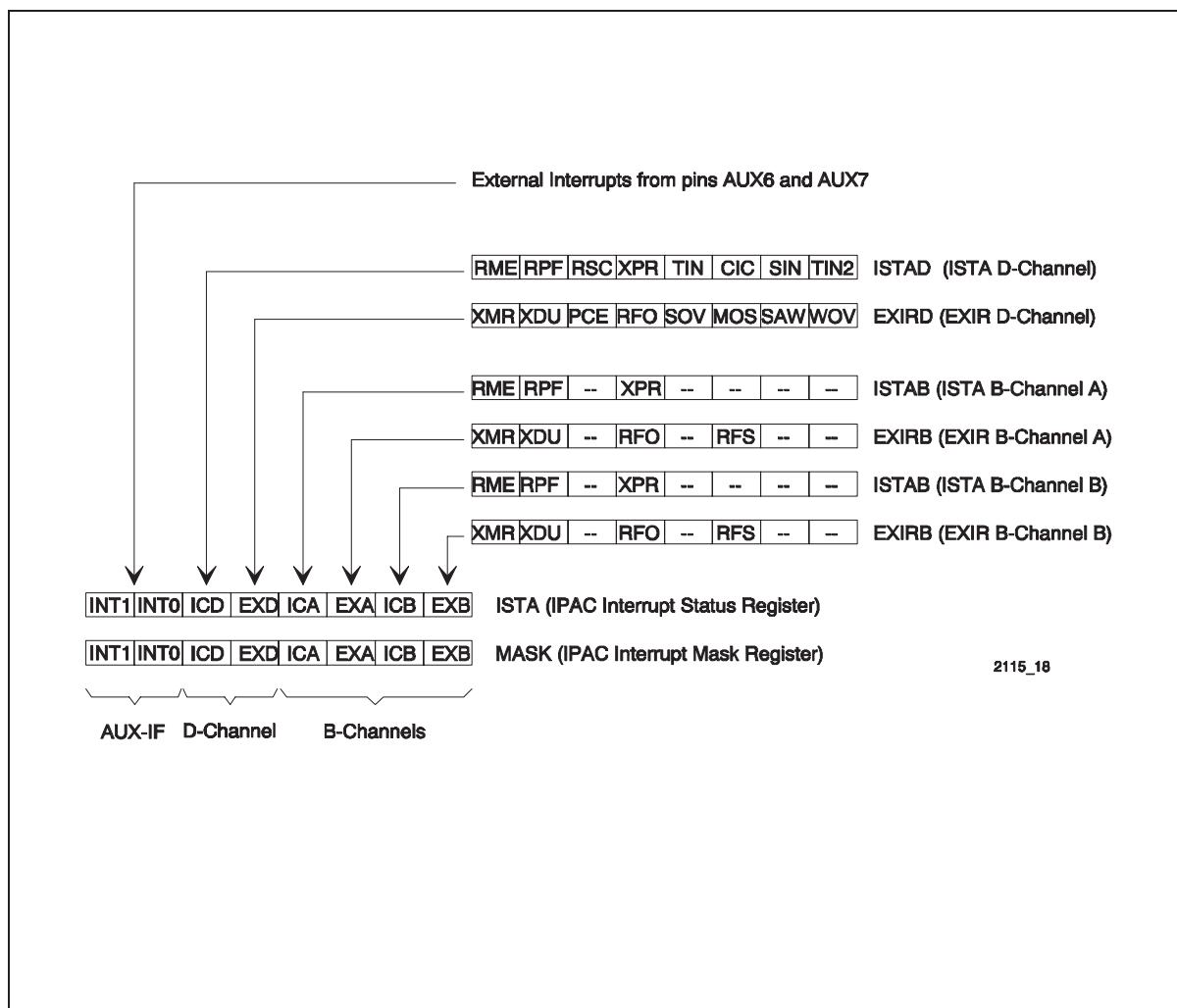
Figure 77 IPAC Interrupt Status Registers
