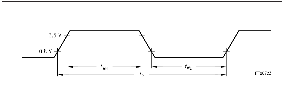
Figure 114 Definition of Clock Period and Width
