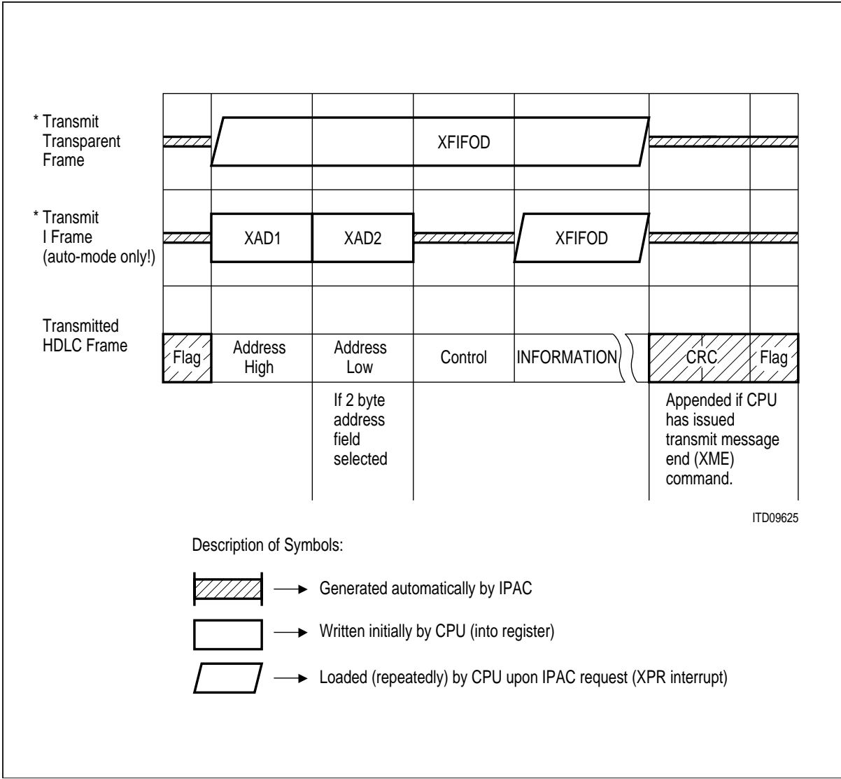
Figure 86 Transmit Data Flow
