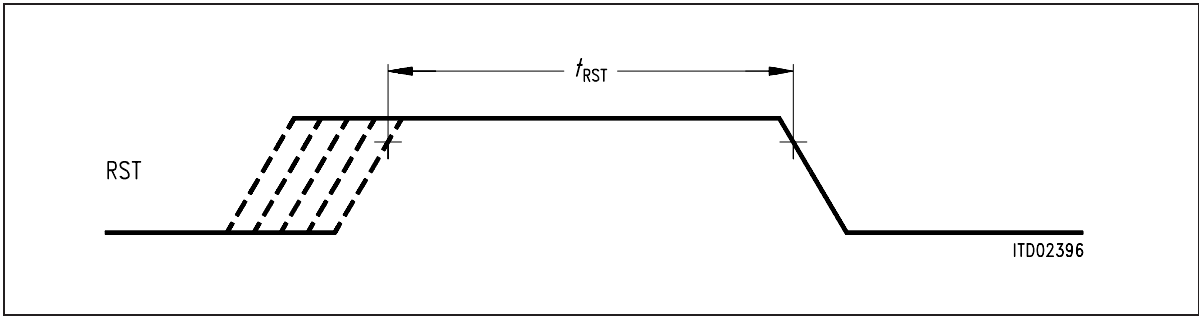
Figure 116 Reset Signal
