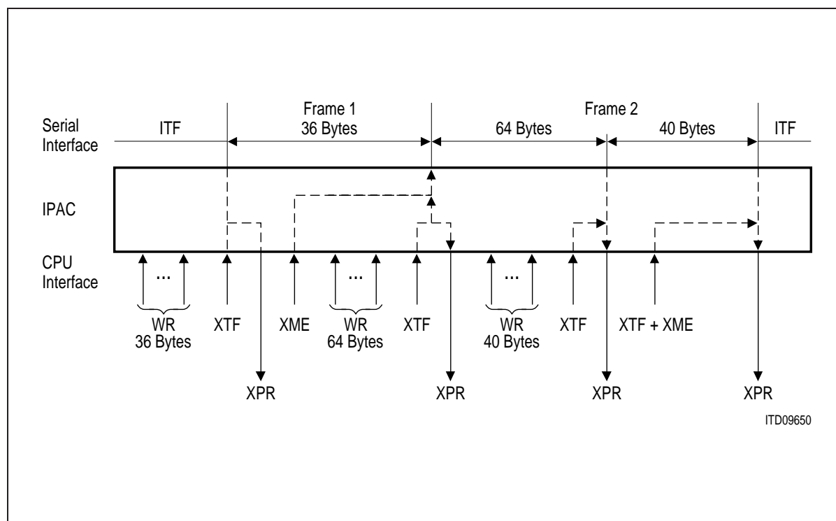
Figure 82 Continuous Frames Transmission Sequence Example
