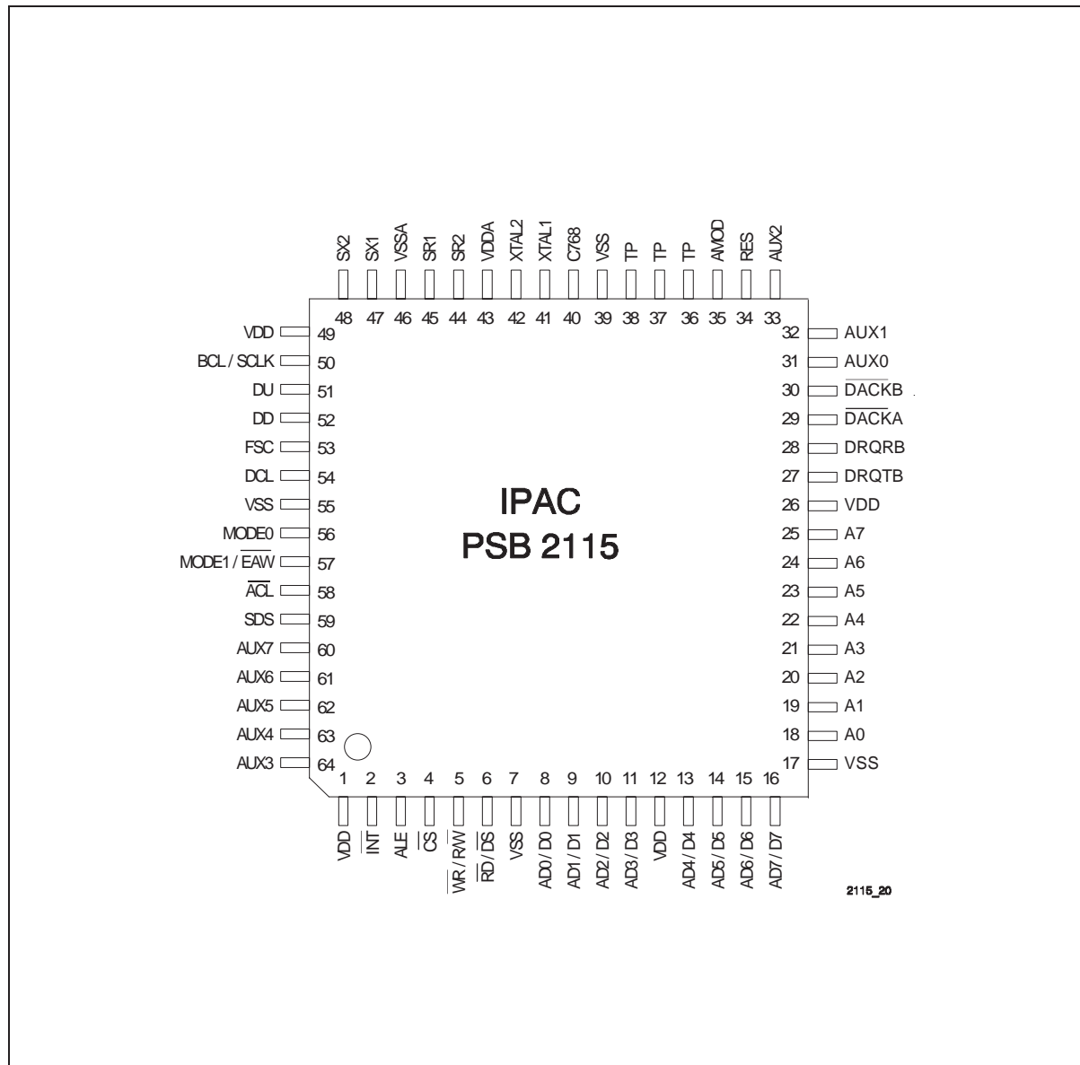
Figure 2 Pin Configuration
