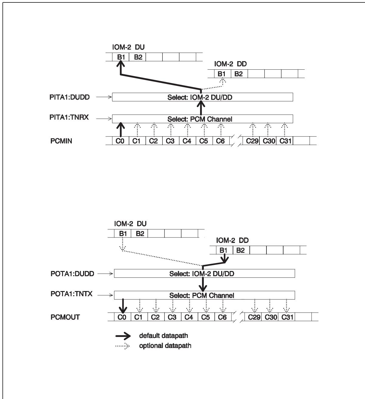
Figure 75 Switching of PCM timeslots on IOM-2 Channel B1
