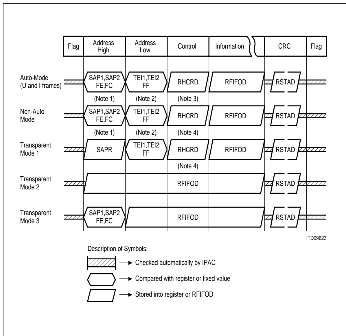
Figure 88 Receive Data Flow
