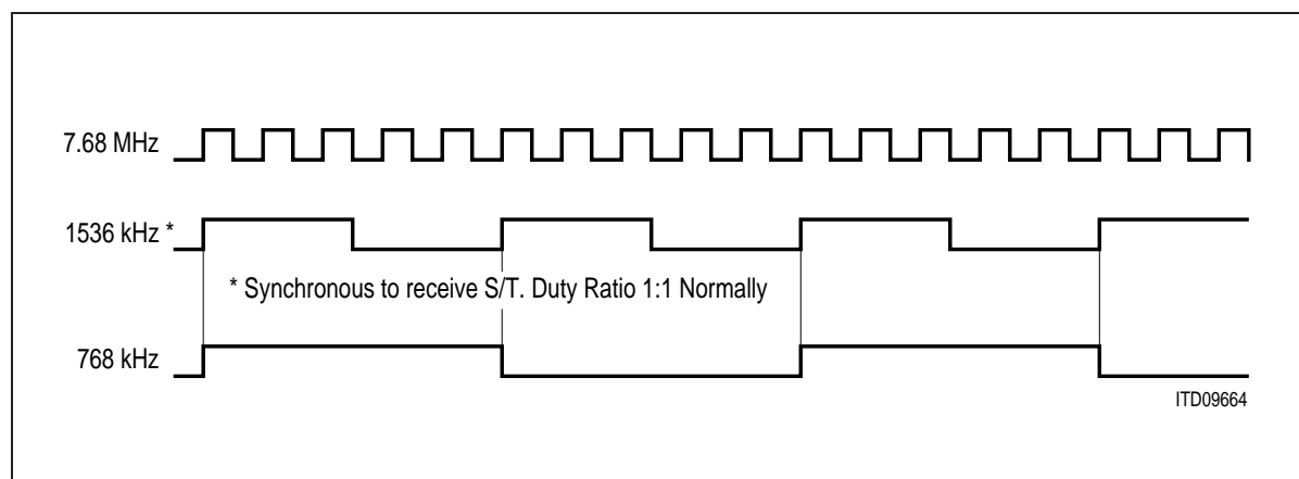
Figure 113 Phase Relationships of IPAC Clock Signals
