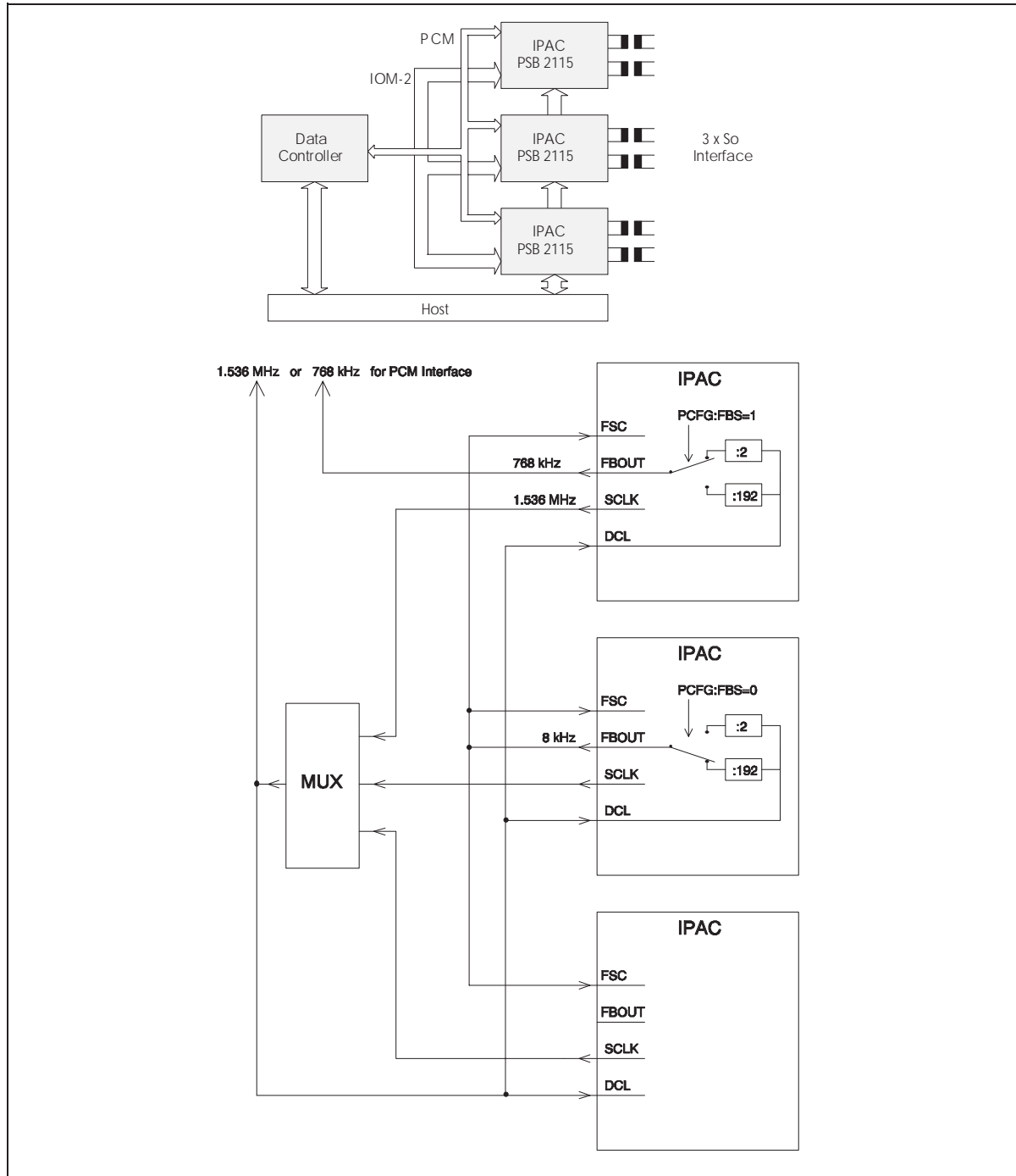
Figure 74 Multiline application
