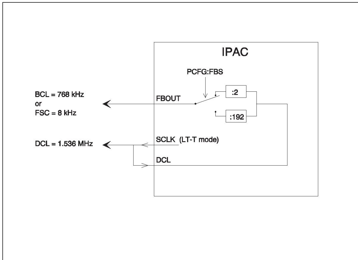
Figure 73 Generation of FSC and BCL in LT-T mode
