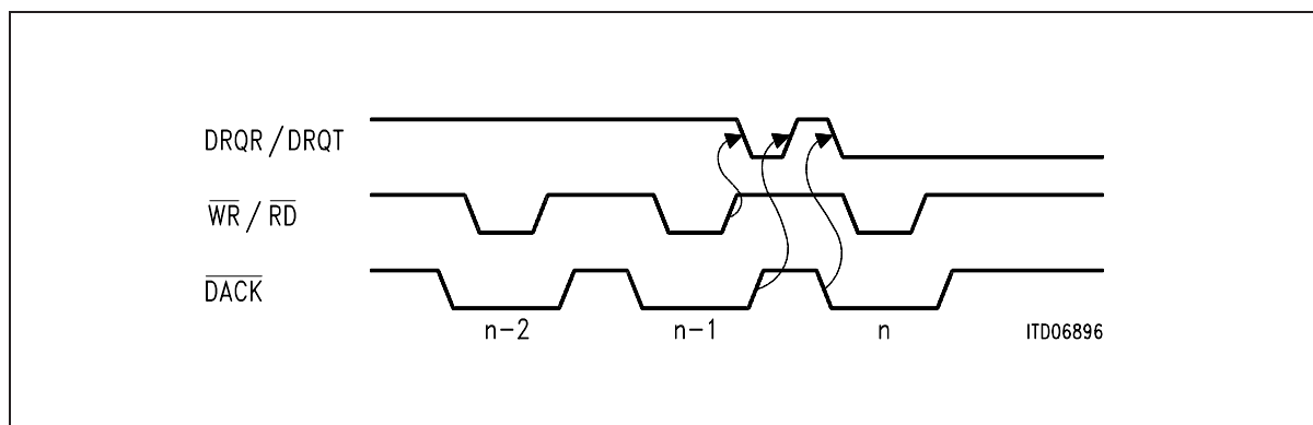
Figure 46 DMA-Transfers with Pulsed \overline{DACK} (read or write)
