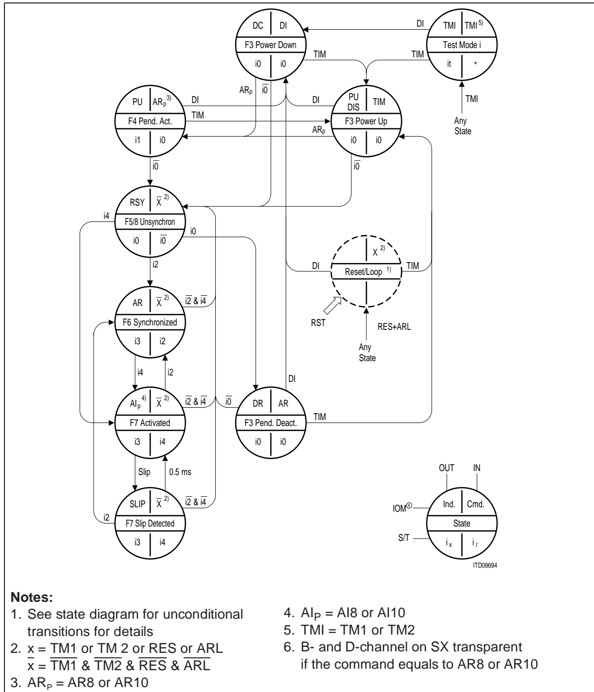
Figure 117 State Transition Diagram in TE/LT-T Modes
