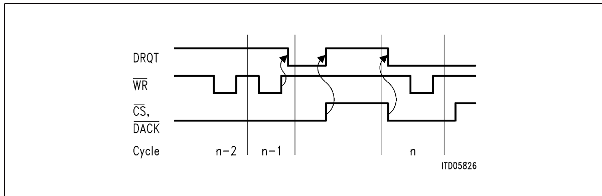
Figure 42 Timing Diagram for DMA-Transfers (slow) Transmit ( n < 64 , remainder of a long message or n = k \times 64 )
