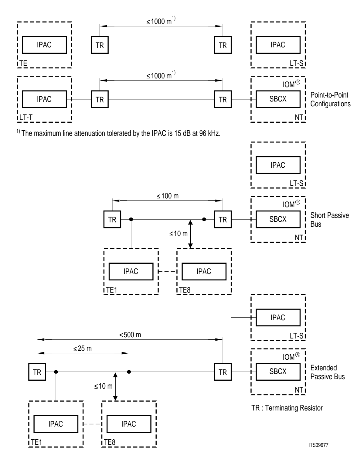
Figure 26 Wiring Configurations in User Premises
