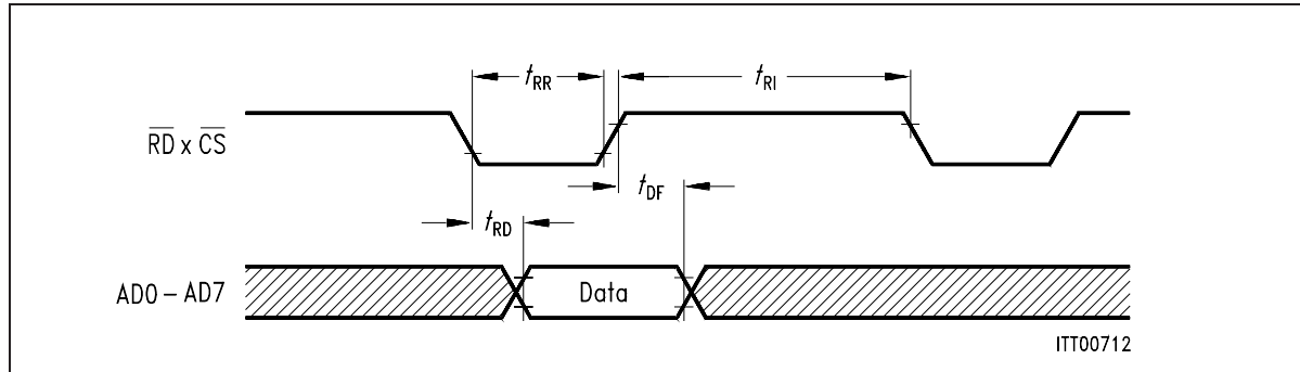
Figure 102 Microprocessor Read Cycle
