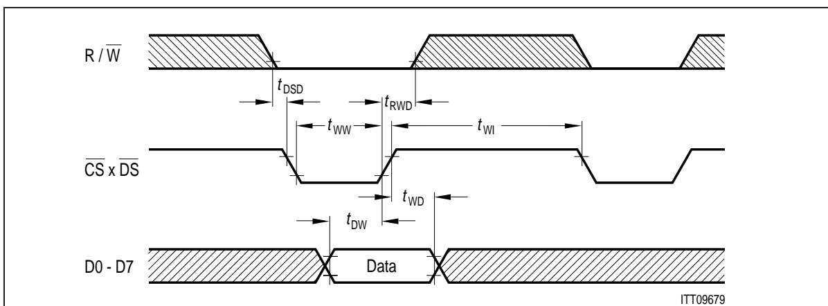
Figure 107 Microprocessor Write Cycle
