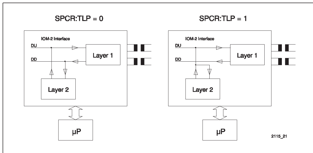
Figure 38 Layer 2 Test Loops
