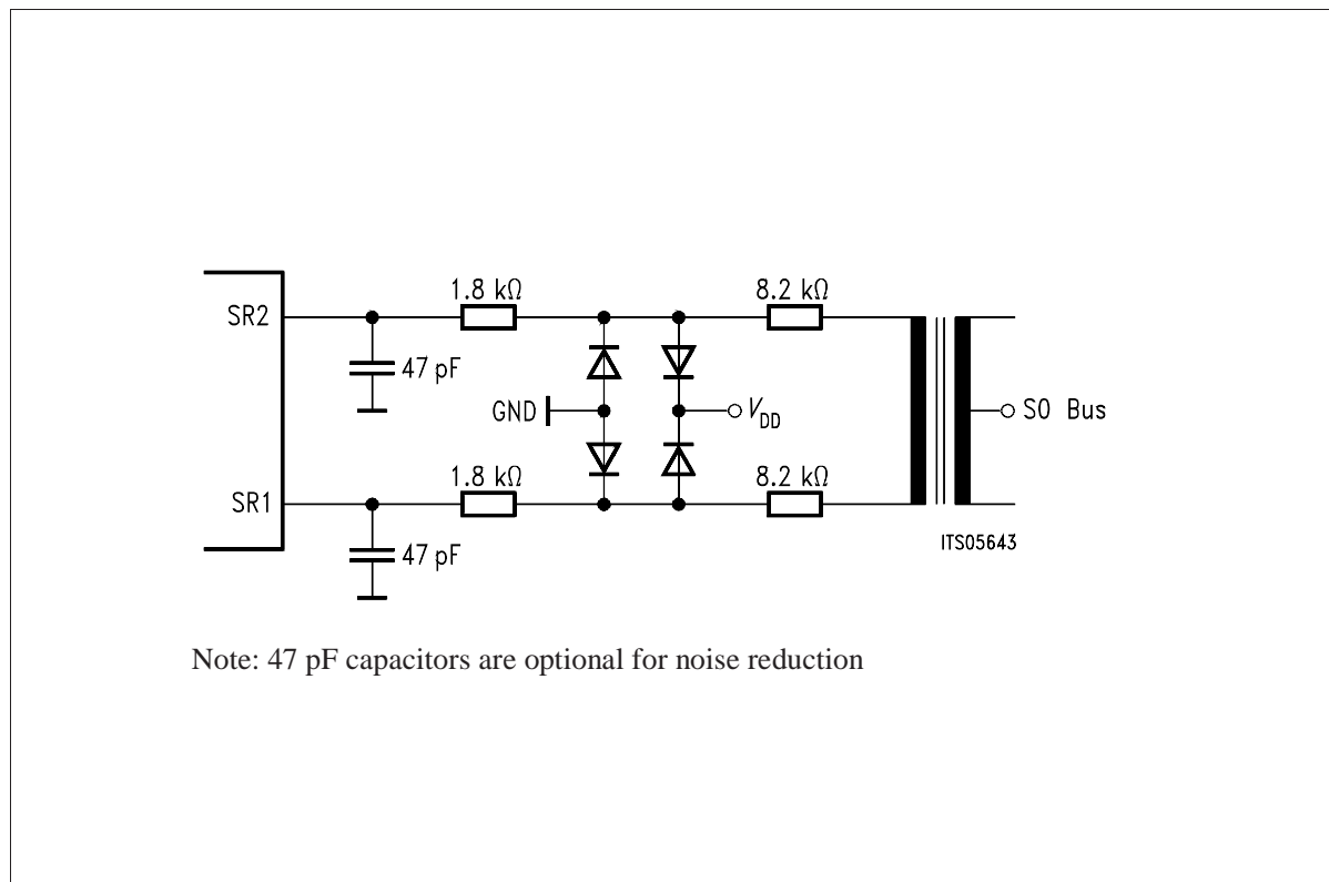
Figure 30 External Circuitry for Symmetrical Receivers
