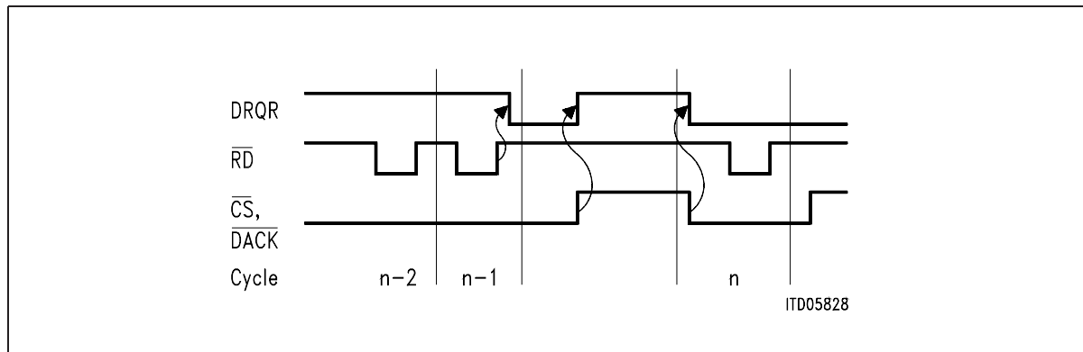
Figure 44 Timing Diagram for DMA-Transfers (slow) Receive ( n = k \times 64 )
