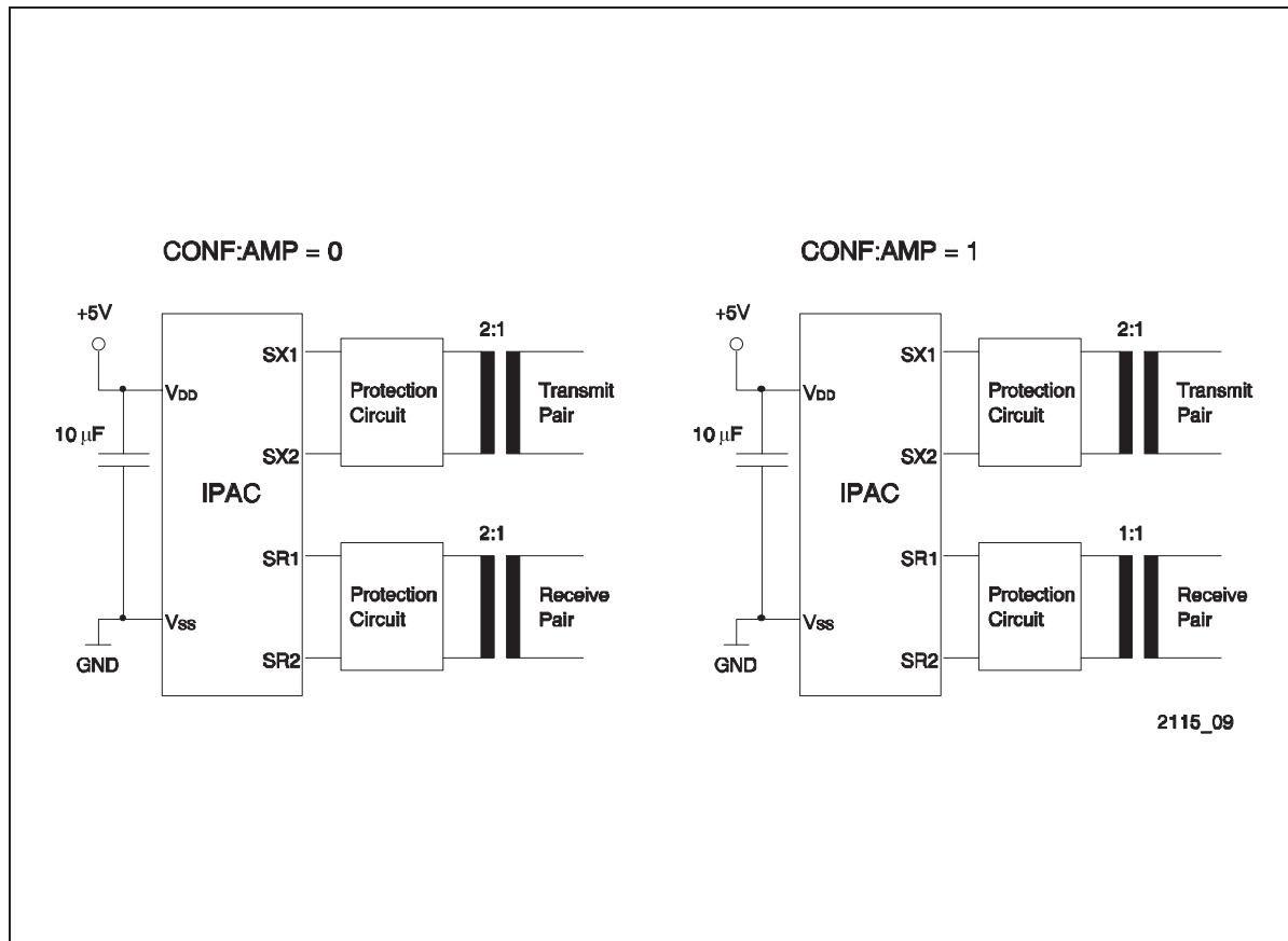
Figure 27 Connection of the Line Transformers and Power Supply to the IPAC
