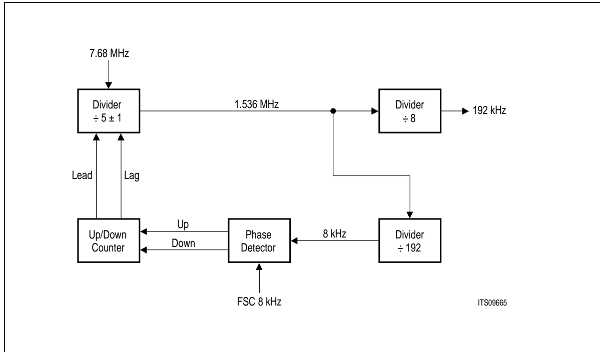
Figure 115 Block Diagram of XPLL
