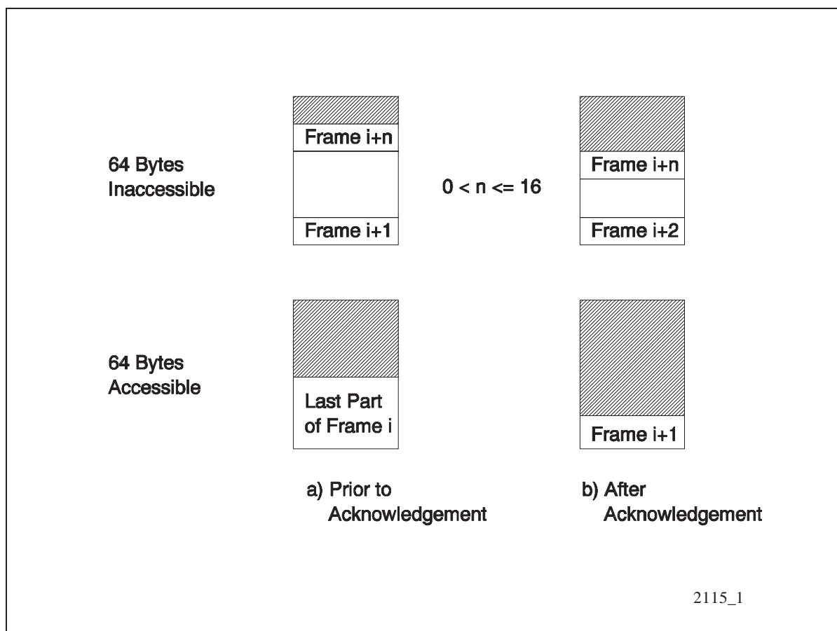
Figure 48 Configuration of RFIFOB (Short Frames)
