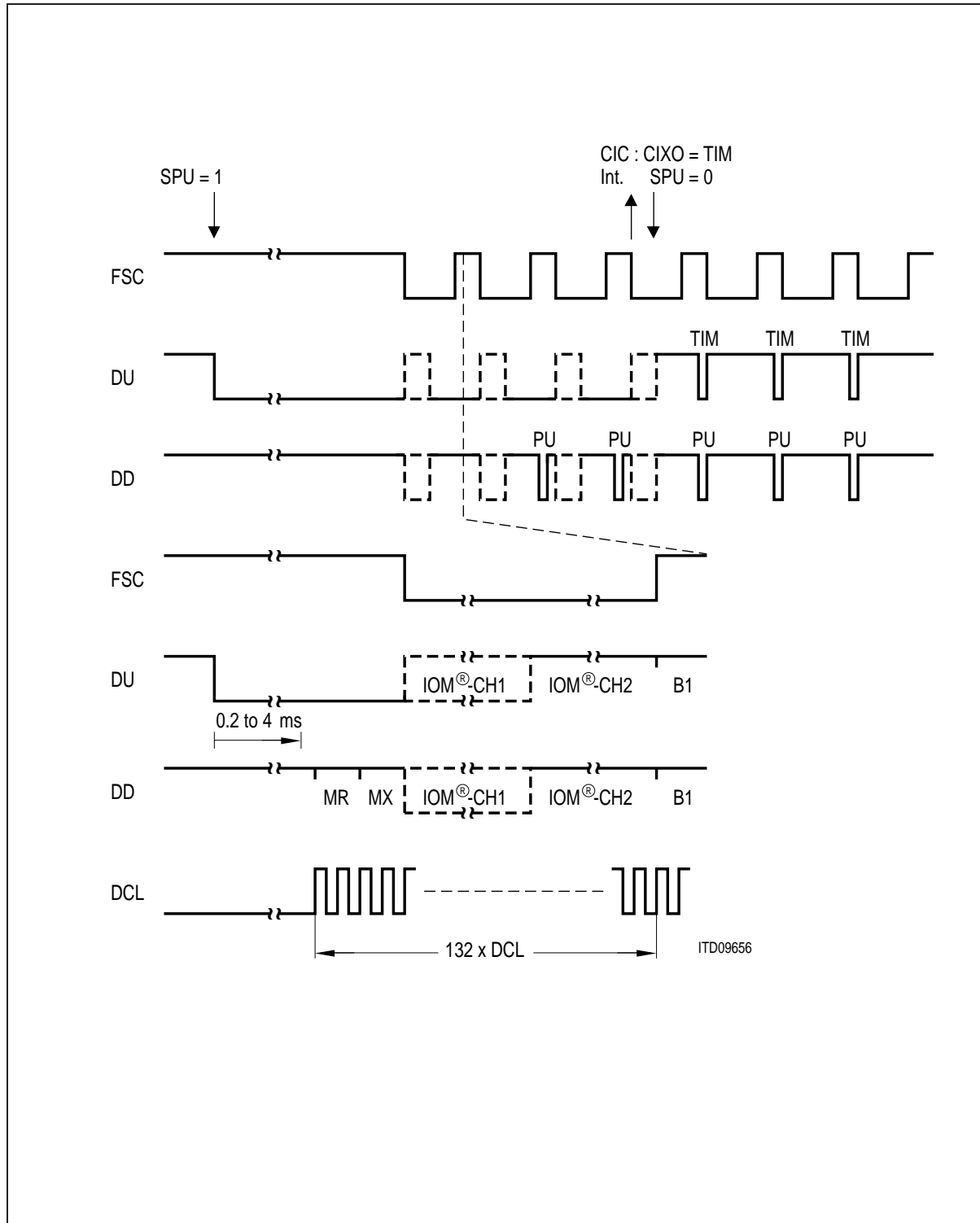
Figure 90 Activation of the IOM interface
