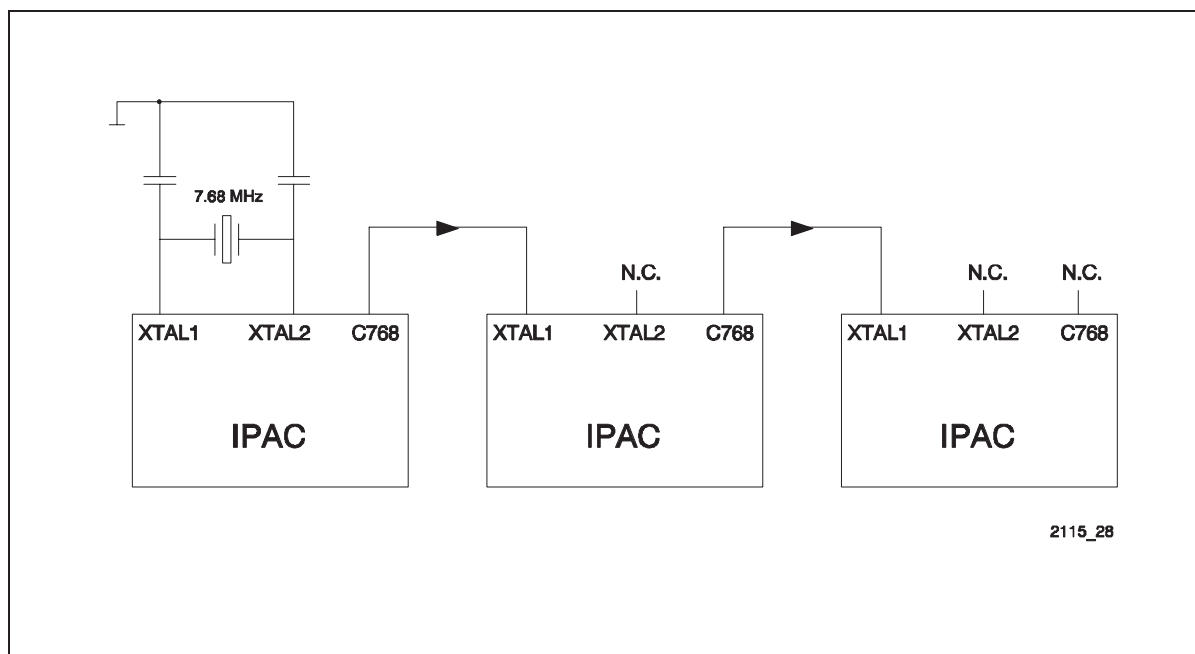
Figure 76 Buffered Oscillator Clock Output
