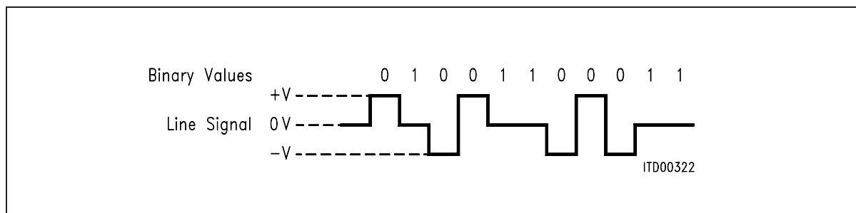
Figure 24 S/T -Interface Line Code (without code violation)
