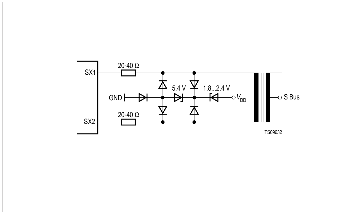
Figure 29 External Circuitry for Transmitters
