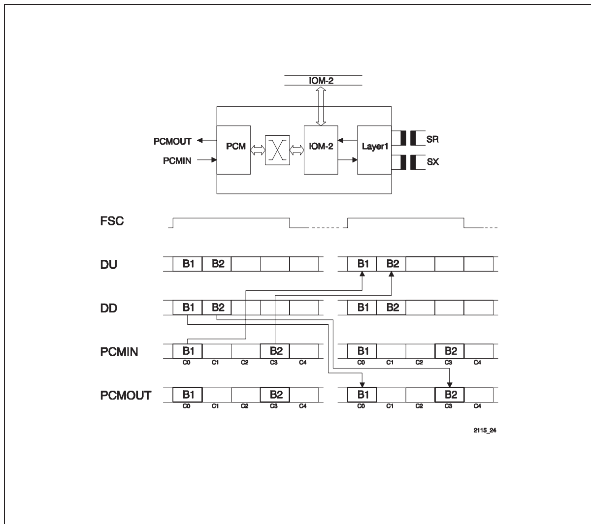
Figure 72 Switching Data between PCM and IOM-2
