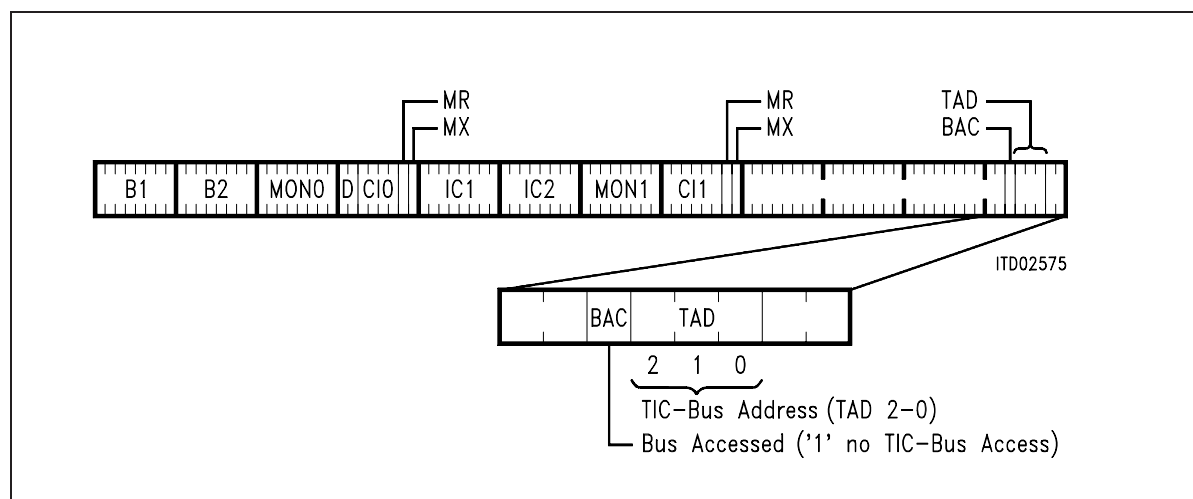
Figure 67 Structure of Last Octet of Ch2 on DU
