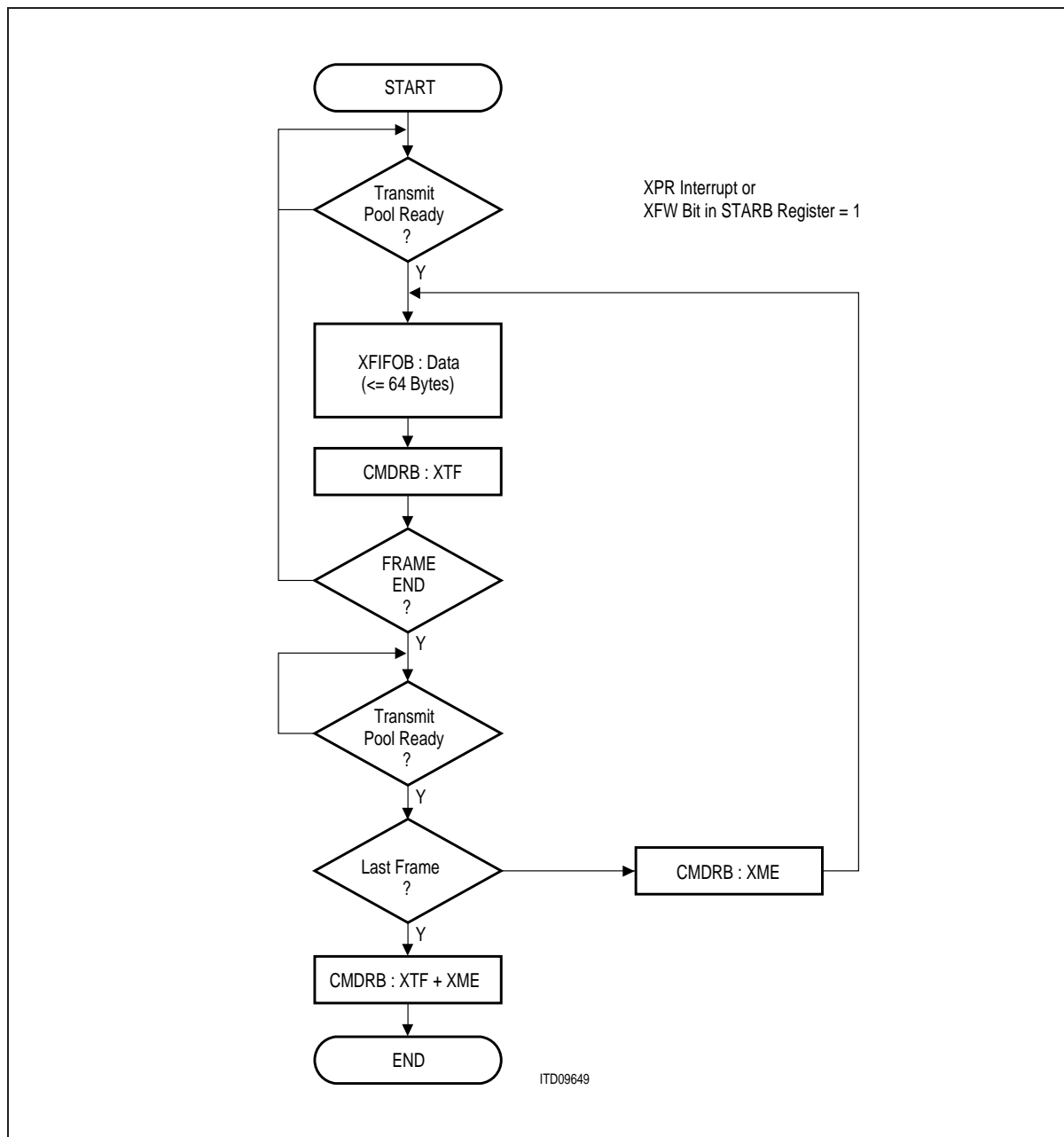
Figure 81 Continuous Frames Transmission (Flow Diagram)
