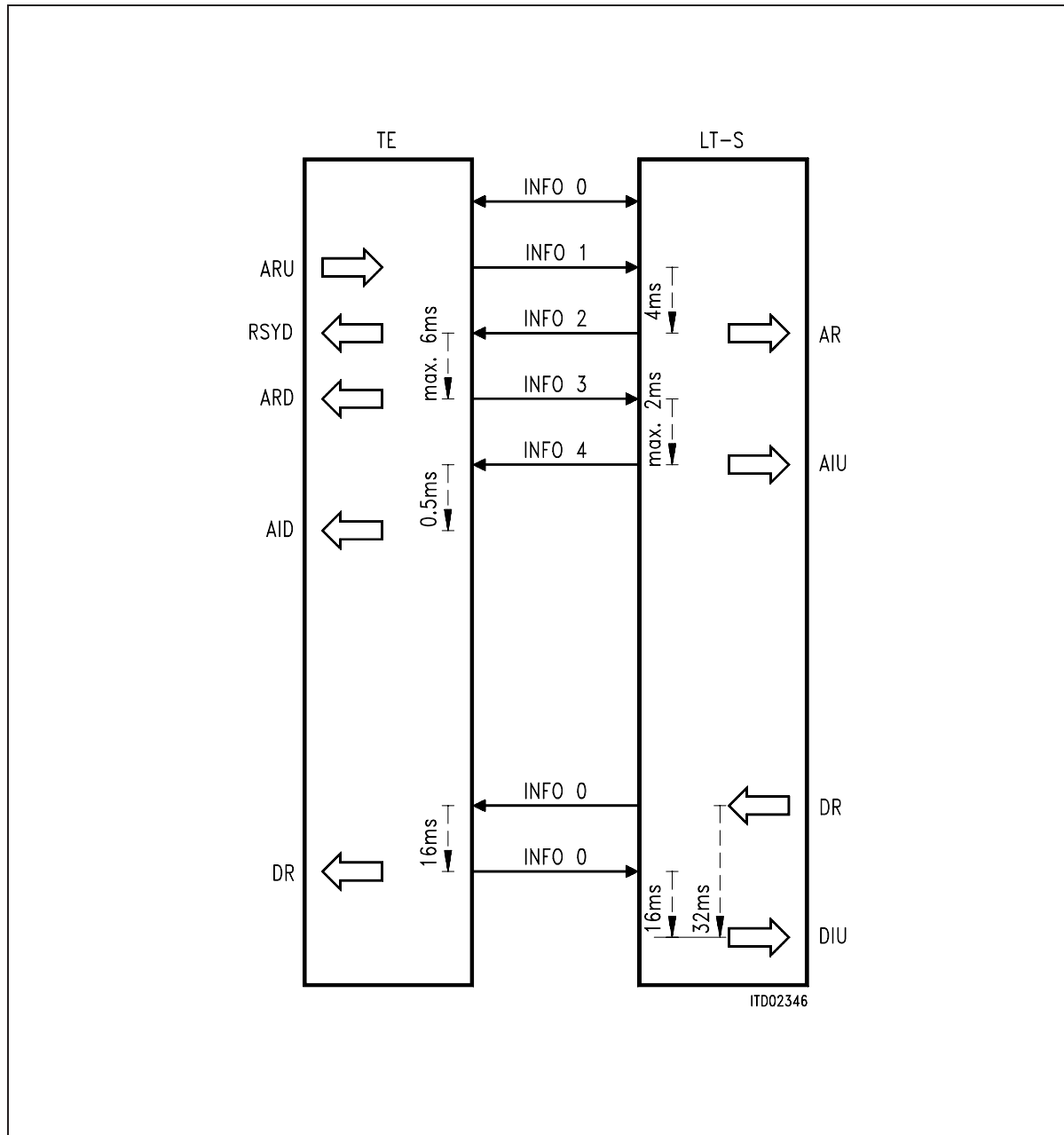
Figure 96 Example of Activation/Deactivation
