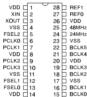
PLL52C59-14A
