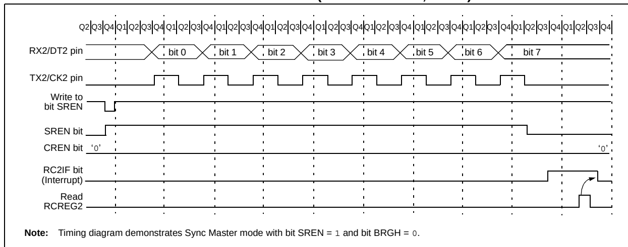
FIGURE 16-8: SYNCHRONOUS RECEPTION (MASTER MODE, SREN)
