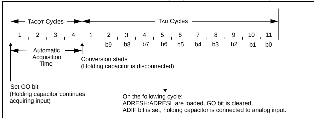
FIGURE 18-4: A/D CONVERSION TAD CYCLES (ACQT<2:0> = 010, TACQ = 4 TAD)
