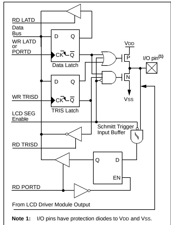
FIGURE 9-10: BLOCK DIAGRAM OF RD7:RD0 PINS
