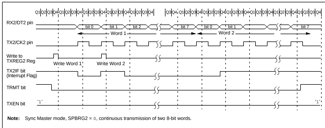
FIGURE 16-6: SYNCHRONOUS TRANSMISSION
