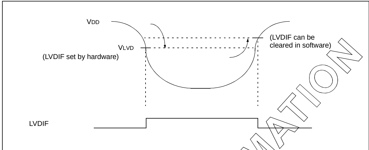
FIGURE 26-3: LOW-VOLTAGE DETECT CHARACTERISTICS
