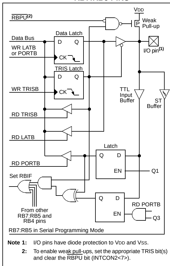
FIGURE 9-6: BLOCK DIAGRAM OF RB7:RB5 PINS
