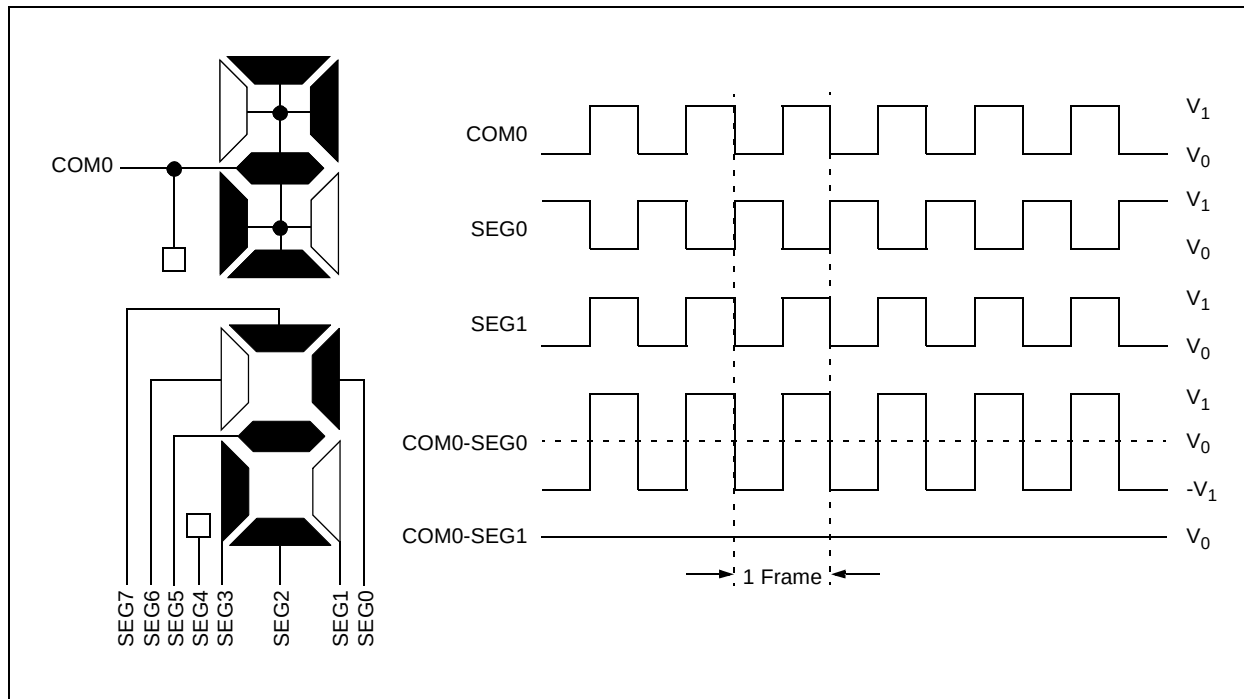
FIGURE 22-4: TYPE-A/TYPE-B WAVEFORMS IN STATIC DRIVE
