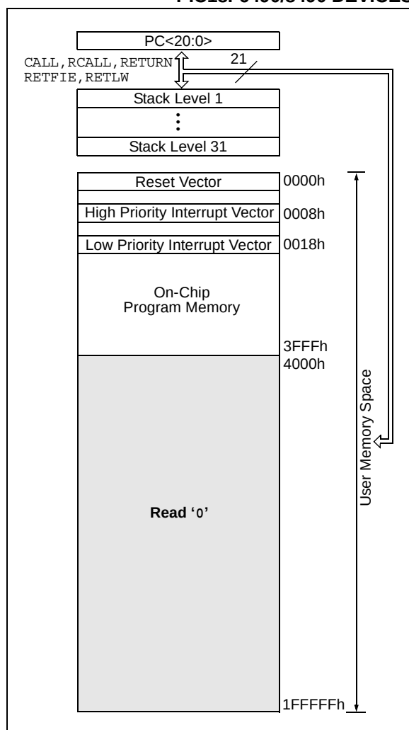
FIGURE 5-1: PROGRAM MEMORY MAP AND STACK FOR PIC18F6490/8490 DEVICES
