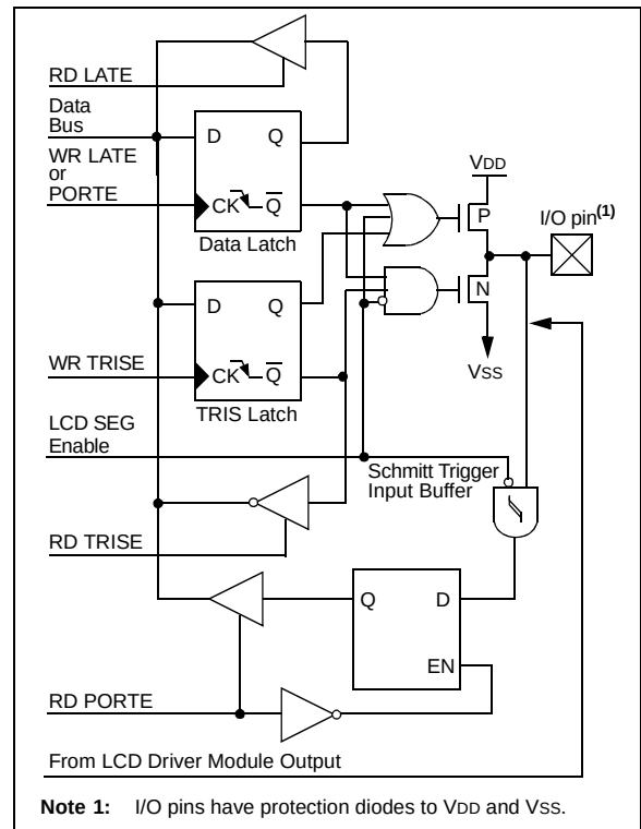
FIGURE 9-11: BLOCK DIAGRAM OF RE6:RE4 PINS
