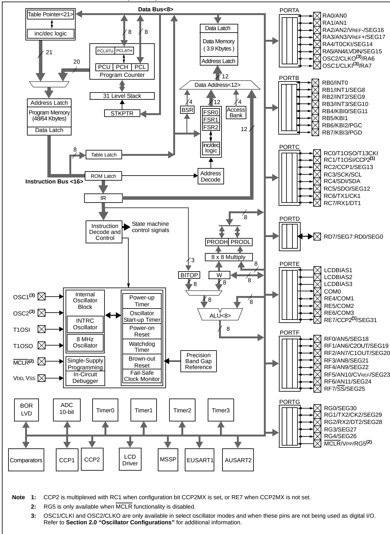
FIGURE 1-1: PIC18F6490 (64-PIN) BLOCK DIAGRAM
