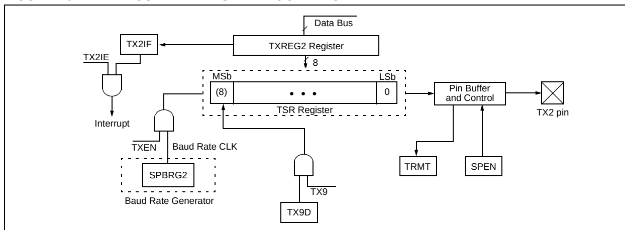
FIGURE 16-1: AUSART TRANSMIT BLOCK DIAGRAM
