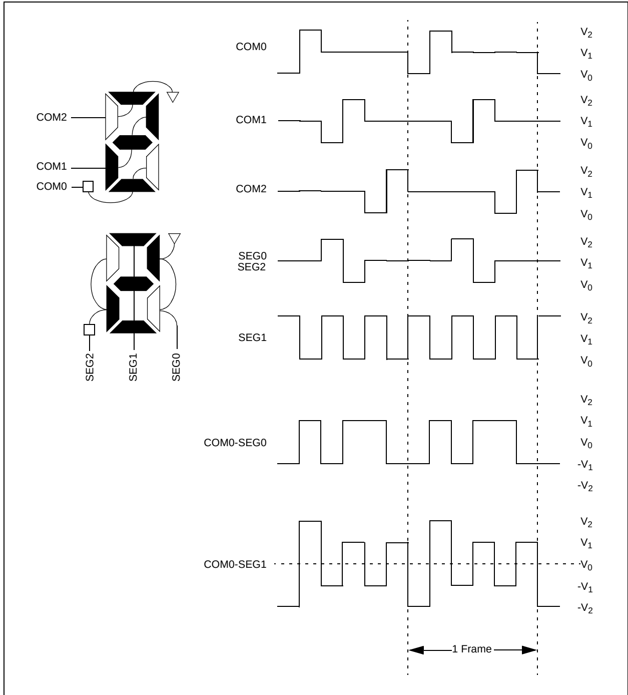
FIGURE 22-9: TYPE-A WAVEFORMS IN 1/3 MUX, 1/2 BIAS DRIVE
