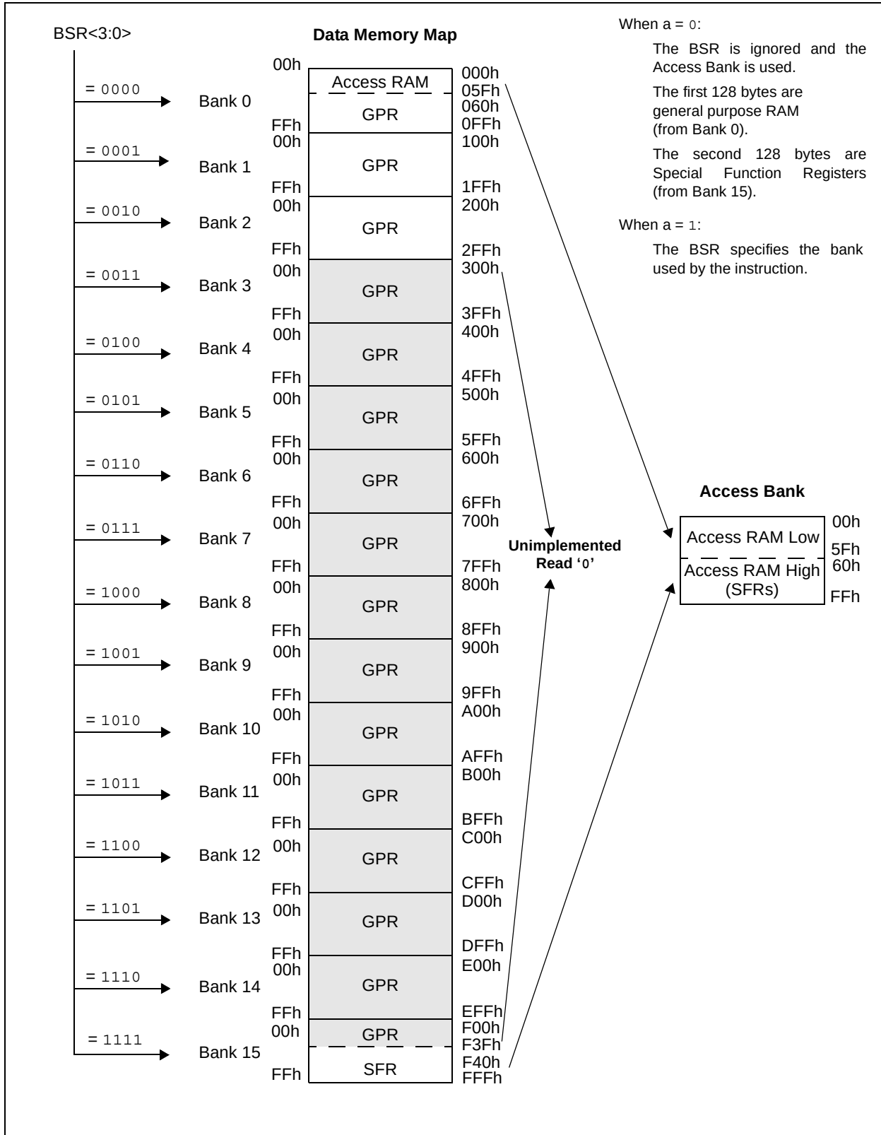
FIGURE 5-5: DATA MEMORY MAP FOR PIC18F6490/8490 DEVICES
