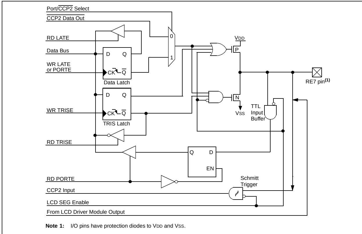
FIGURE 9-12: BLOCK DIAGRAM OF RE7/CCP2 PIN
