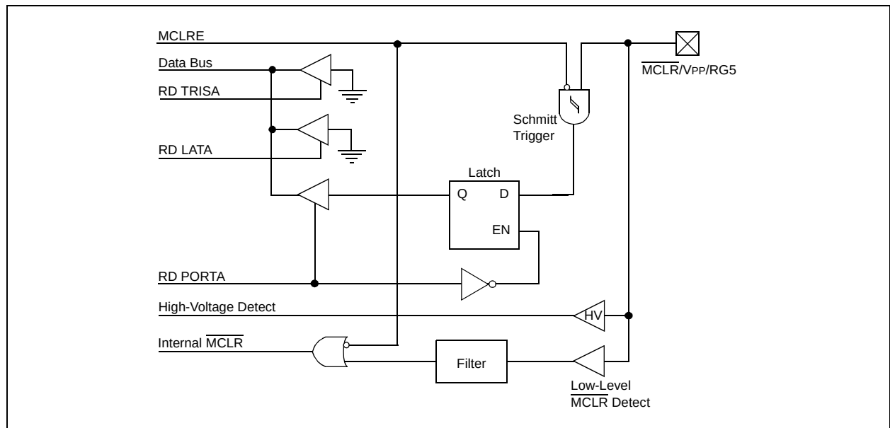
FIGURE 9-17: BLOCK DIAGRAM OF MCLR/VPP/RG5 PIN
