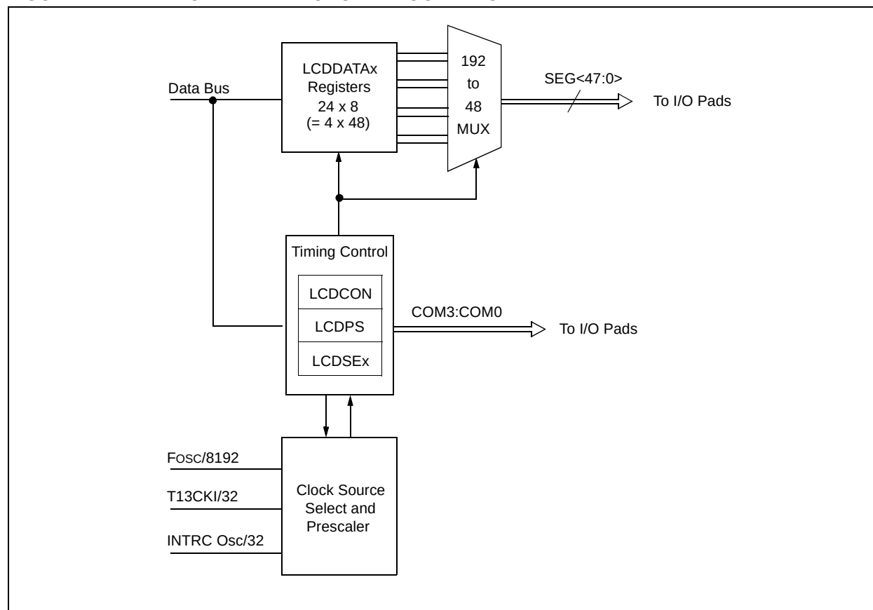
FIGURE 22-1: LCD DRIVER MODULE BLOCK DIAGRAM
