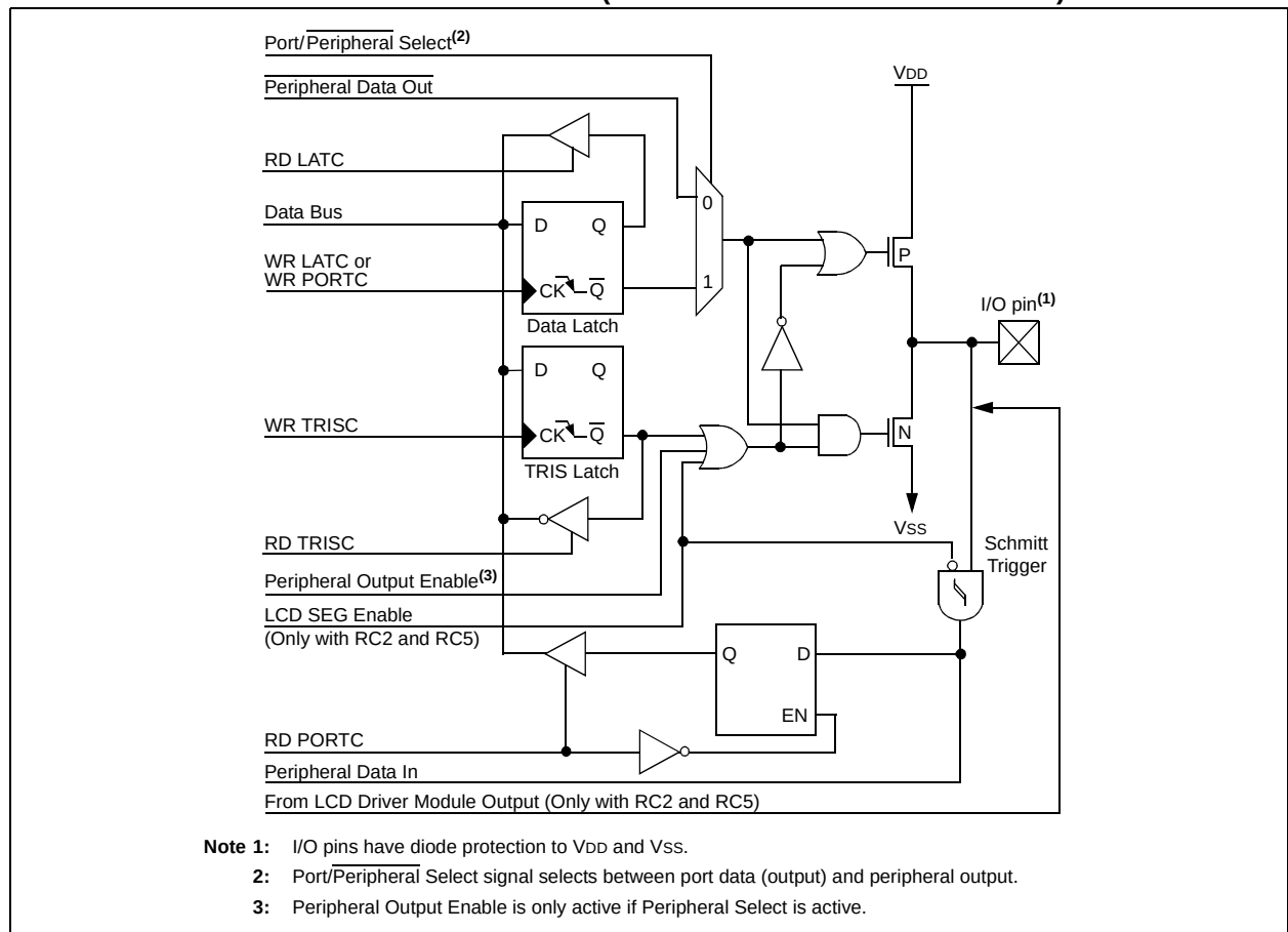
FIGURE 9-9: PORTC BLOCK DIAGRAM (PERIPHERAL OUTPUT OVERRIDE)
