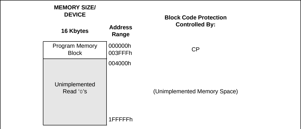
FIGURE 23-5: CODE-PROTECTED PROGRAM MEMORY FOR PIC18F6490/8490
