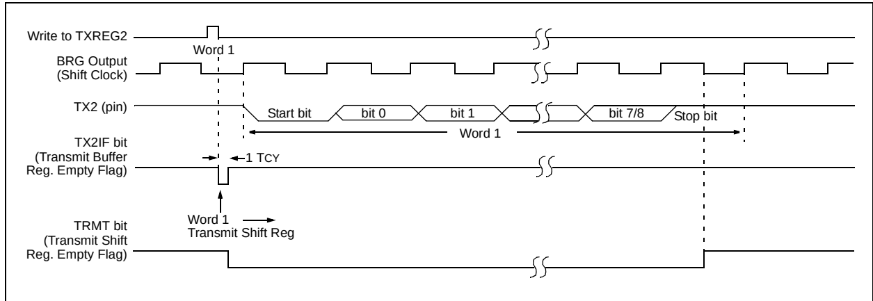
FIGURE 16-2: ASYNCHRONOUS TRANSMISSION
