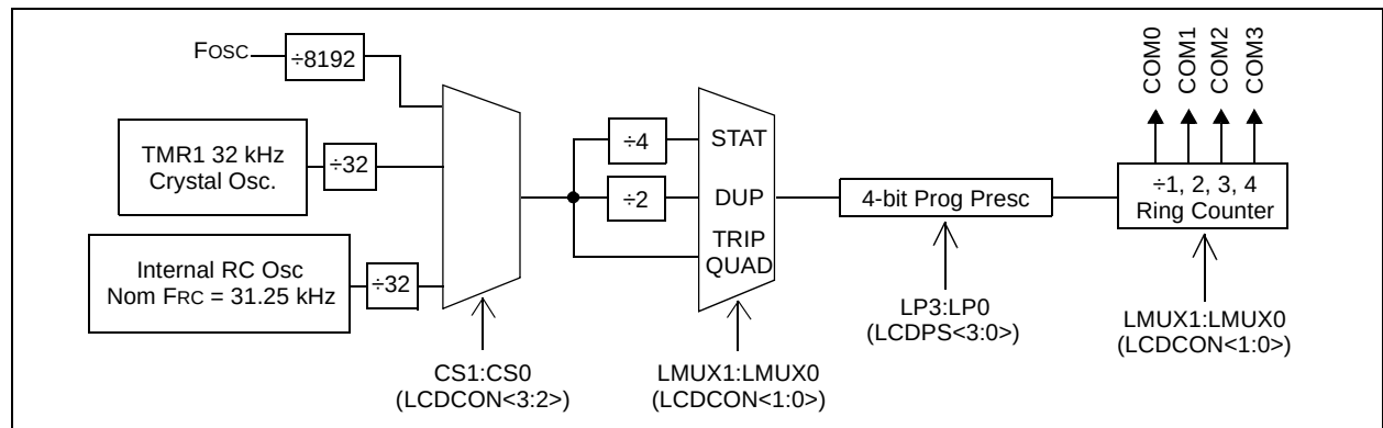
FIGURE 22-3: LCD CLOCK GENERATION
