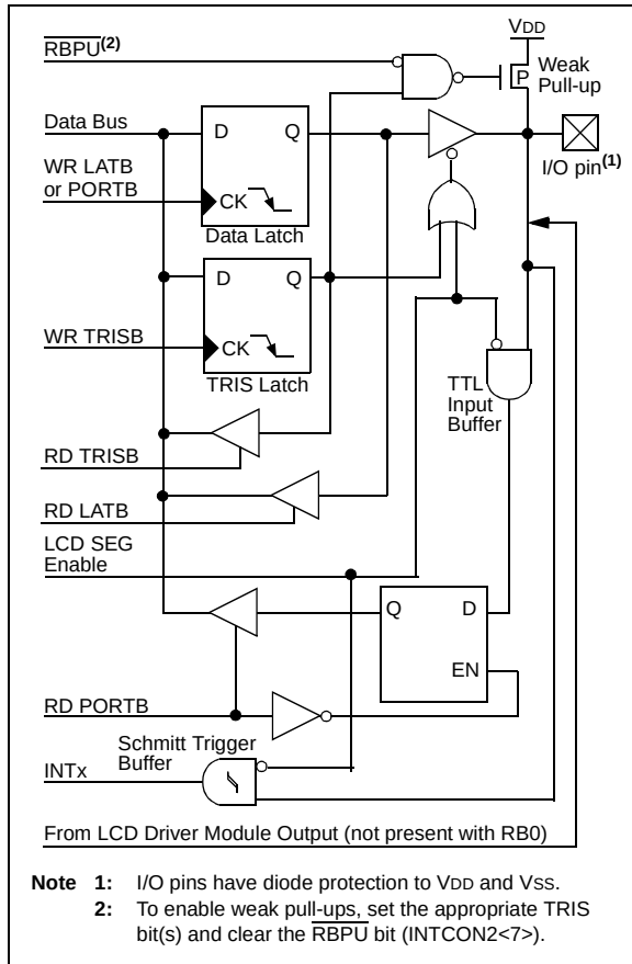
FIGURE 9-7: BLOCK DIAGRAM OF RB3:RB0 PINS
