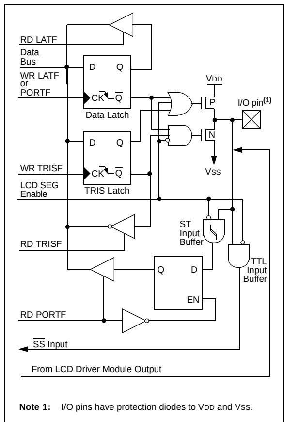
FIGURE 9-15: BLOCK DIAGRAM OF RF7 PIN
