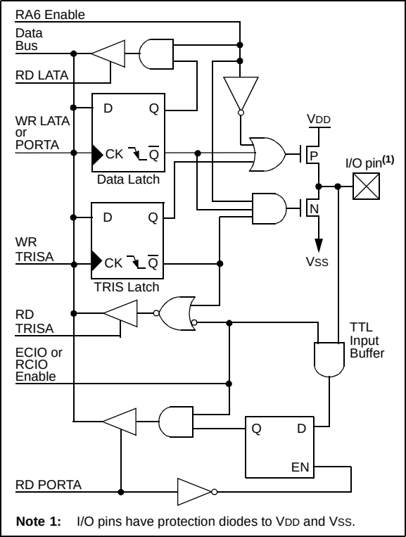
FIGURE 9-3: BLOCK DIAGRAM OF RA6 PIN
