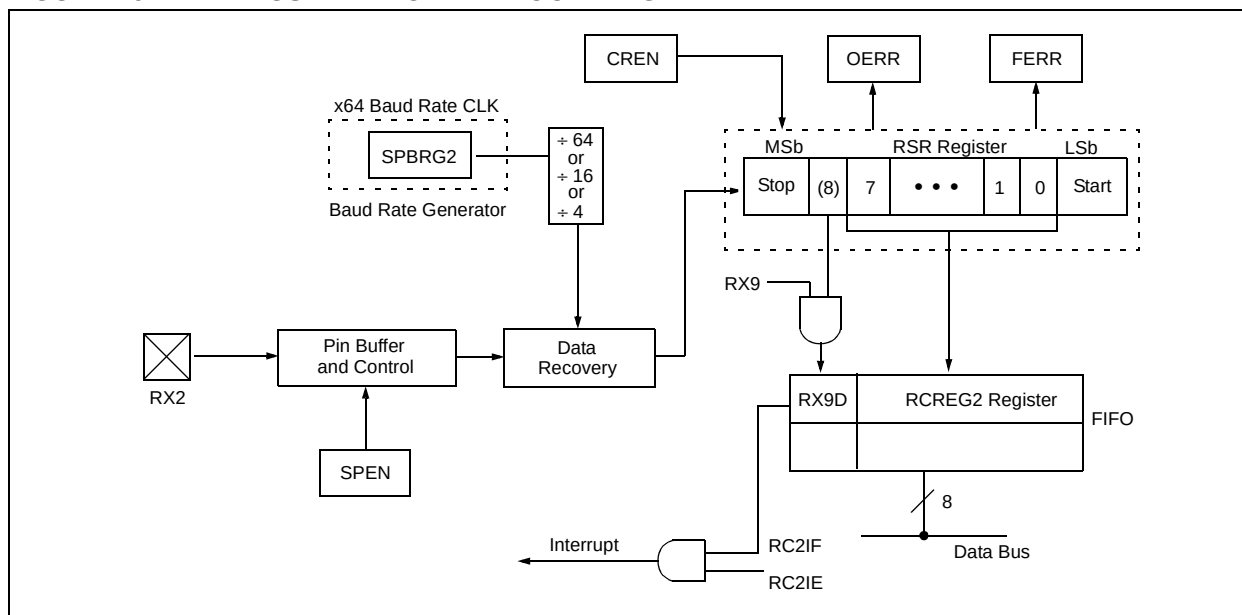
FIGURE 16-4: AUSART RECEIVE BLOCK DIAGRAM
