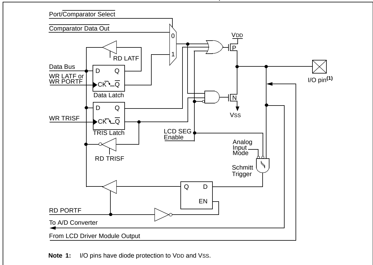
FIGURE 9-13: BLOCK DIAGRAM OF RF1/AN6/C2OUT, RF2/AN7/C1OUT PINS
