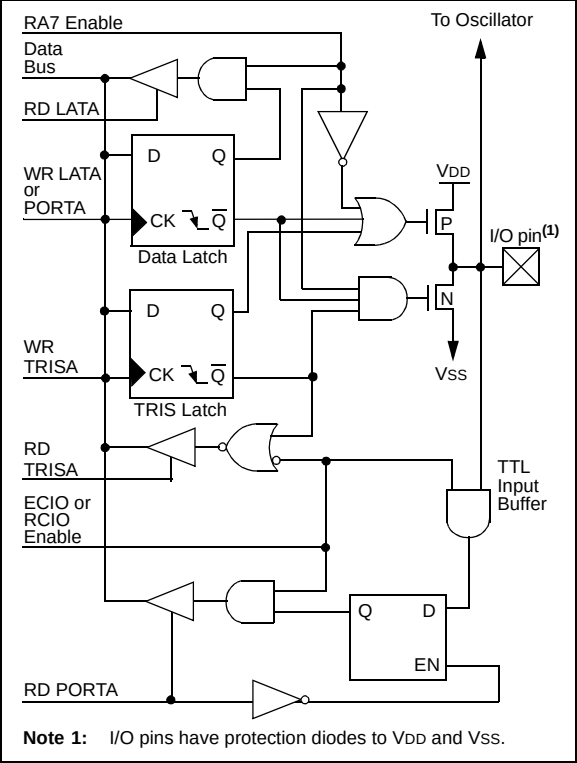
FIGURE 9-5: BLOCK DIAGRAM OF RA7 PIN
