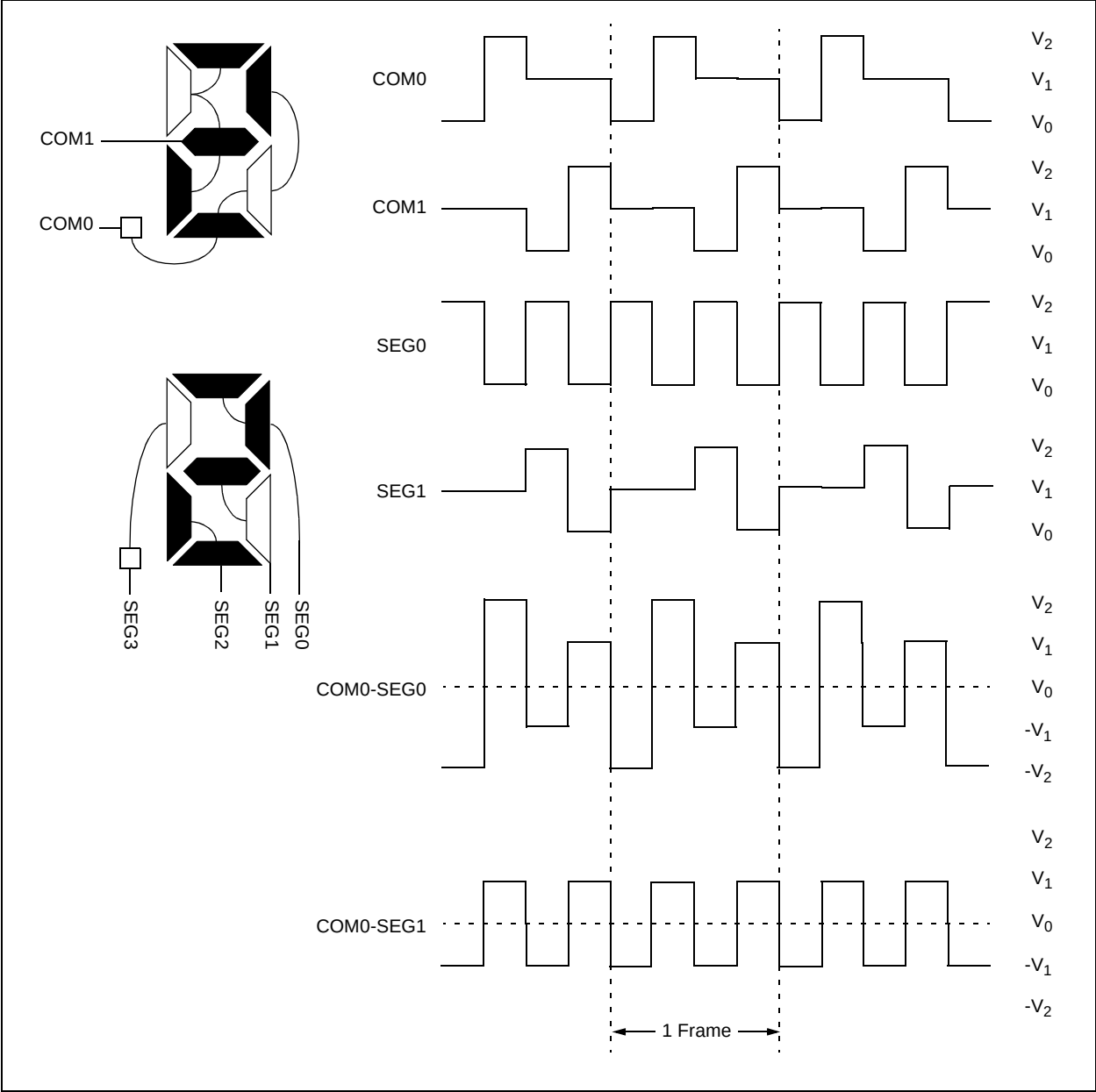
FIGURE 22-5: TYPE-A WAVEFORMS IN 1/2 MUX, 1/2 BIAS DRIVE
