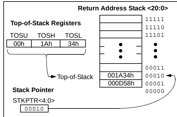
FIGURE 5-2: RETURN ADDRESS STACK AND ASSOCIATED REGISTERS
