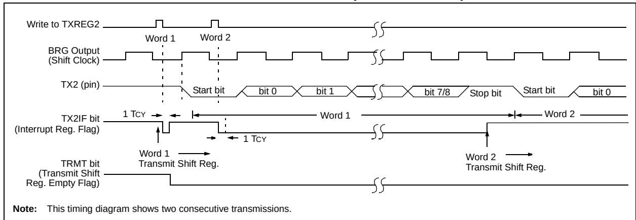
FIGURE 16-3: ASYNCHRONOUS TRANSMISSION (BACK TO BACK)
