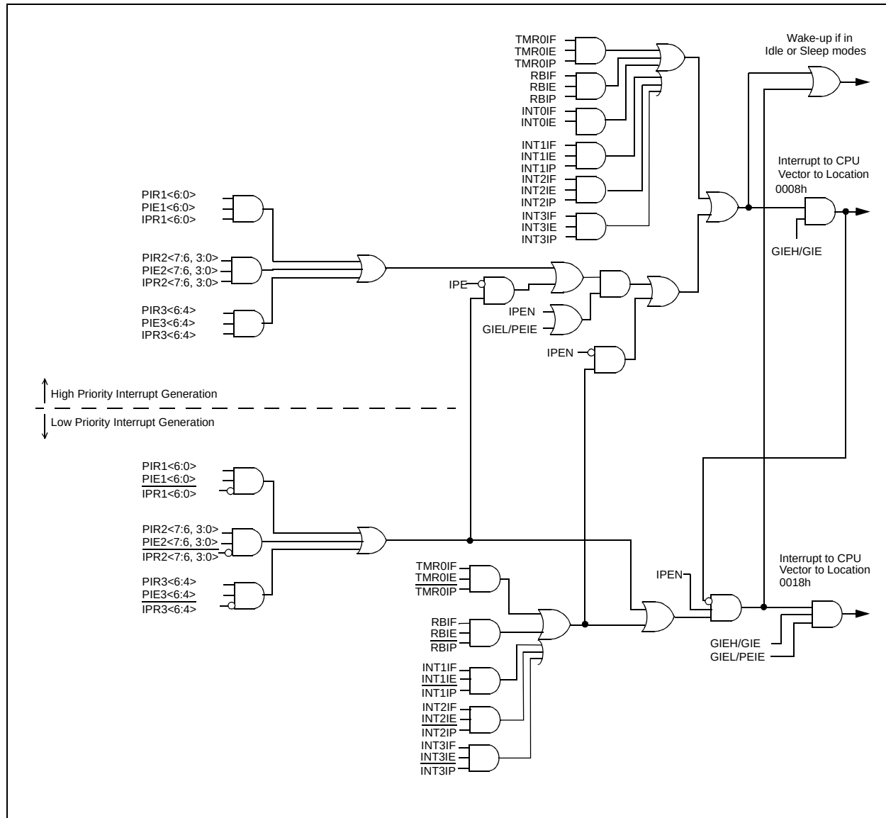
FIGURE 8-1: PIC18F6490/8490 INTERRUPT LOGIC
