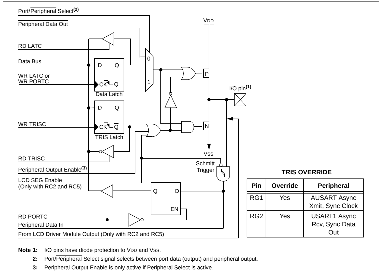
FIGURE 9-16: PORTG BLOCK DIAGRAM (PERIPHERAL OUTPUT OVERRIDE)
