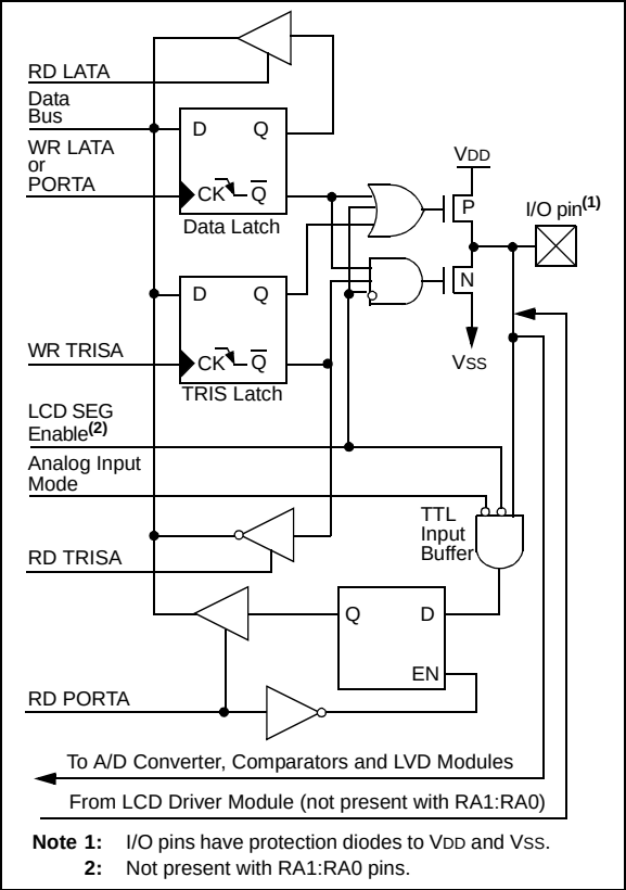
FIGURE 9-2: BLOCK DIAGRAM OF RA3:RA0 AND RA5 PINS
