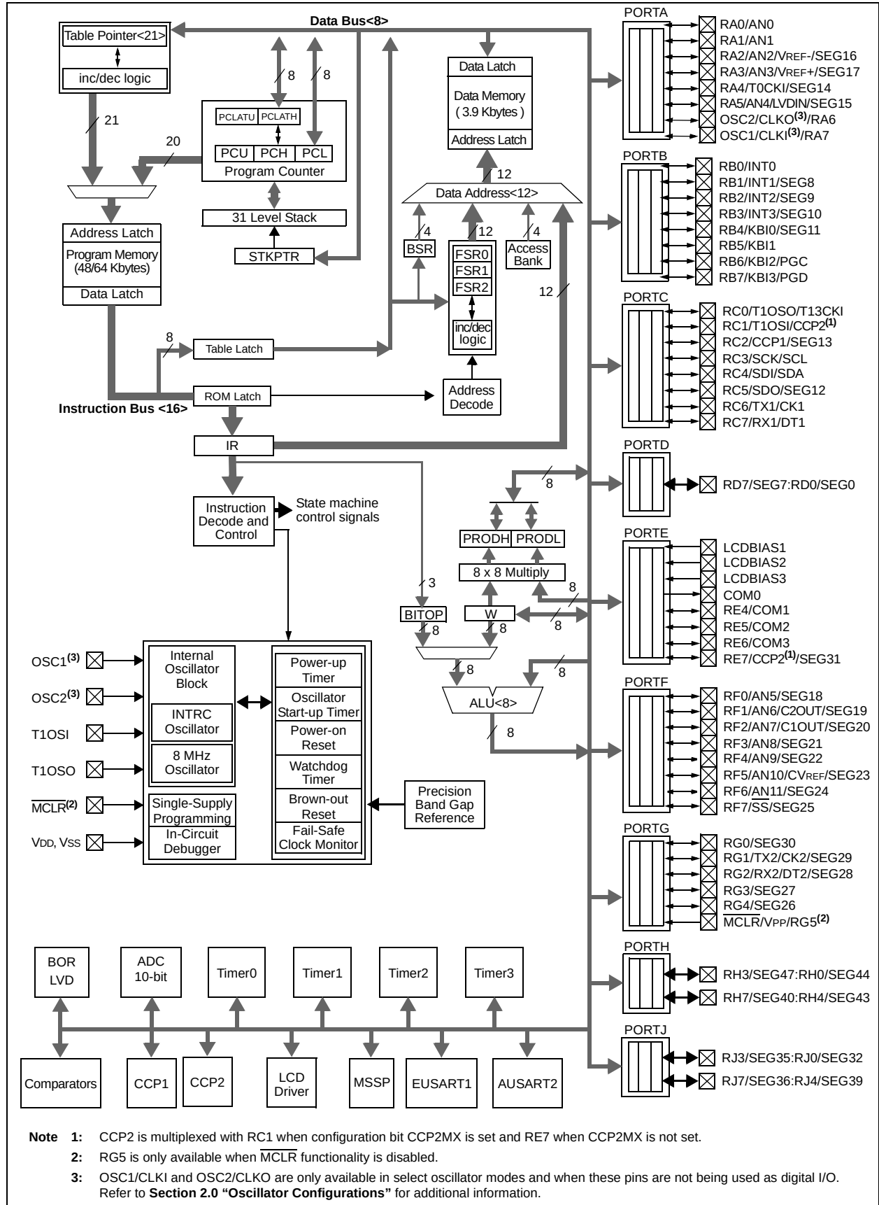
FIGURE 1-2: PIC18F8490 (80-PIN) BLOCK DIAGRAM
