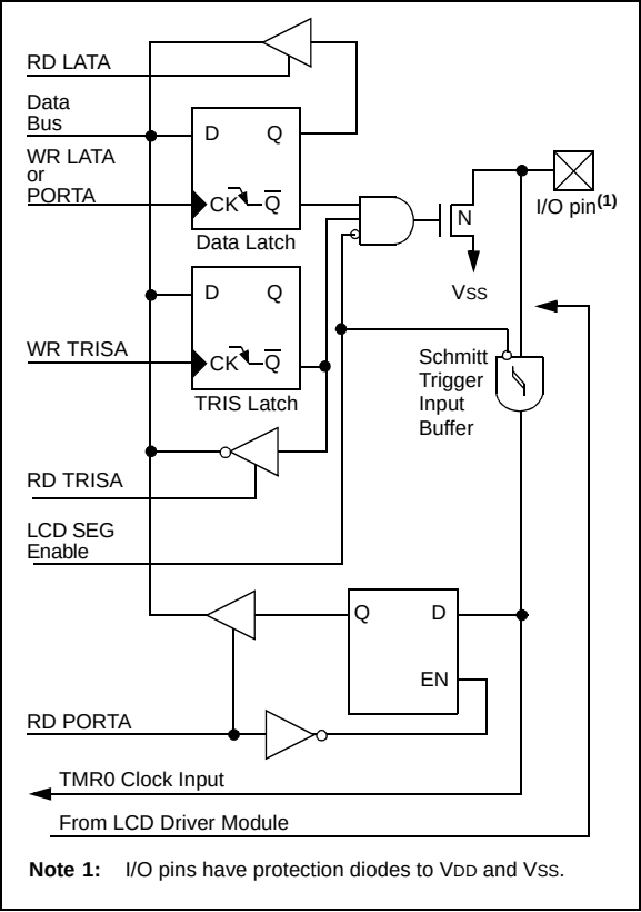
FIGURE 9-4: BLOCK DIAGRAM OF RA4/T0CKI PIN
