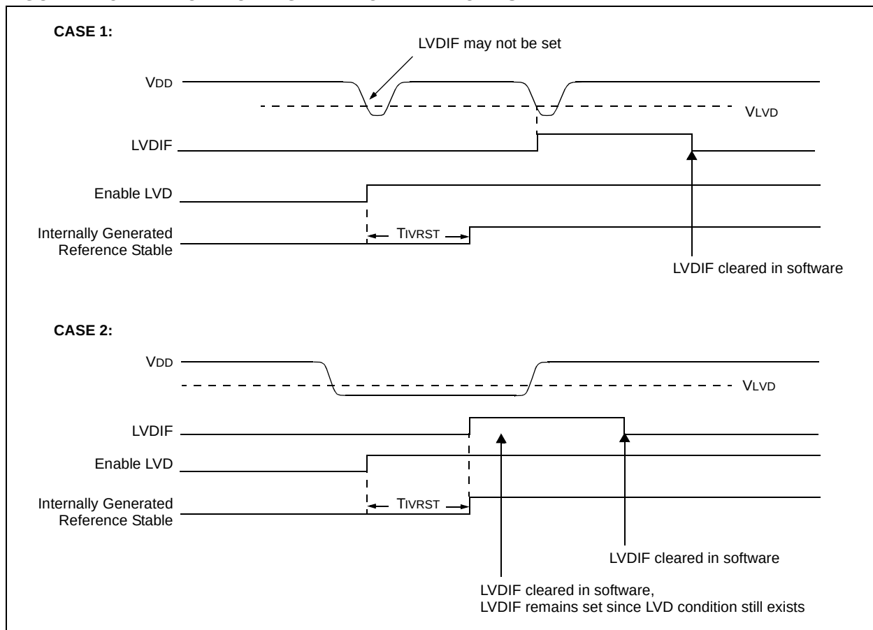
FIGURE 21-3: LOW-VOLTAGE DETECT WAVEFORMS
