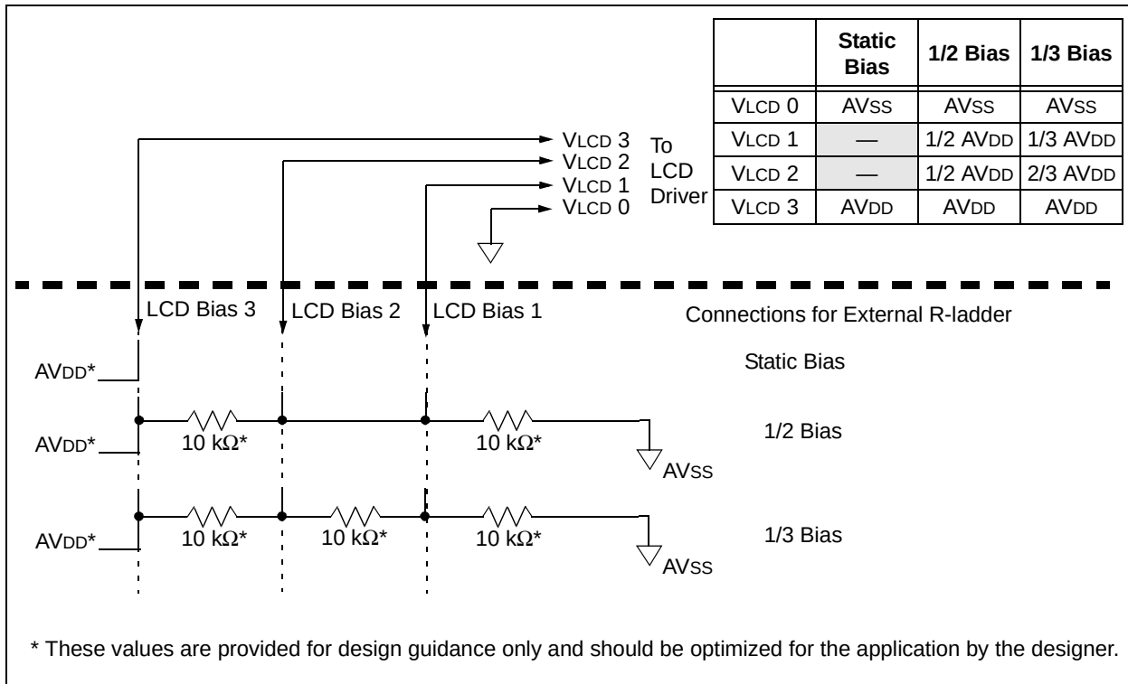
FIGURE 22-2: LCD BIAS RESISTOR LADDER CONNECTION DIAGRAM
