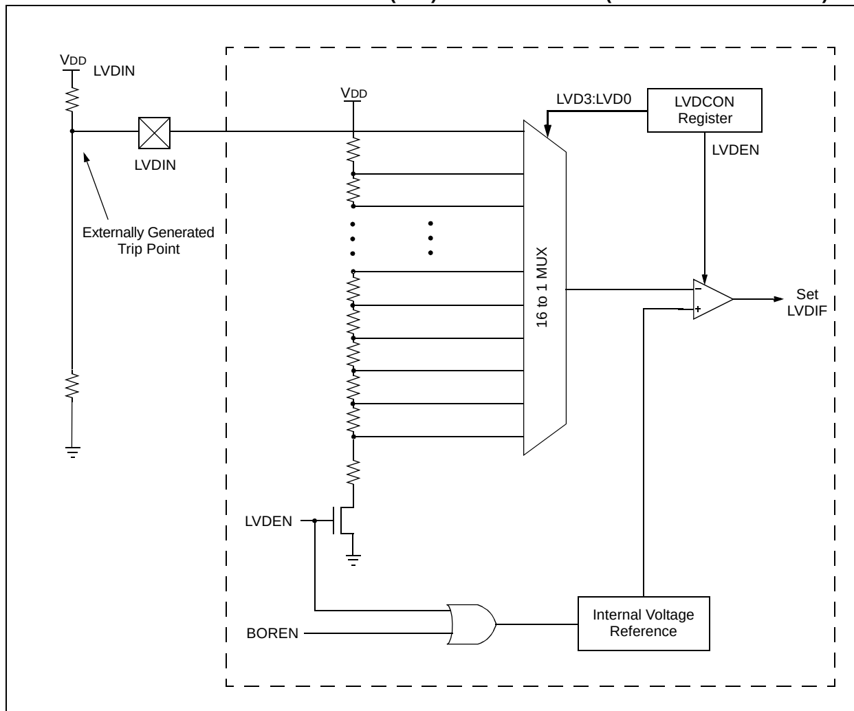
FIGURE 21-2: LOW-VOLTAGE DETECT (LVD) BLOCK DIAGRAM (WITH EXTERNAL INPUT)
