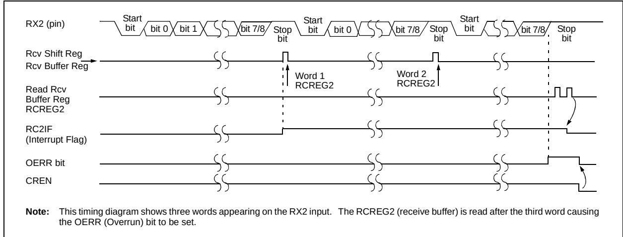
FIGURE 16-5: ASYNCHRONOUS RECEPTION
