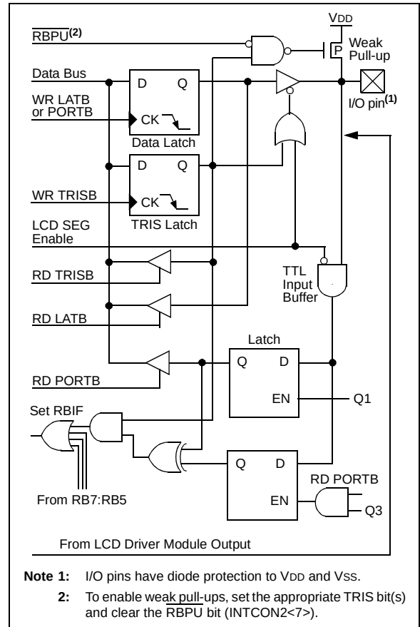
FIGURE 9-8: BLOCK DIAGRAM OF RB4 PIN
