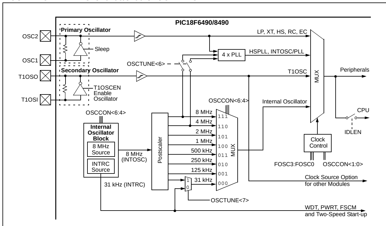
FIGURE 2-8: PIC18F6490/8490 CLOCK DIAGRAM
