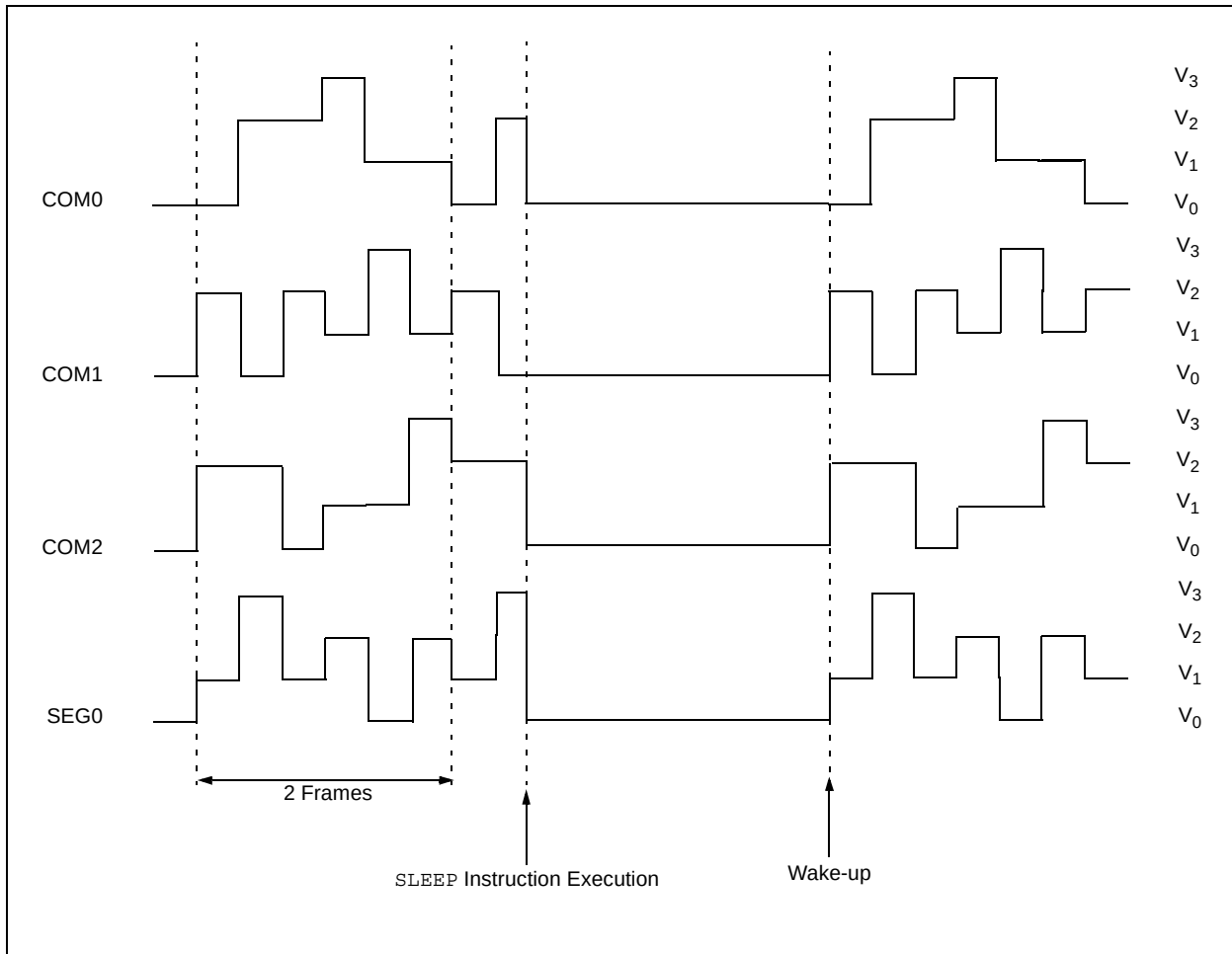
FIGURE 22-16: SLEEP ENTRY/EXIT WHEN SLPEN = 1 OR CS1:CS0 = 00
