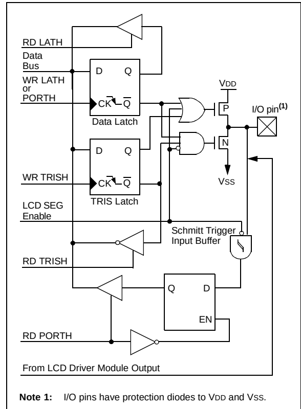
FIGURE 9-18: BLOCK DIAGRAM OF RH7:RH0 PINS
