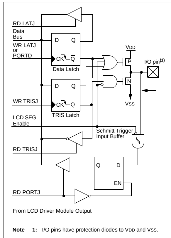
FIGURE 9-19: BLOCK DIAGRAM OF RJ7:RJ0 PINS
