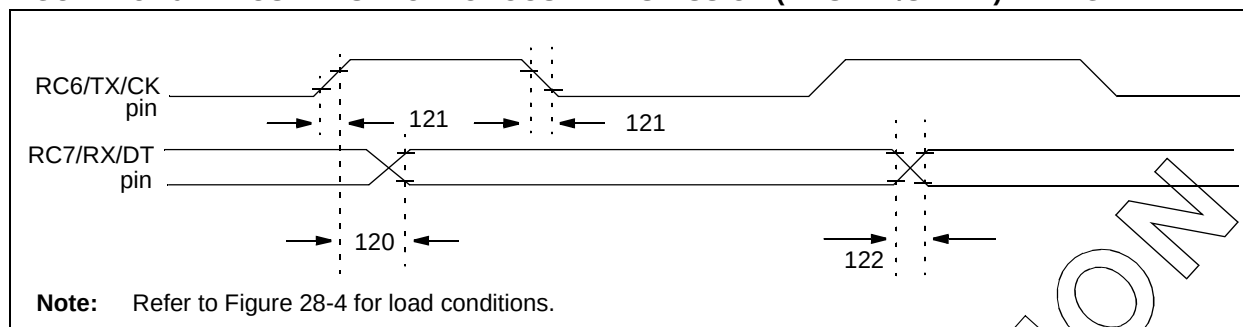
FIGURE 28-19: USART SYNCHRONOUS TRANSMISSION (MASTER/SLAVE) TIMING
