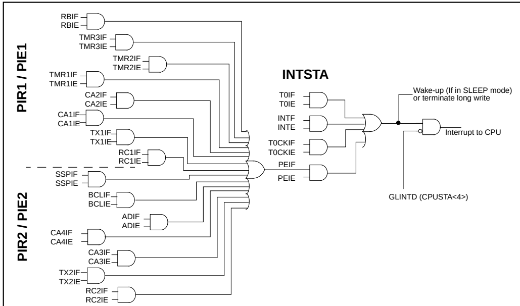
FIGURE 6-1: INTERRUPT LOGIC
