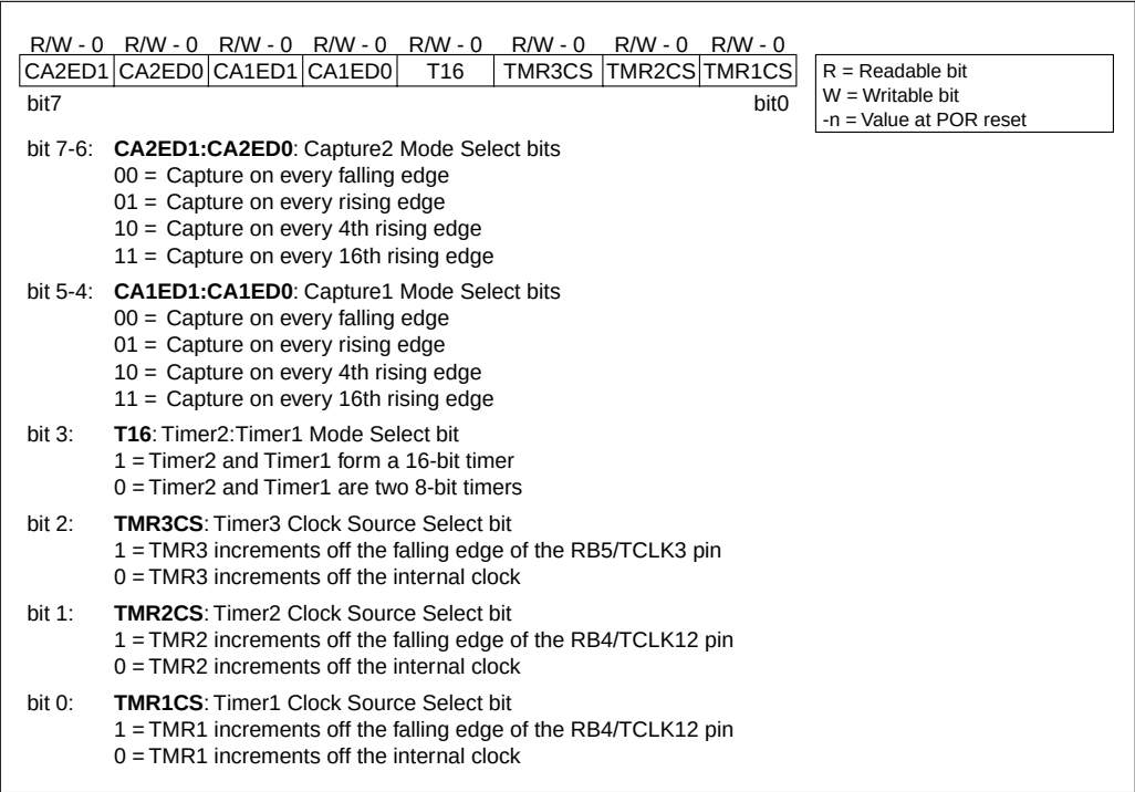
FIGURE F-12: TCON1 REGISTER (ADDRESS: 16h, BANK 3)
