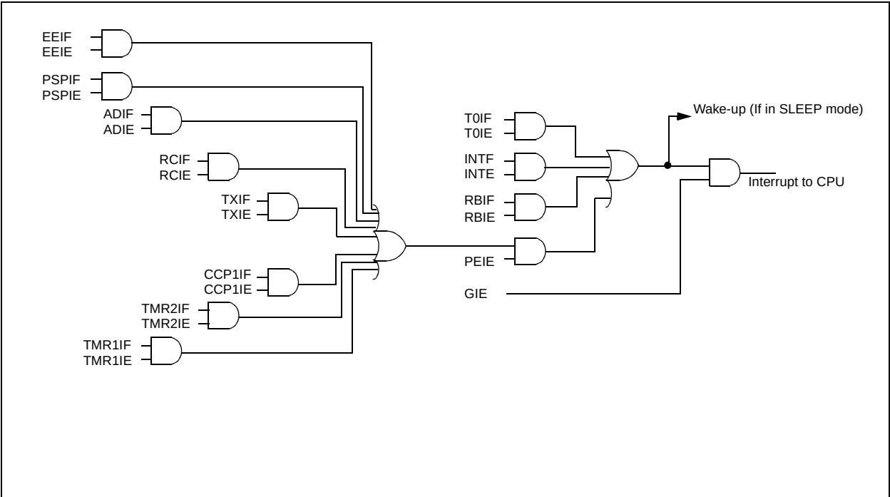
FIGURE 11-9: INTERRUPT LOGIC
