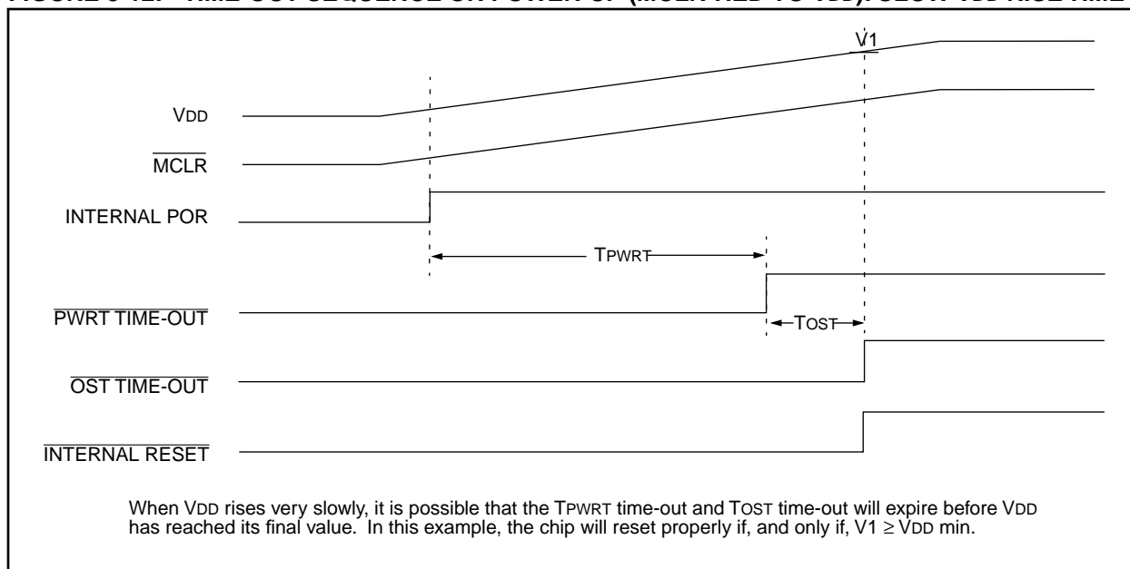
FIGURE 8-12: TIME-OUT SEQUENCE ON POWER-UP ( \overline{\text{MCLR}} TIED TO V_{DD} ): SLOW V_{DD} RISE TIME
