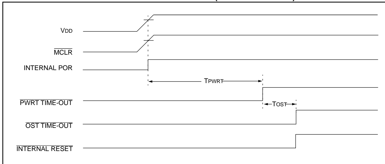
FIGURE 8-12: TIME-OUT SEQUENCE ON POWER-UP ( \overline{\text{MCLR}} TIED TO V_{DD} ): SLOW V_{DD} RISE TIME
