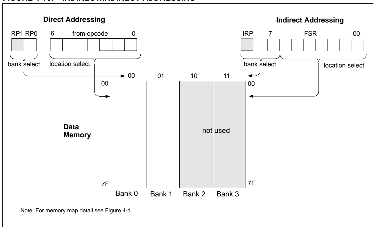
FIGURE 4-10: INDIRECT/INDIRECT ADDRESSING
