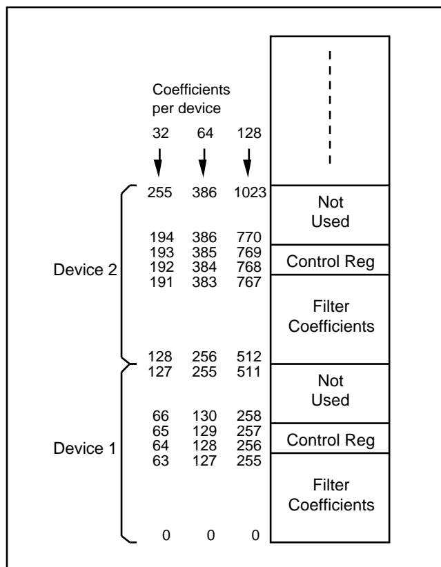
Fig. 16 EPROM Memory Map
