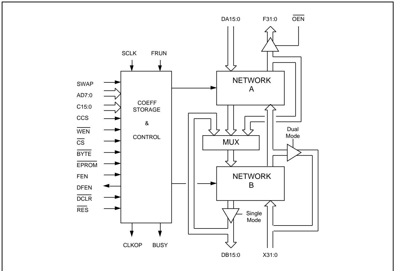
Fig. 4 Block Diagram
