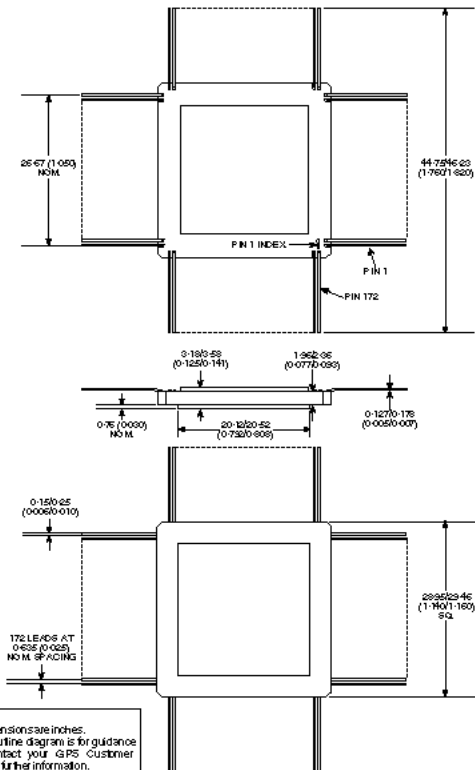
172-LEAD CERAMIC POWER FLATPACK - GC172 (POWER)
