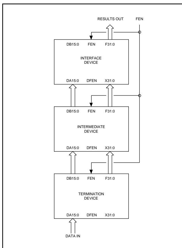
Fig. 13 Full Speed Cascaded System
