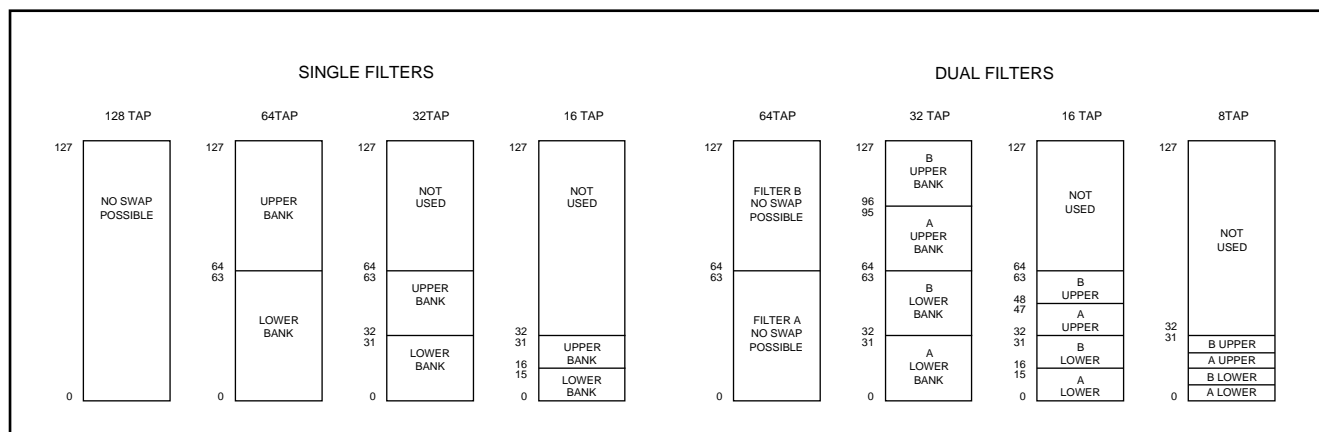
Fig. 14 Coefficient Memory Map
