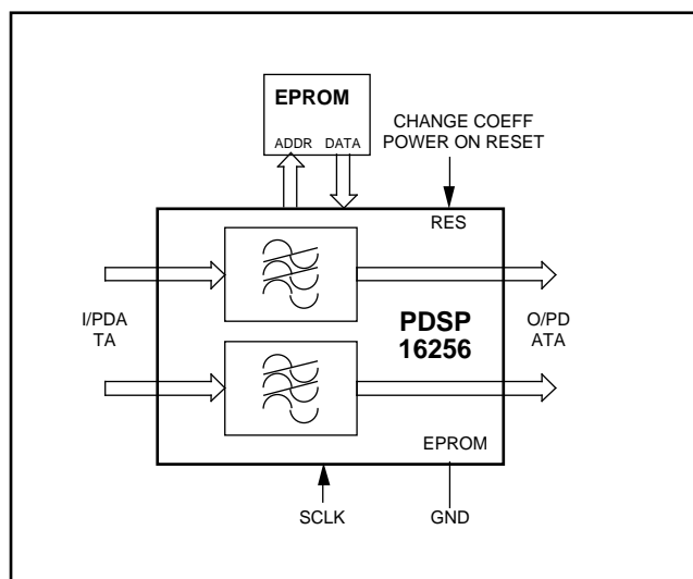
Fig. 1 Dual Filter
