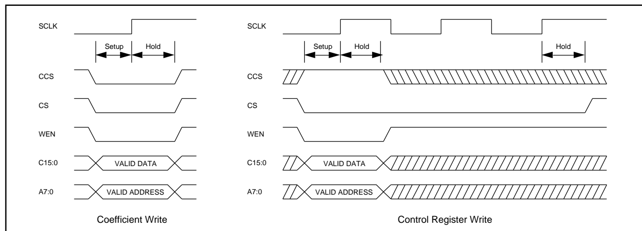
Fig. 17 Remote Master Setup & Hold Timings
