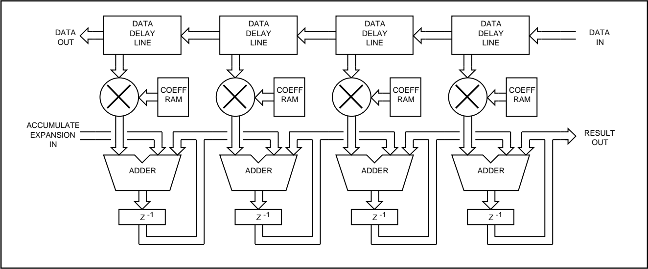
Fig. 5 Filter Network Diagram
