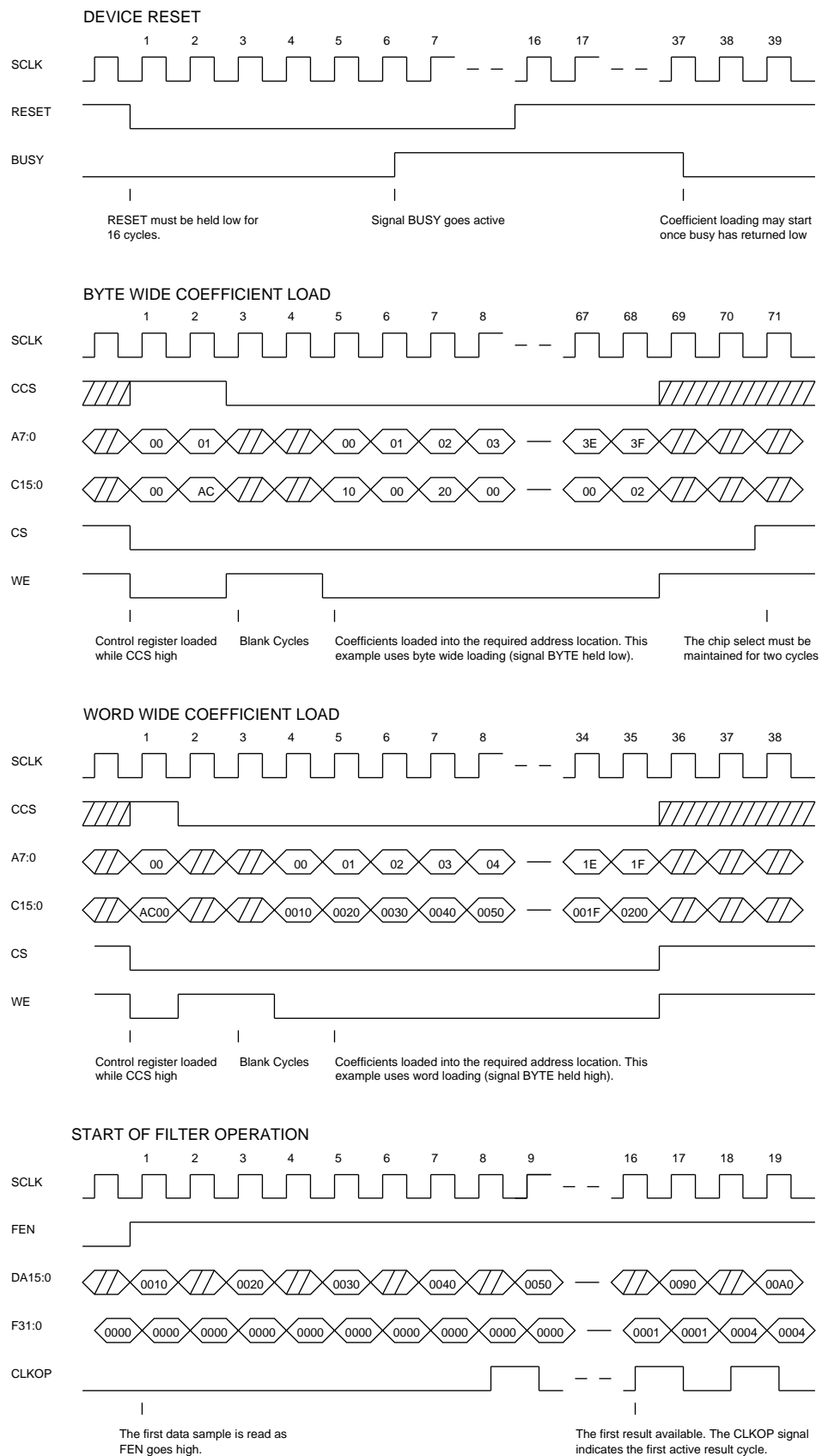
Fig. 19 Device Startup
