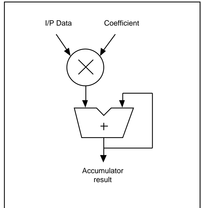
Fig. 10 Multiplier Accumulator
