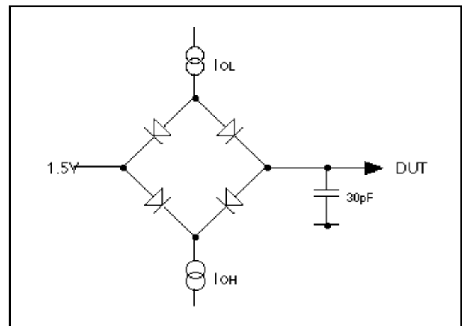
Fig. 20 Three state delay measurement load.
