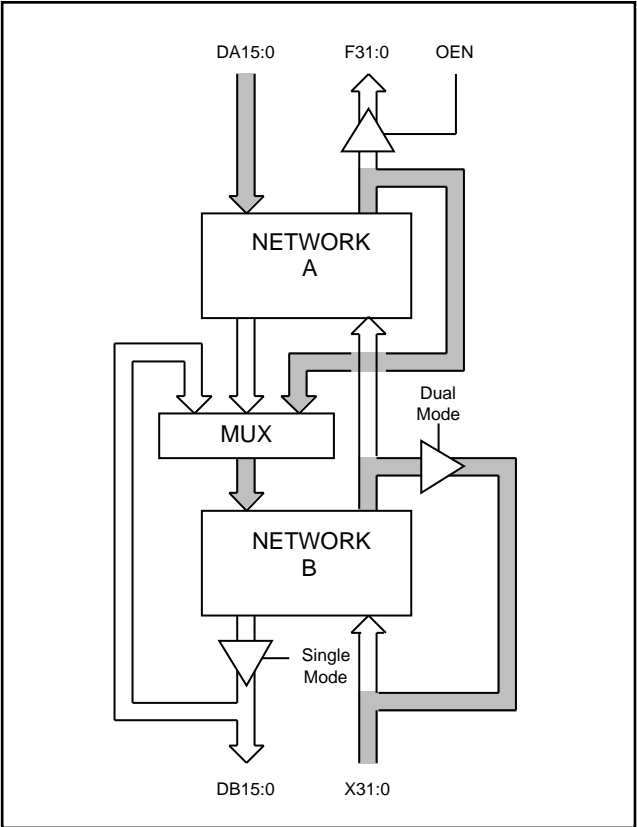
Fig. 9 Dual Cascaded Filter Bus Utilisation
