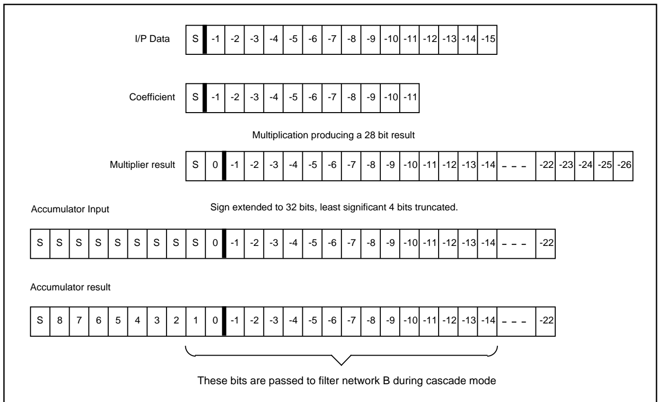
Fig. 11 Filter Accuracy
