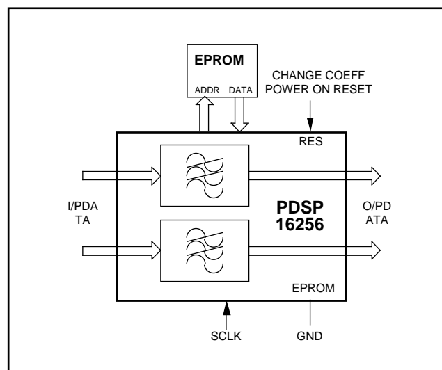
Fig. 2 Typical System Application
