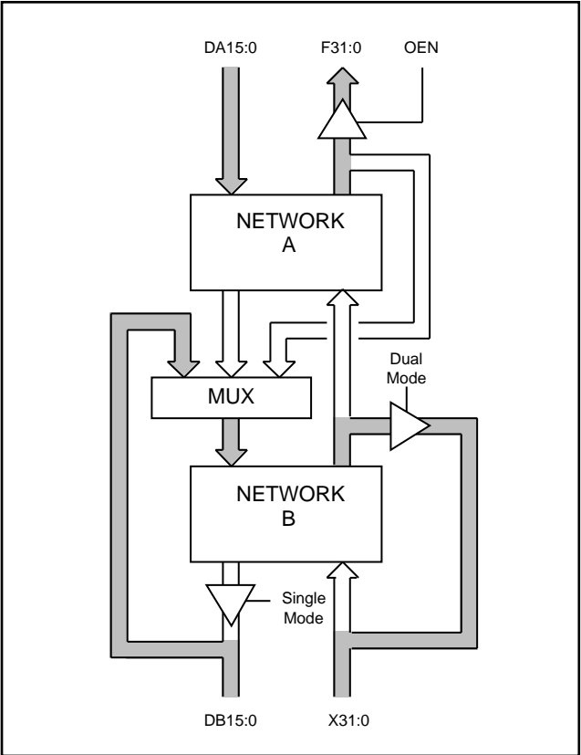
Fig. 8 Dual Independent Filter Bus Utilisation
