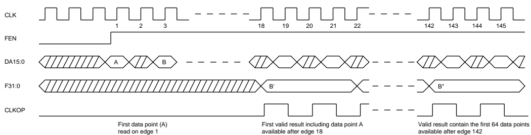
Fig. 7 Single Filter Timing Diagrams
