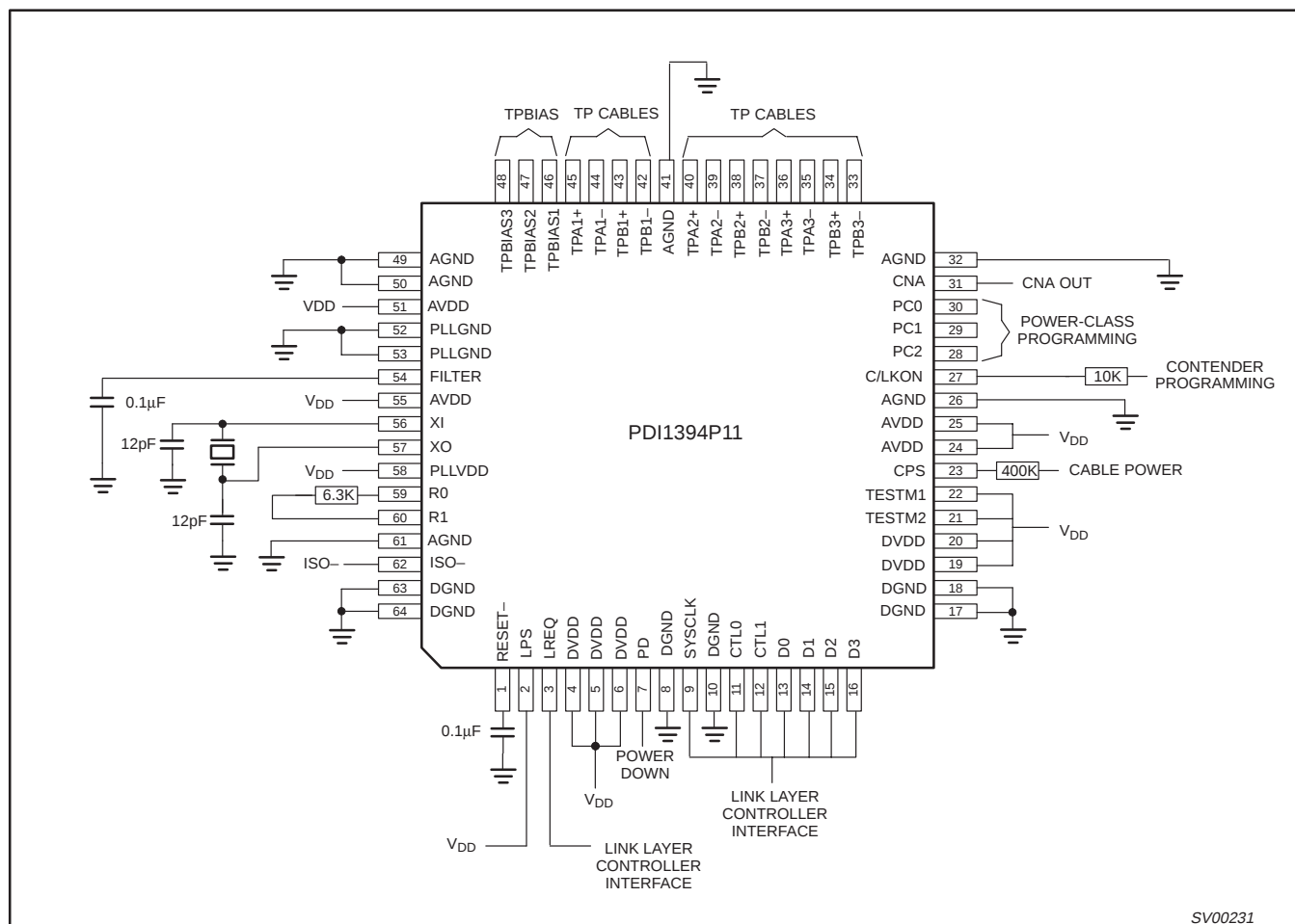
Figure 3. External Component Connections
