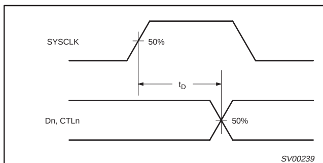
Figure 2. Dn, CTLn, output delay relative to SYSCLK
