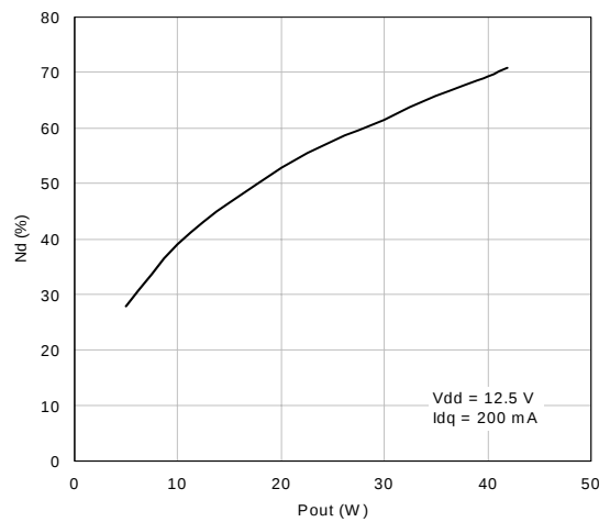
Drain Efficiency vs Output Power ( f = 175\text{ MHz} )
