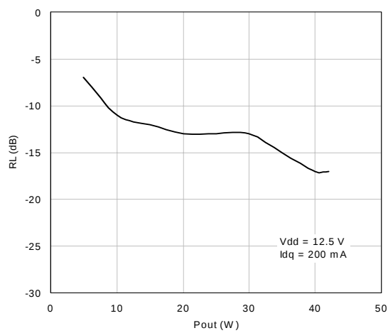
Input Return Loss vs Output Power ( f = 175\text{ MHz} )
