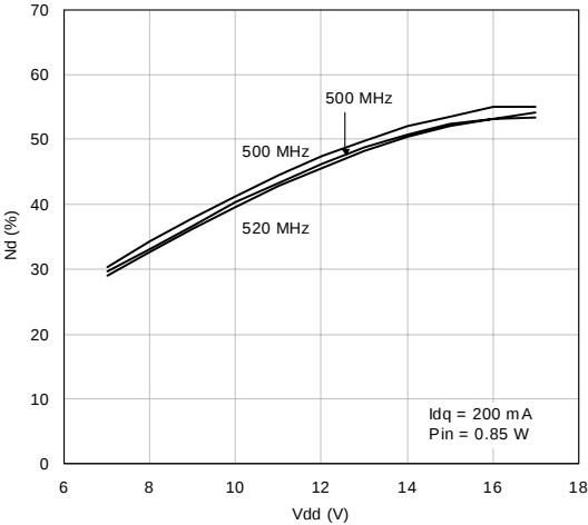
Drain Efficiency vs Supply Voltage
