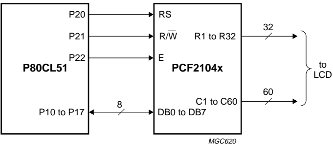
Fig.27 Direct connection to 8-bit microcontroller; 8-bit bus.
