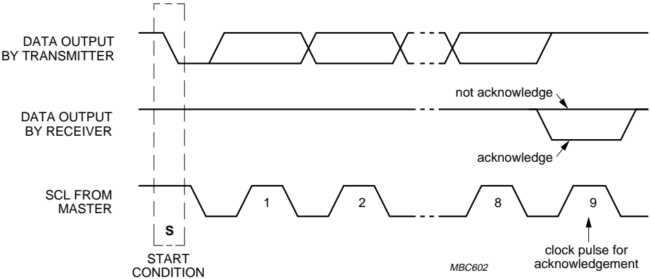
Fig.20 Acknowledgement on the I 2 C-bus.
