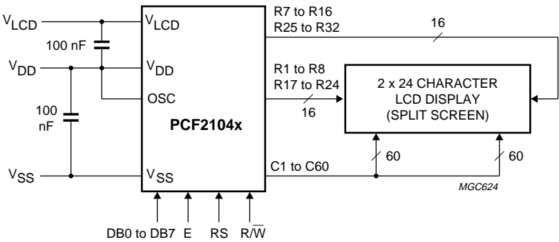
Fig.29 Typical application using parallel interface.
