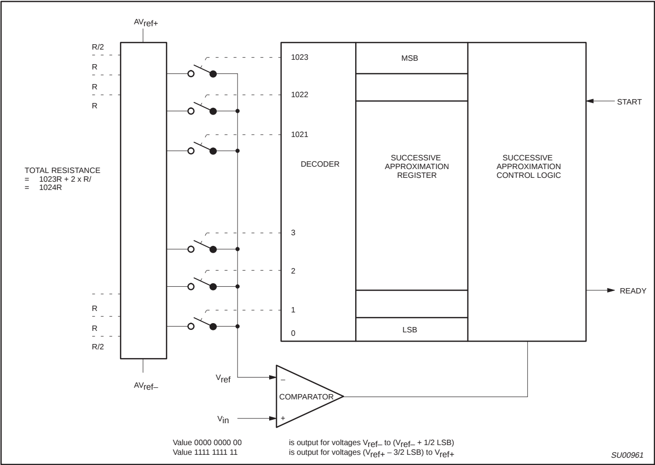
Figure 23. ADC Realization
