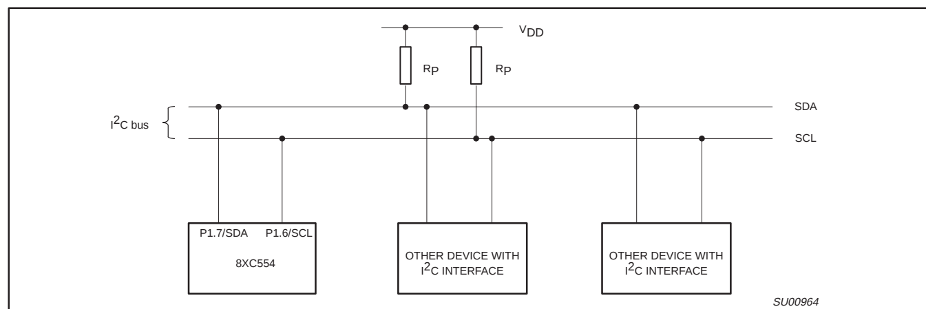
Figure 32. Typical I 2 C Bus Configuration
