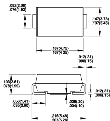
DO-214AA (SMB)
