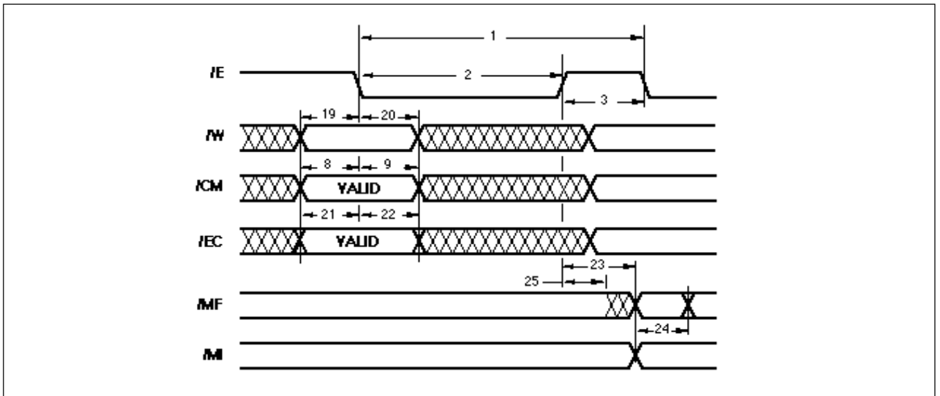
Fig.12 P1480 match flag response
