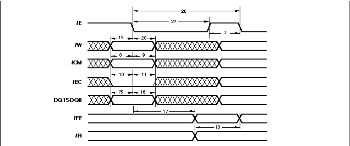
Fig.11 P1480 write cycle
