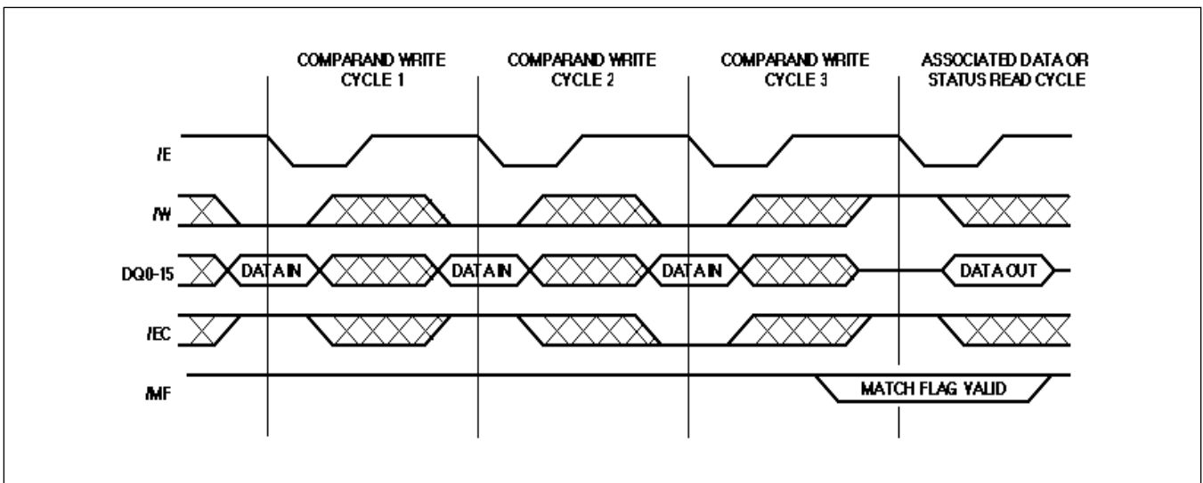
Fig.6 - Cycle-to-cycle timing
