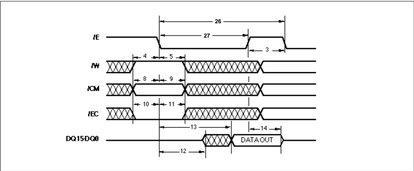
Fig.10 P1480 read cycle
