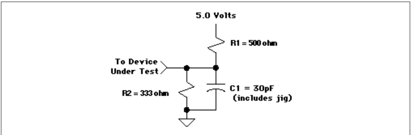
Fig.7 - AC test load
