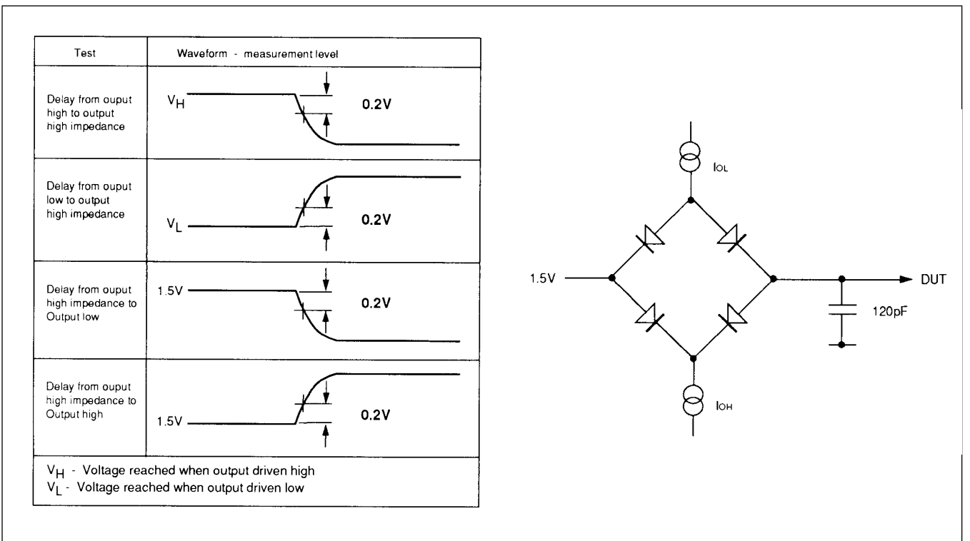
Fig.8 - Three state delay measurement
