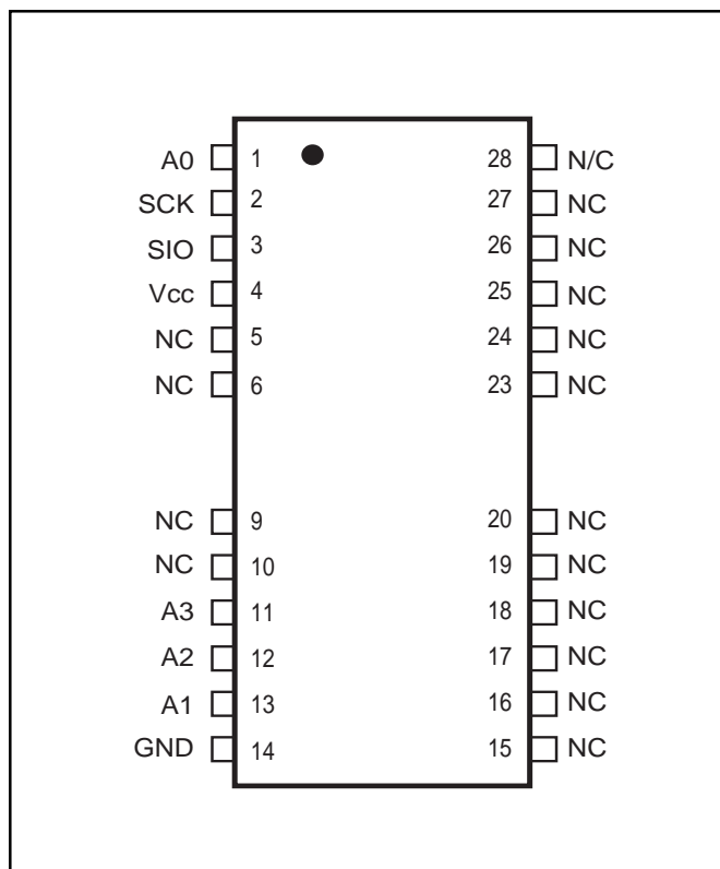
Figure 1. NX26F080A and NX26F160 Pin Assignments
