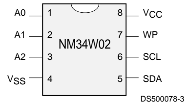
TSSOP Package (MT8)
