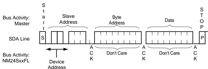
WP Register Write (Figure 7).
