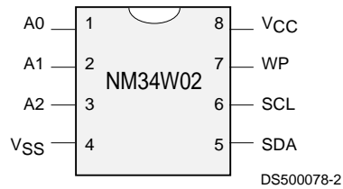
SO Package (M8)
