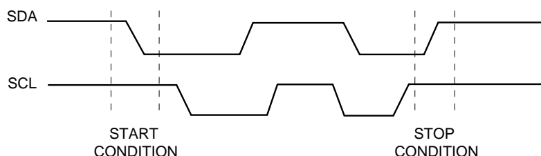
Start and Stop Definition (Figure 2).
