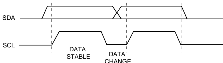
Data Validity (Figure 1).
