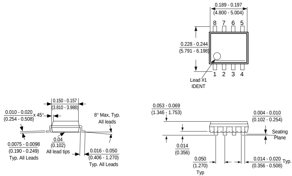
Molded Small Out-Line Package (M8) Order Number NM24C65xxxM8 or NM24C65xxxEM8 Package Number M08A
