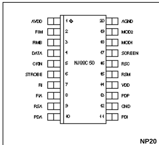
Fig.1 Pin assignment
