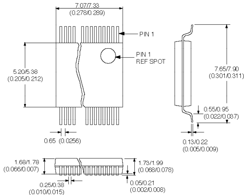
20 - LEAD SHRUNK MINIATURE PLASTIC DIL - NP20
